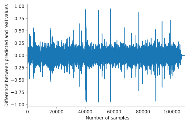
Figure 7.6: MLP difference between predicted and actual values for one interface.
