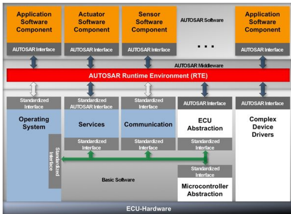
FIGURE 2.9 – Architecture Logicielle
