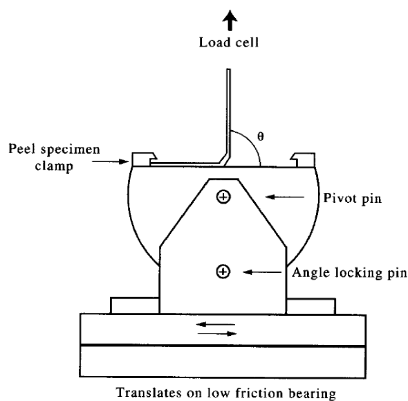
Figure I.4.8: Peel testing rig [57].
