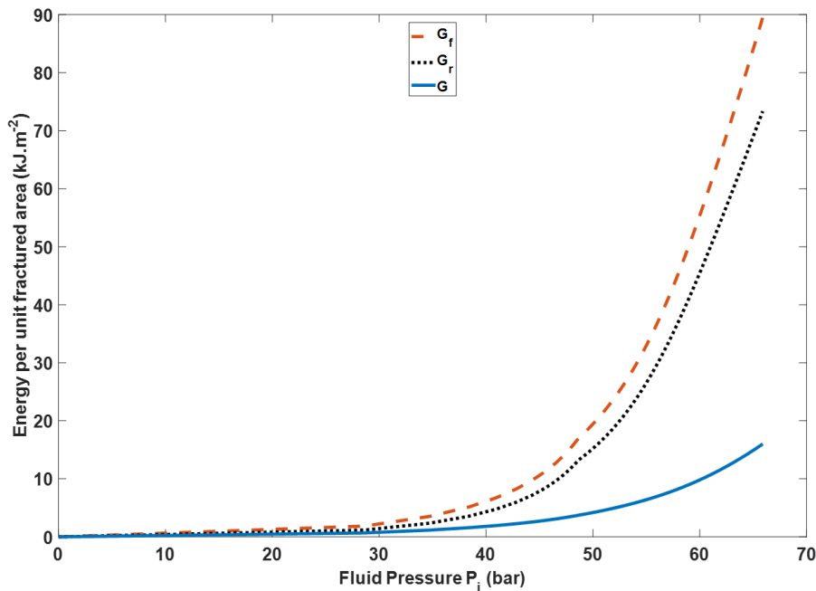
Figure II.3.4: Comparison of the energies stored in the fluid and the rubber at crack propagation, calculated for a unit fractured area. G_r is the contribution of the rubber envelope and G_f is of the fluid. G is the SERR, plotted using (II.3.11).
