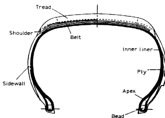
Figure I.2.1: Cross-section of a tyre [4].
