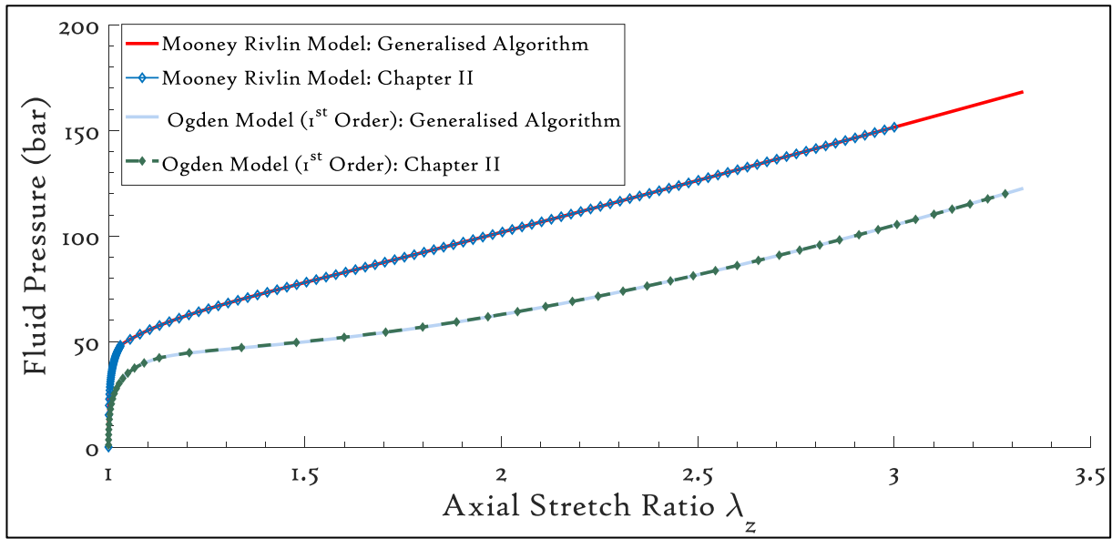
Figure IV.2.3: Comparison between Thick-Walled Cylinder Inflation algorithms presented in Figure IV.2.2 and Chapter II.
