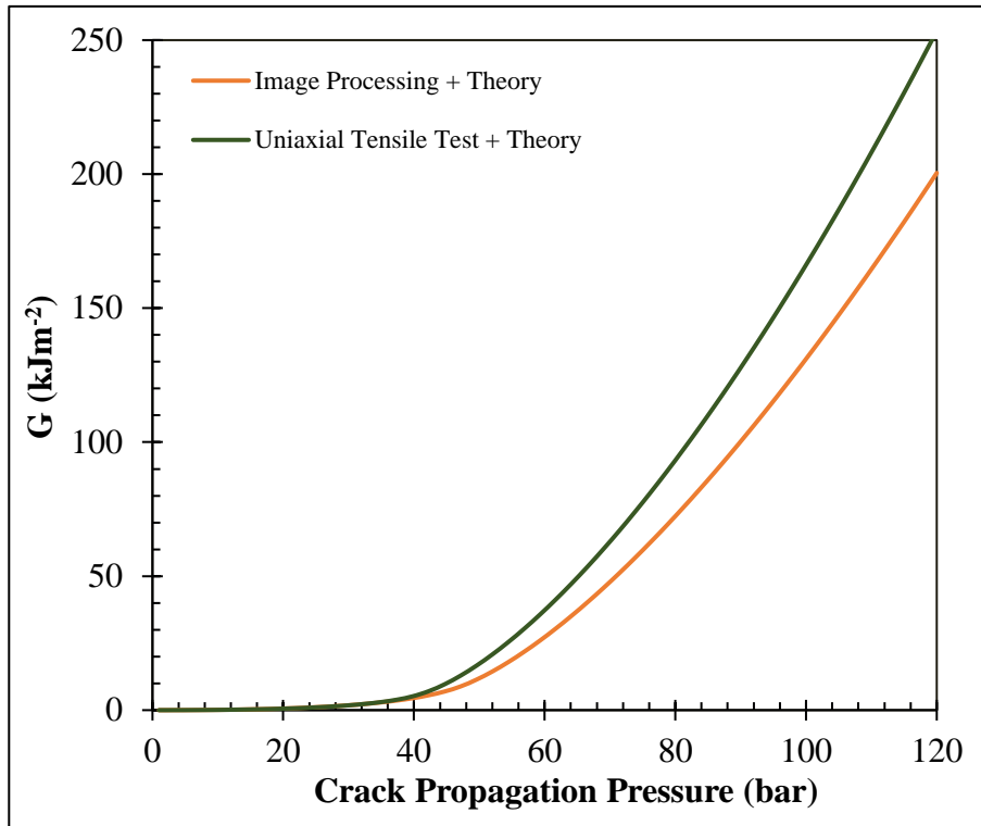
Figure III.3.8: Effect of rubber model parameters on SERR calculation.
