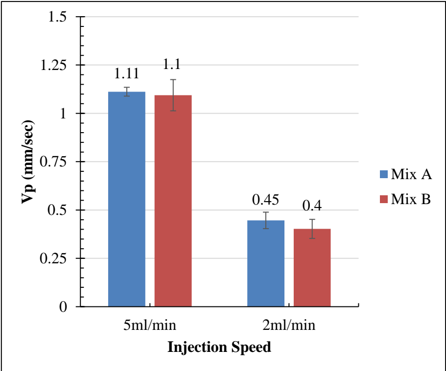
Figure III.4.8: Average crack propagation speeds for the 20 tests.
