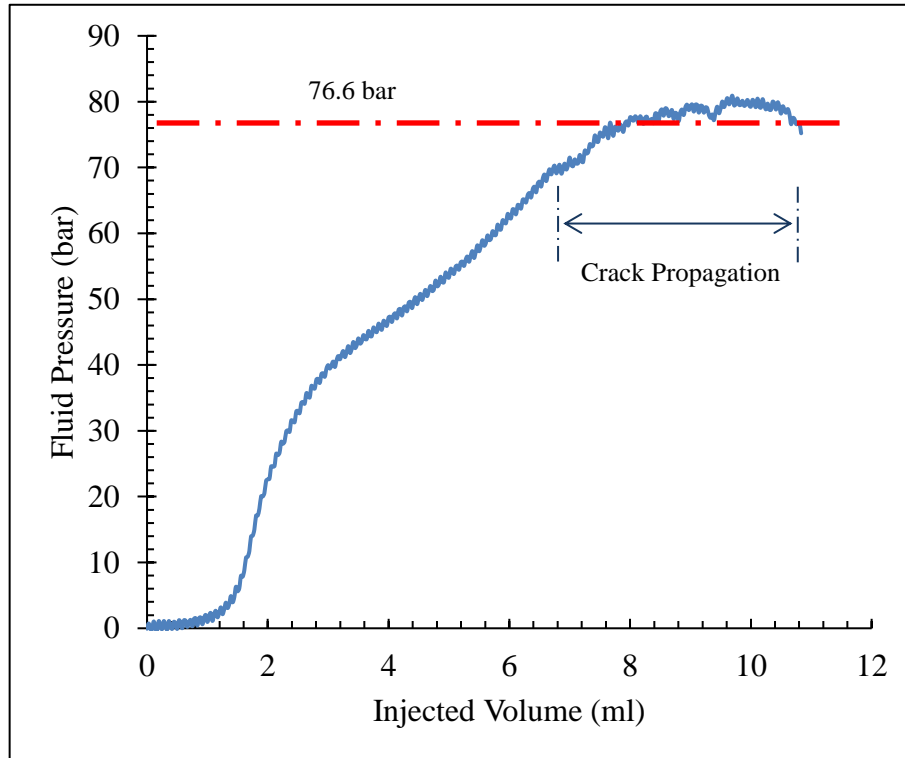
Figure III.3.1: A typical fluid pressure versus injected fluid volume evolution during RCAIT.
