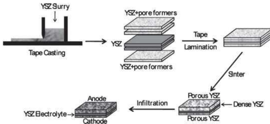
Figure 1.19. Diagram showing the steps used to fabricate an SOFC in which the electrodes are produced by infiltration of active components into a porous YSZ scaffold[40].
