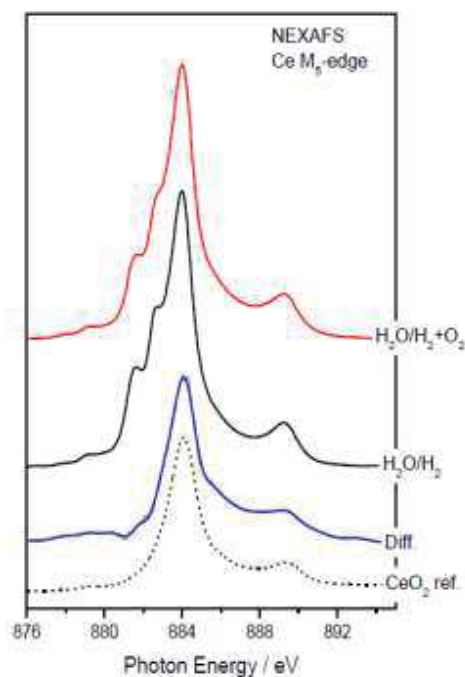
Figure 3.7. Ce M 5 -edge NEXAFS spectra measured on the Ni-GDC electrode in 0.5 mbar H 2 O/H 2 at 640 °C and at a current of -100 mA/cm 2 before and during co-feed of O 2 . The
