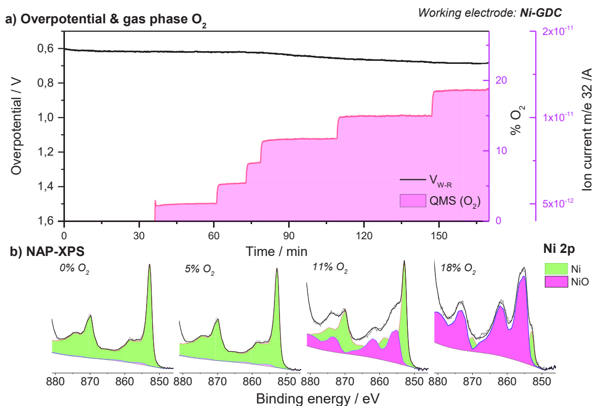
Figure 3.2. a) Time evolution of the Ni-GDC cathode overpotential ( black line ) and the on line mass spectrometer signal of oxygen ( pink line ) measured at constant current of -100 \text{ mA/cm}^2 while different concentrations of O_2 were introduced in the H_2O/H_2 feed. The temperature was kept constant at 640^\circ\text{C} . b) Ni 2p NAP-XPS spectra recorded during characteristic moments of
