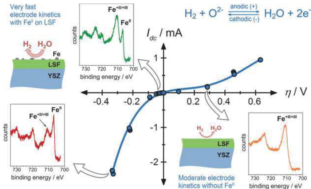
Figure 1.29. Current–overpotential curve ( I_{dc} vs.) of LSF in a humid reducing atmosphere (0.25 mbar \text{H}_2 +0.25 mbar \text{H}_2\text{O} ). The reaction proceeding on the surface of the LSF working electrode is given on the top right. For selected points of the curve (indicated by arrows), the Fe2p XPS spectra are shown as insets. The sketches indicate the situation for the LSF surface and the resulting reactivity, respectively[47].
