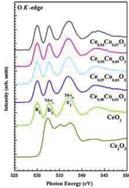
Figure 1.26. O K-edge spectra of \text{Ce}_{1-x}\text{Co}_x\text{O}_2 ( 0 \leq X \leq 0.07 ) nanoparticles along with reference spectrum of \text{Ce}_2\text{O}_3 [45].
