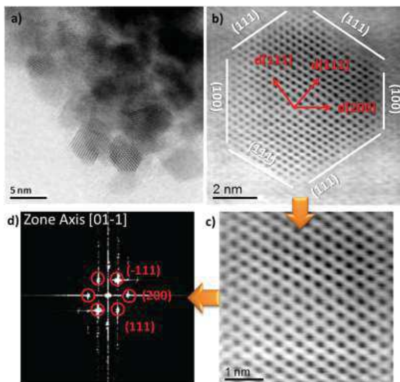
Figure. 4.6. High resolution bright field STEM image and the corresponding FFT diffraction pattern of \text{Ni}_{0.1}\text{Ce}_{0.9}\text{O}_{2-x} formed after calcination at 400 °C.
