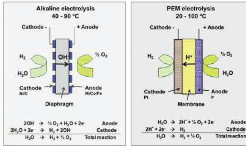
Figure 1.2: Schematic of the operating principle of the low temperature electrolysis technology (alkaline and PEM water electrolysis cell), taken from[29].
