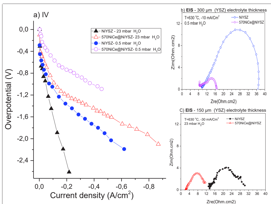
Figure 5.5. a) Current-overpotential curves measured under steam electrolysis conditions over Ni-YSZ and 570NiCe@NiYSZ electrodes during stem electrolysis at 630^\circ\text{C} in 0.5 mbar and 23 mbar of 100% \text{H}_2\text{O} . Impedance spectra presented in Nyquist form, b) obtained under constant
