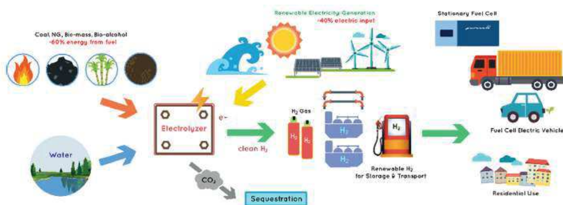
Figure 1.8. Hydrogen production by electrolysis and its applications[33].
