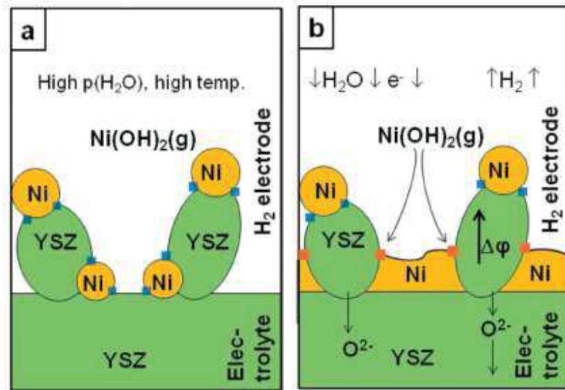
Figure 1.15. Illustration of the possible mechanism for the changes in the microstructure at the YSZ-Ni/YSZ interface observed for the high current density, a) The YSZ-Ni/YSZ interface at OCV prior to degradation at high current density electrolysis testing, 3PB are marked by blue squares, b) The YSZ-Ni/YSZ interface upon degradation at high current density electrolysis testing. The electrical potential gradient in the YSZ particles is illustrated by \uparrow\Delta\phi and the 3PB marked by red squares will be more reducing points than those 3PB marked by blue squares and the reduction of nickel hydroxide will take place at the red marked 3PB leading to a dense Ni-YSZ layer[37].
