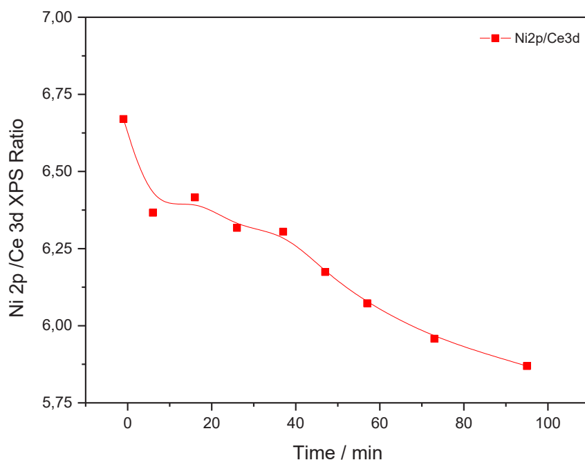
Figure 3.10. Time evolution of the Ni2p/Ce 3d peak area ratio derived by the analysis of the corresponding NAP-XPS spectra. Measurements were performed on preoxidized Ni-GDC cathode electrodes in 3:1 H 2 O/H 2 gas mixture at 640 °C and at constant current of -100 mA/cm 2 .
