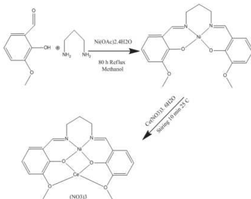
Figure 4.3. Synthesis step of \text{Ni}^{\text{II}}\text{-Ce}^{\text{III}} (N,N'-bis(3-methoxysalicylidene)-propylene-1,3-diamine).
