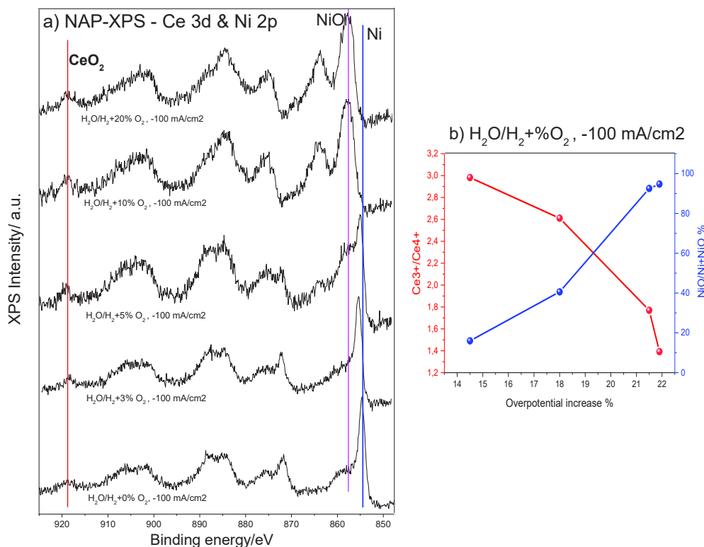
Figure 5.14. The NAP-XPS Ce 3d Ni 2p spectra measured on the 20NiCe@Ni-YSZ cathode electrode in 0.5 mbar \text{H}_2\text{O}/\text{H}_2 at 640 °C under -100 \text{ mA/cm}^2 and co-feed of \text{O}_2 (from bottom to the top). b) The evolution of \text{Ce}^{3+}/\text{Ce}^{4+} components ratio as derived by the analysis of the corresponding NAP-XPS Ce 3d spectra.
