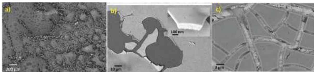
Figure. 4.5. SEM images of a \text{Ni}_{0.1}\text{Ce}_{0.9}\text{O}_{2-x} layer (a) fresh after drop casting the solution on a \text{SiO}_2/\text{Si} wafer (b) after calcination at 400 °C on a \text{SiO}_2/\text{Si} wafer and (c) after calcination at 400 °C on a Au polycrystalline foil.
