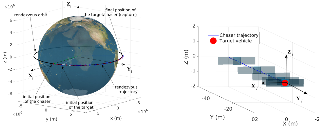
Figure 3.1: The orbit and rendezvous trajectory in \mathcal{F}_i (left) and in the LVLH frame \mathcal{F}_l (right). The trajectory corresponds to the results in section 3.6
