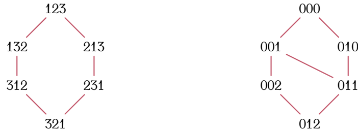
FIGURE 1.15. Hasse diagrams of S(3) and of the Lehmer code lattice of size 3.
