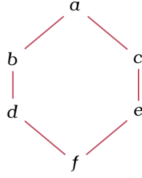
FIGURE 2.3. Counterexample of a lattice not EL-shellable.
