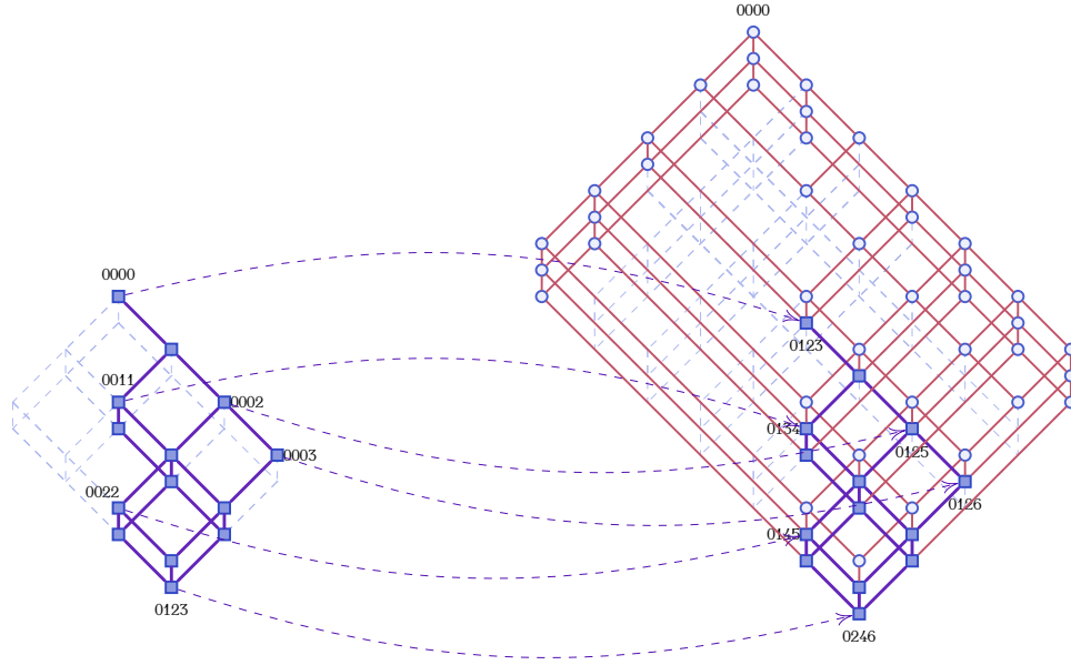
FIGURE 2.40. The subset of \text{Ca}_2(4) formed by its input-wings is isomorphic to \text{Hi}_1(4) .
