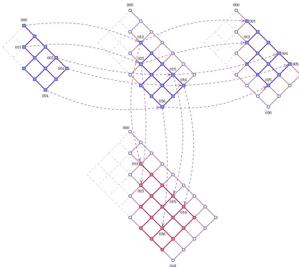
FIGURE 2.4. From the top to bottom and left to right, here are the posets Hi_2(3) , Hi_3(3) , Hi_3(3) , and Hi_4(3) . All these posets contain Hi_2(3) as subposet by restricting on input-wings, output-wings, or butterflies.
