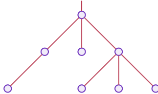
FIGURE 1.2. A rooted tree of size 8.
