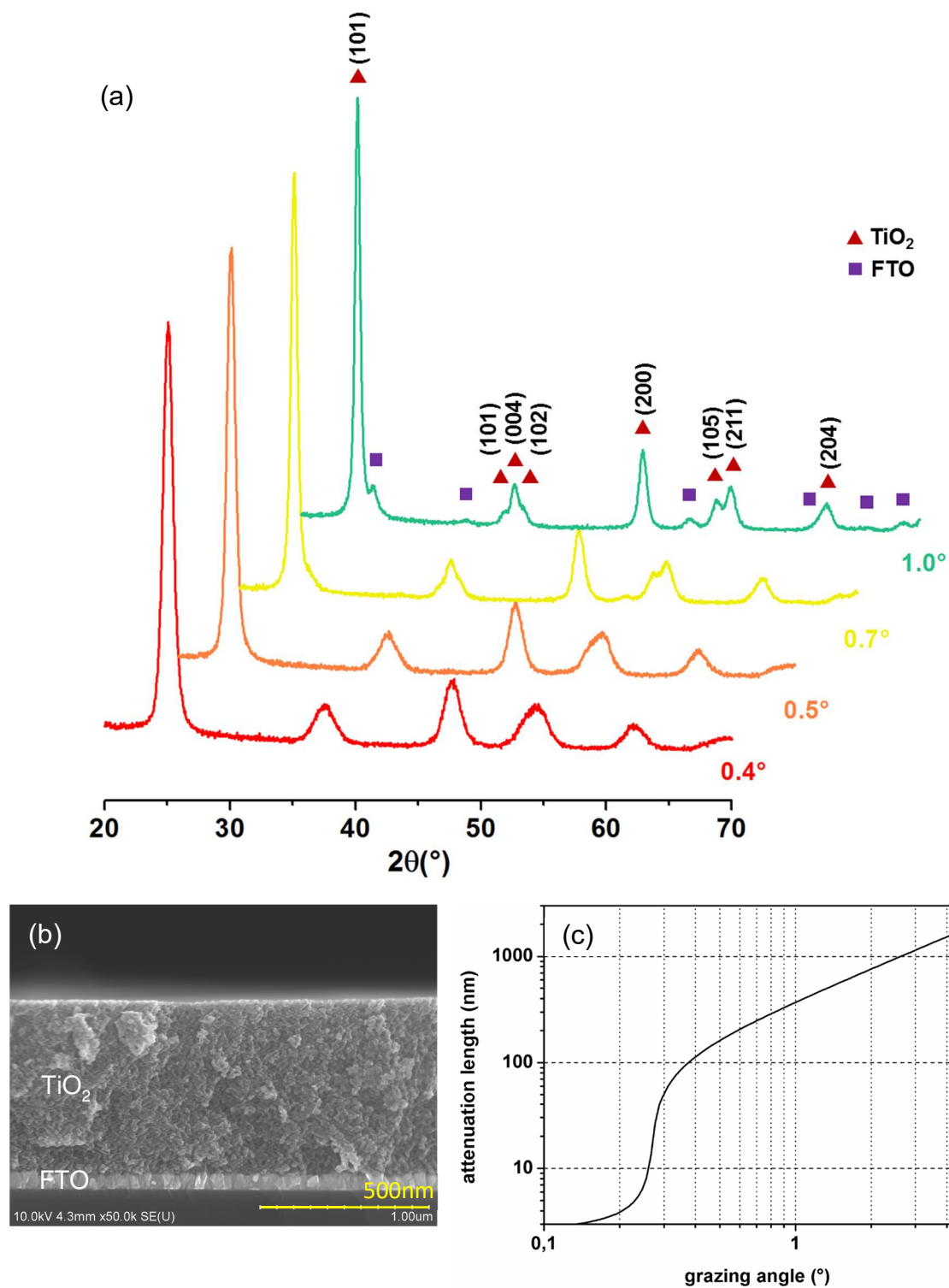
Figure 14: XRD diagram of mesoporous PB-PEO \text{TiO}_2 (2M, 1 \mu\text{m} --thick) for incident angle from 0.4° to 1.0° (a). Corresponding FEG-SEM cross section (b). Corresponding attenuation length function for a density of 85% ( \alpha_c = 0.273^\circ ) (c).
