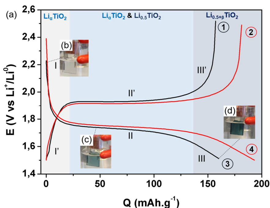
Figure 3: (a) Potential versus Capacity evolution (discharge-charge at 2C-rate) of \text{TiO}_2 mesoporous films (230 nm-thick, PB-PEO, 1M \text{TiCl}_4 ) in dark condition (black) and under light (red). (b, c, d) Pictures of the cell at the beginning of zone II and at the end of zone III. \text{Li}_{0.5}\text{TiO}_2 corresponds to a capacity of 168 \text{ mAh.g}^{-1} .
