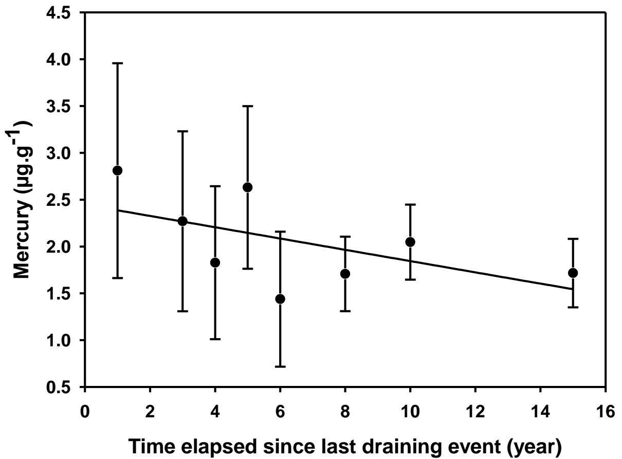
Figure 3. Relationship between the time since last draining event and Hg concentration ( r_s = -0.28 ). For each site, Hg levels are given as the mean \pm SE ( \mu\text{g}\cdot\text{g}^{-1} dw).
