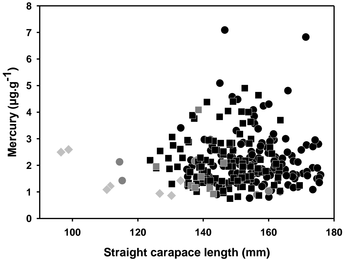
Figure 2. Relationship between turtle straight shell length (SCL) and Hg concentration ( \mu\text{g.g}^{-1} dw). Symbols stand as follow: circles represent females, squares represent males, diamond represent unsexed individuals. Black symbols represent adults, while dark grey symbols stand for juveniles.
