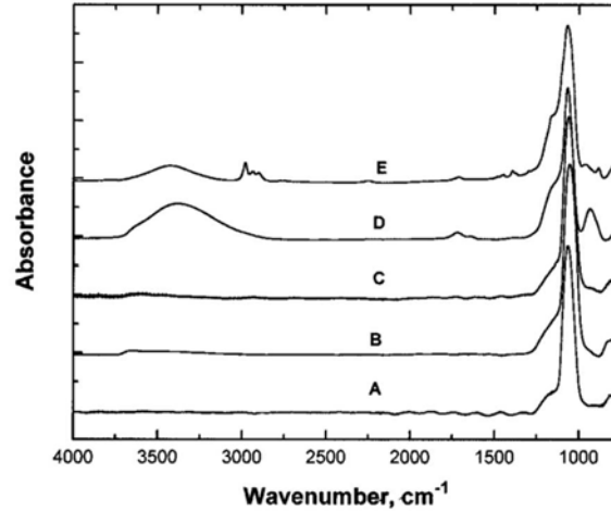
Fig. 4. Transmission FTIR spectra of the films deposited under various conditions (that are given in table 2) [17].
