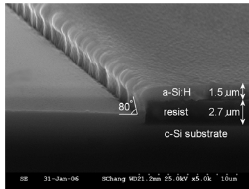
Fig. 6. SEM cross-section of a-Si:H film deposited over step of resist [2].
