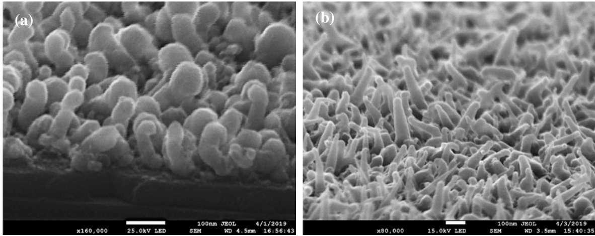
Fig. 91. SEM images of 20 nm In/50 nm a-Si samples underwent H 2 plasma treatment for different durations: (a) 10 min; (b) 30 min.
