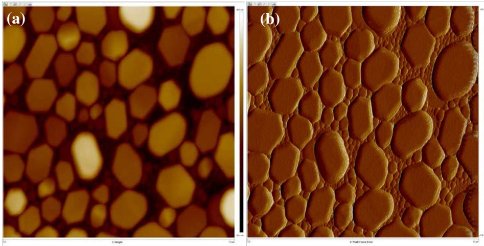
Fig. 77. AFM images of deposited indium of sample Test (mono-Si/20nm In): (a) height; (b) peak force error (scan area 1\mu\text{m}\times 1\mu\text{m} ).
