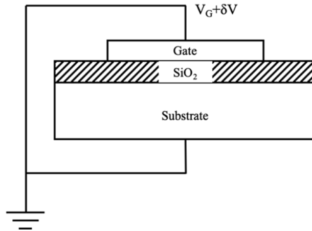
Fig. 35. Schematic of capacitance measurement setup.
