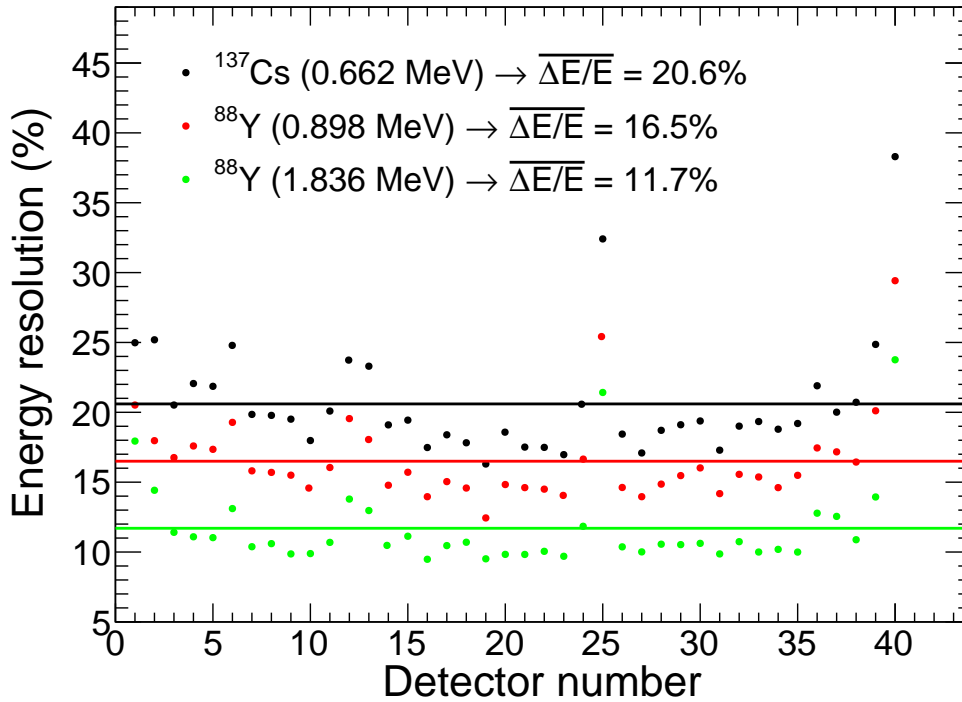
Figure 2.11: Relative resolution at three energies given by the calibration sources for each crystal of the TAC for the 238 U campaign. Similar spread was obtained for the other two uraniums but with lower average resolution for 234 U campaign. The coloured lines are the average resolution.
