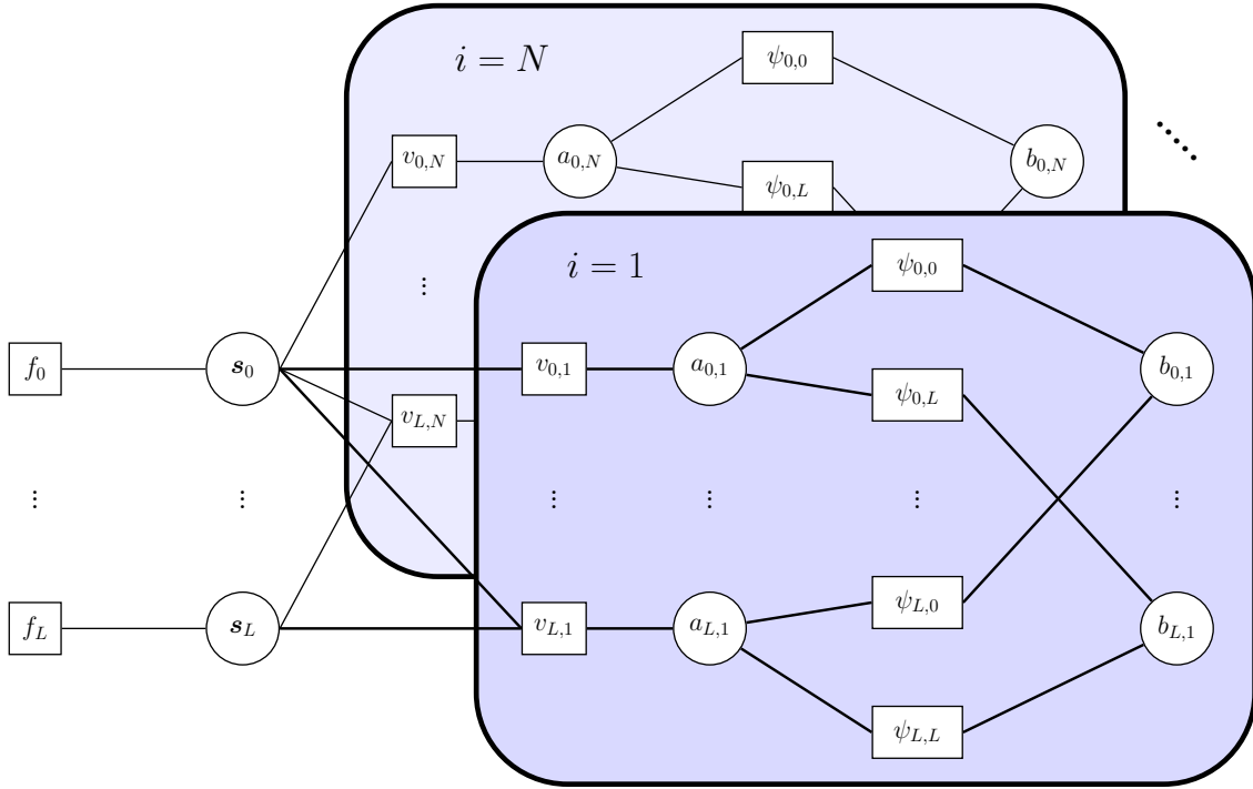
FIGURE 5.8: Factor graph with distributed BP (for performance comparison only). For notational convenience, v_{k,i} represents v(a_{k,i}, \mathbf{s}_0, \mathbf{s}_k) and \psi_{k_1,k_2} = \psi(a_{k_1,i}, b_{k_2,i}) \forall i .
