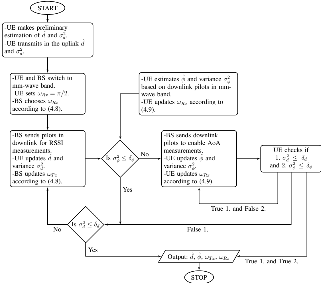
FIGURE 4.5: Flowchart representing the BS and user beam selection procedure as a part of the localization aided initial access procedure.
