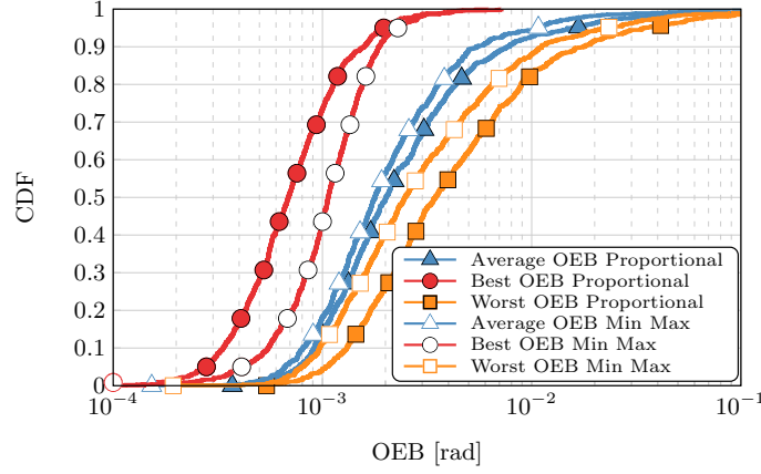
FIGURE 2.17: Empirical CDF of the OEB per user (best, worst and average performance) for different fairness strategies over 1000 MC trials.
