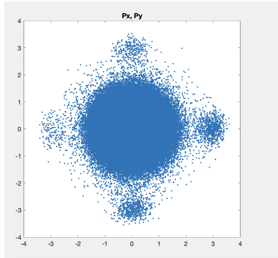
Figure 6.8: Scatter plot of \mathbf{P} on x-y plane through LAMMPS. Eight molecules are simulated in a system of side length 18.975\text{\AA} for twenty hours. The central cluster represents non-excited polarization while four lobes around are excited chain states.
