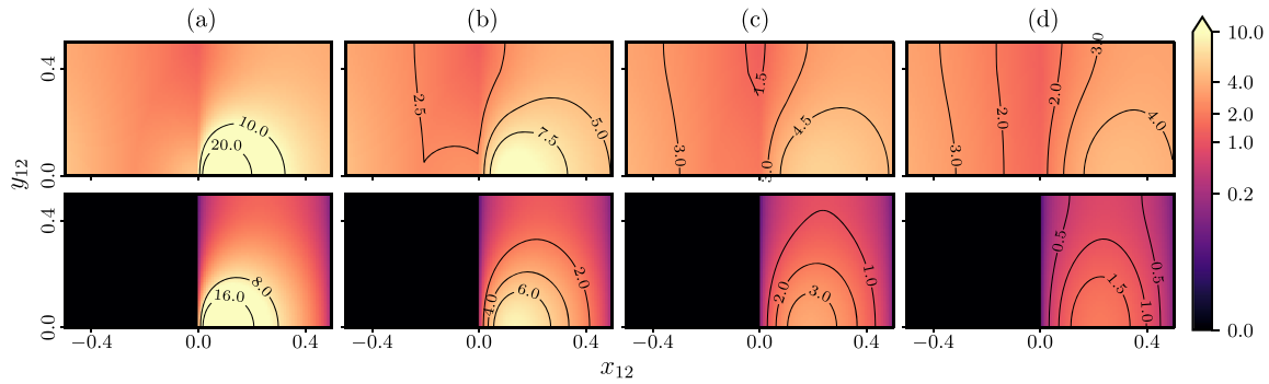
FIG. 7. Comparison of the sum of the separate-image event rates \sum_{\mathbf{n}} \beta[\tilde{q}_{((1,2), \text{Coulomb}_{\mathbf{n}}),1}(\mathbf{r}_{12})]^+ (upper row) and the merged-image event rate \beta[\tilde{q}_{((1,2), \text{Coulomb}),1}(\mathbf{r}_{12})]^+ (lower row). In all panels \mathbf{r}_{12} = (x_{12}, y_{12}, z_{12}) with (a) z_{12} = 0.1 , (b) z_{12} = 0.2 , (c) z_{12} = 0.3 , and (d) z_{12} = 0.4 . L = 1 and \beta c_1 c_2 = 1 throughout.
