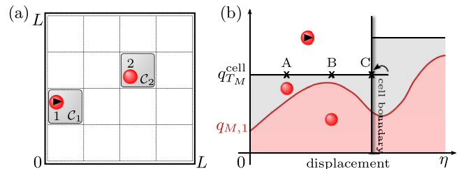
FIG. 4. Cell-veto algorithm for a two-particle factor M . (a) Active particle 1 in cell C_1 and target particle 2 in cell C_2 . (b) The event-rate q_{M,1}(\mathbf{r}_1, \mathbf{r}_2) is bounded from above by the cell-event rate q_{T_M}^{\text{cell}}(C_1, C_2) , which can be sampled trivially. A cell event may either be rejected (at point “A”) or confirmed (at point “B”) as a particle event [see Eq. (50)], while a cell event taking place outside C_1 (at point “C”) means that the active particle 1 will advance toward the cell boundary.
