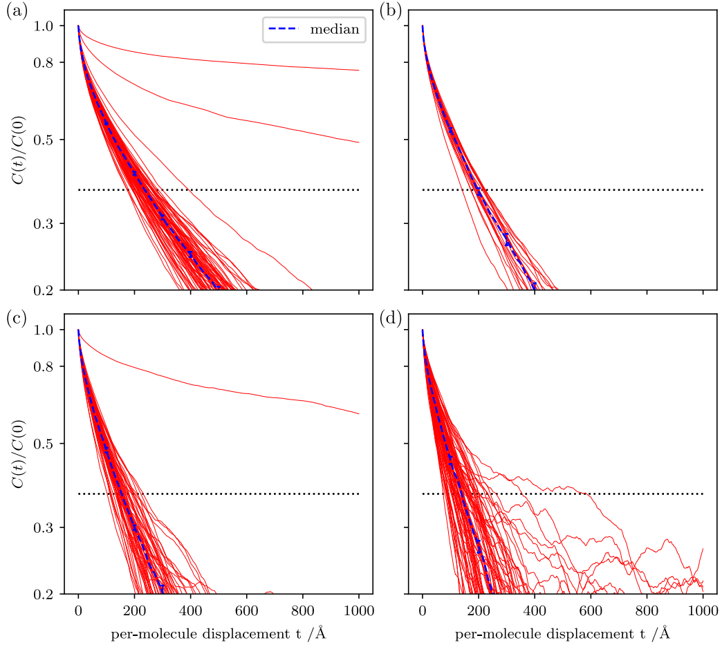
Figure 6.10: Normalized C_P of eight-molecule simulations with variable molecule translation lengths between cyclic atom mode. (a) Pure atom mode \ell_m = 0 . (b) \ell_m = 1 \text{\AA} . (c) \ell_m = 5 \text{\AA} . (d) \ell_m = 20 \text{\AA} . Error bars are obtained through bootstrapping method. Dotted lines are for y = 1/e .
