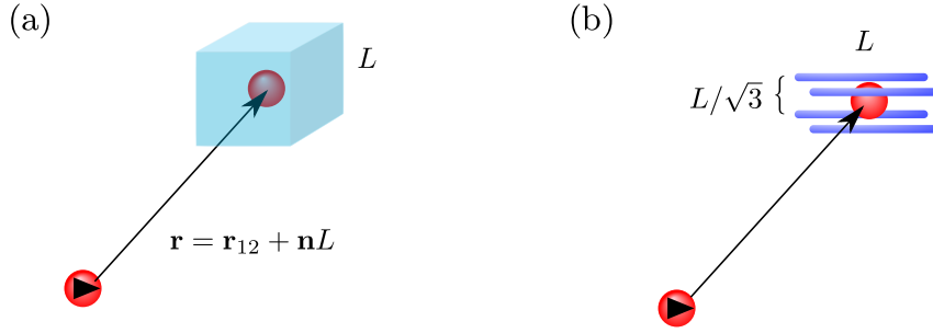
Figure 3.5: Two constructs of compensating charge with vanishing quadrupole moment. (a) Volume-charge model. (b) “Kite” model with each line of length L . The target image is in the center of the kite, and four legs of the kite make up a square of side length L/\sqrt{3} .
