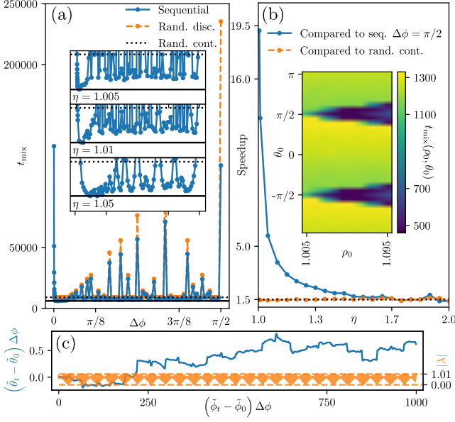
FIG. 4. Mixing times and trajectories for general \Delta\phi (a): t_{\text{mix}} at \eta = 1.005 compared to mixing times of random discrete and continuous MCMC. Inset: t_{\text{mix}} for small \Delta\phi and \eta \gtrsim 1 . (b): Optimal speedup with respect to \Delta\phi = \pi/2 and to random continuous MCMC. Inset: Dependence on \rho_0 and \theta_0 for \eta = 1.1 and \Delta\phi = \pi/180 . (c): \bar{\theta}_t and \lambda_t for \eta = 1.01 and \Delta\phi = 85\pi/180 .
