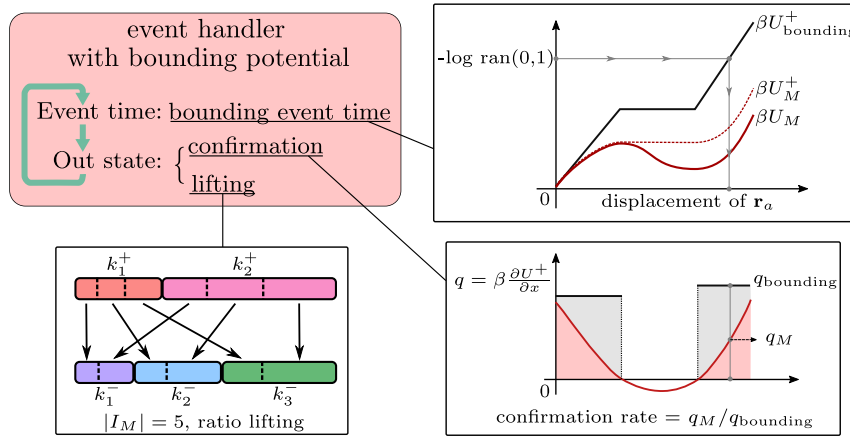
Figure 5.1: Schema of event handler with bounding potential. Displacements concerning only bounding potentials are drawn during send_event_time . Event confirmations and lifting changes are done within send_out_state .
