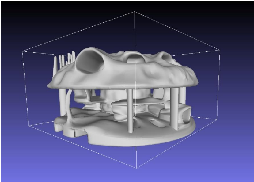
Figure IV-3: representation on MeshLab of the 3D CAD model of the module designed by Boskalis. The box surrounding it is the its bounding box that correspond to the volume occupied by the module. The dimension of the bounding box is used to compute the parameters Topo and Poro .
