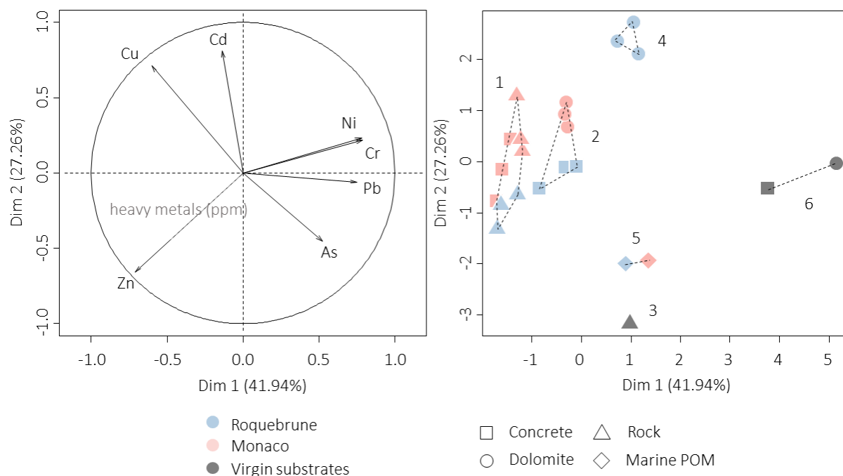
Figure III-11: Principal component analysis on the percentage of heavy metals within the biofilm, the sinking material and the virgin substrates used for the biofilm monitoring at D28 on both sites (Monaco and Roquebrune): A) Correlation circle of the variables, B) and ordination of the samples on the first two dimensions
