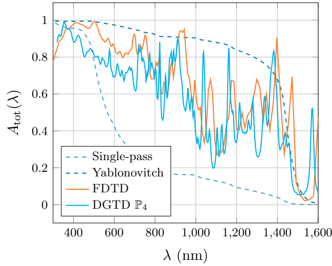
Figure 5.23 | Superposition of our results with theoretical limits.
