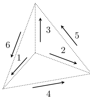
Figure 4.3 | The d.o.f. are associated to the edges of the element to naturally satisfy the continuity requirements for the approximated vector fields.
