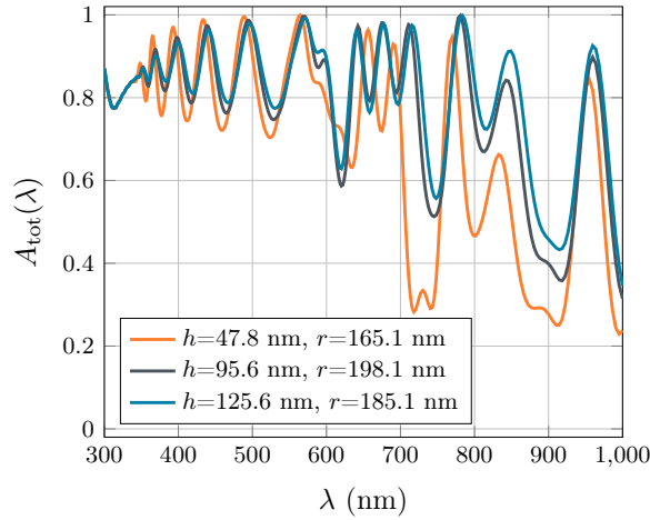
Figure 5.15 | Absorption coefficient for various textures with DGTD- \mathbb{P}_3 method. Computation times for each configuration are respectively 1181 sec, 3062 sec and 2572 sec.
