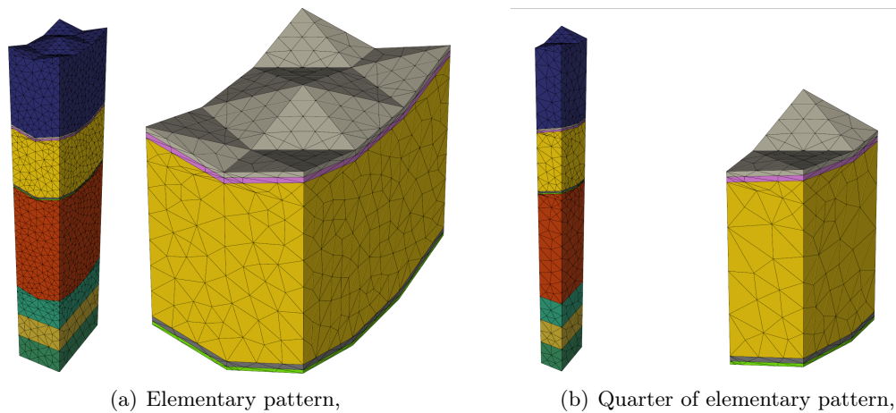
Figure 5.10 | Unit pattern with an isolation of the very thin Si-based layers.
