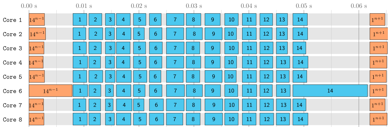
Figure 6.3 | DIOGENeS-DGTD traces: focus on the main time loop. Isolation of one iteration of DIOGENeS-DGTD with LRSK-14-5 time scheme on 8 cores. The highlighted iteration corresponds to the update of the reflection observable.
