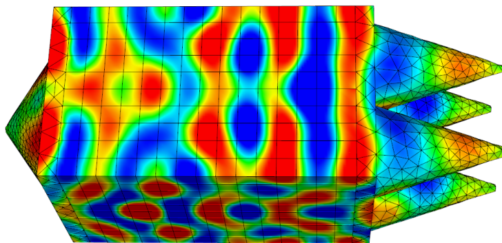
Figure 3.11 | Simulation of light trapping in a solar cell based on nanocone gratings. Simulations using hybrid mesh: contour lines of the module of the DFT of \mathbf{E} for a wavelength \lambda = 450 nm.
