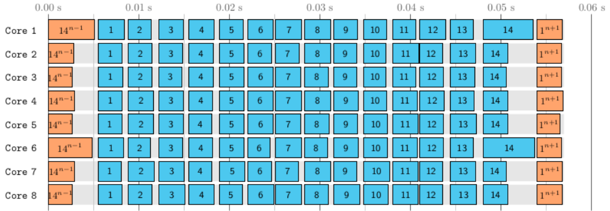
Figure 6.11 | DIOGENeS-DGTD traces: focus on the main time loop. Isolation of one iteration of DIOGENeS-DGTD with LRSK-14-5 time scheme on 8 cores. The highlighted iteration corresponds to the update of the reflection observable.
