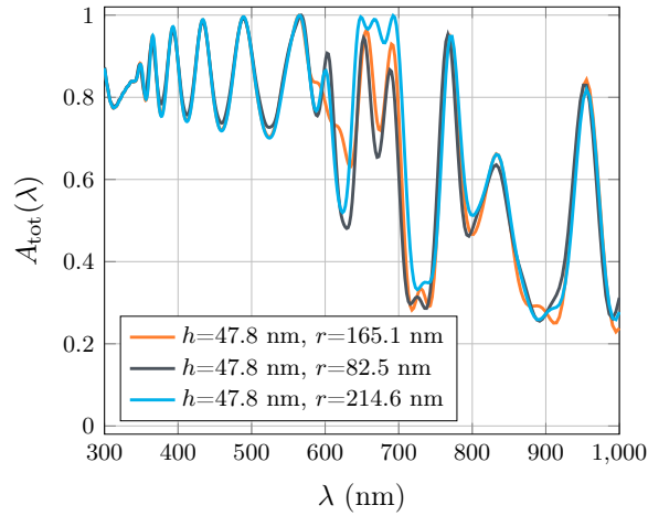
Figure 5.13 | Absorption coefficient for various textures obtained with DGTD- \mathbb{P}_3 method. Computation times for each configuration are respectively 1181 sec, 1360 sec and 1356 sec.
