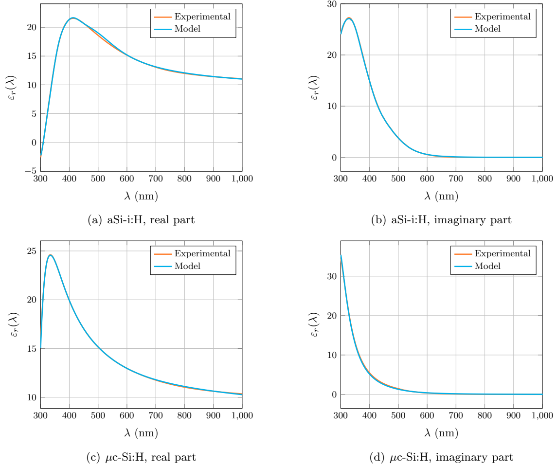
Figure 4.45 | Real and imaginary parts of the relative permittivity of front TCO, a-Si:H, \mu\text{c-Si:H} and back TCO predicted by our dispersive model compared to experimental data.
