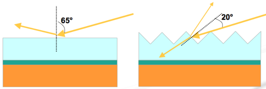
Figure 1.3 | Standard solar glass (left) versus light trapping (right). Source: Saint Gobain
