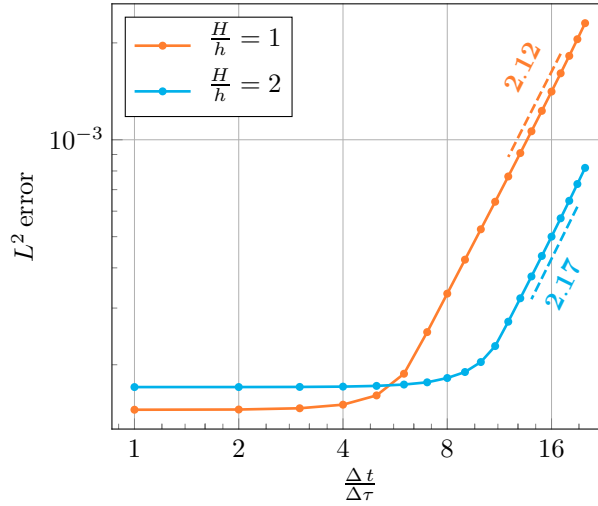
Figure 7.8 | Convergence study of MHM-DGTD method with LTS with (p^e, p^K) = (1, 3) , for fixed “small enough” (h, \Delta\tau, H) with H = 3.12e-2 , \Delta\tau = \frac{Ch}{10} and \Delta t \rightarrow 0 (right to left).
