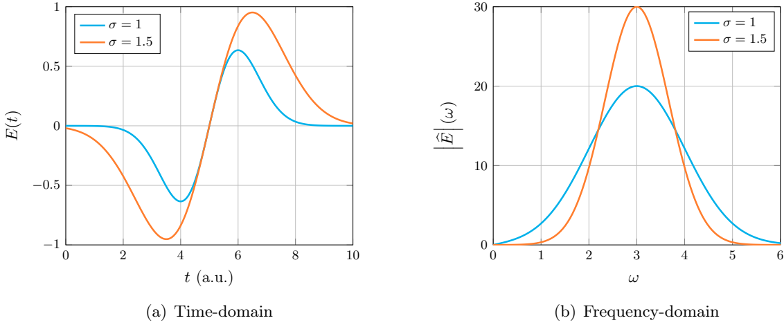
Figure 2.15 | Wideband pulse representation in time-domain and frequency-domain. Parameters are E_0 = 20 \text{ V}\cdot\text{m}^{-1} , \omega_0 = 3 , t_0 = 5 . The shorter the time-domain pulse, the wider the frequency-domain spectrum.
