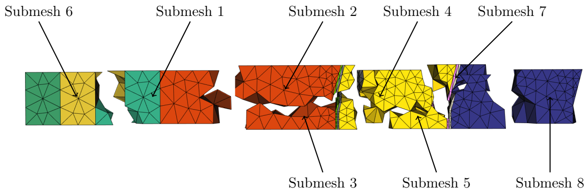
Figure 6.10 | Exploded view of partitions of the PV glass presented in section 5.2.
