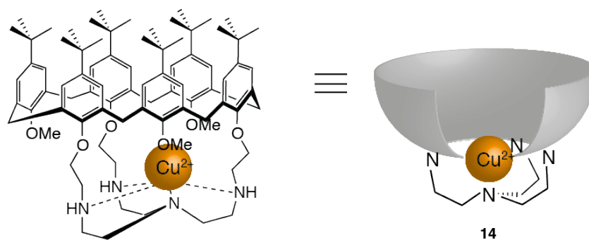
Figure I-3: Calix[6]trenCu 14 and its schematic representation.
