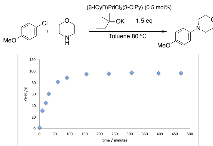
Figure IV-31: Reaction conditions and kinetic profile of the ( \beta -ICyD)PdCl 2 (3-CIPy) catalyzed Buchwald-Hartwig amination of 4-chloroanisole.
