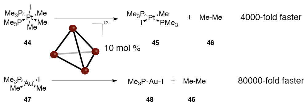
Scheme I-26: Reductive elimination of 44 and 45 catalyzed by 32
