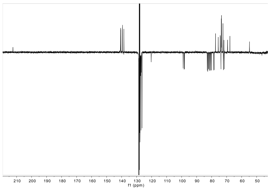
Figure S26: ^{13}\text{C-NMR} of \alpha\text{-ICyD 159} . ( \text{C}_6\text{D}_6 , 101 MHz, 300 K)
