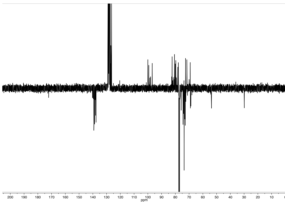
Figure S29: ^{13}\text{C} -Jmod of the 77:23 mixture of 160:127 ( \text{CDCl}_3 , 600 MHz, 300 K)
