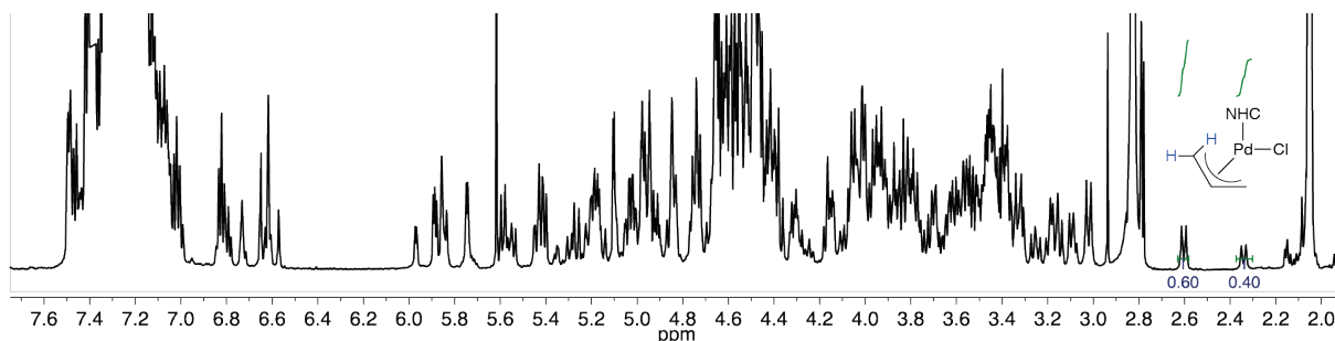
Figure III-36: ^1\text{H-NMR} of (\gamma\text{-AE-ICyD})\text{PdCl}(\eta^3\text{-allyl}) . Acetone- \text{d}_6 , 600 MHz, 300 K.
