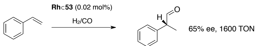
Scheme I-28. Hydroformylation reaction catalyzed by RhC53
