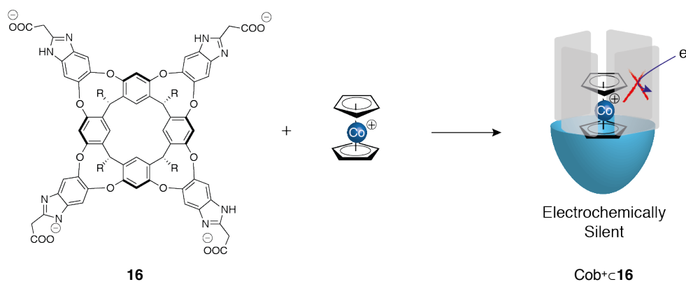
Scheme I-10: Formation of the electrochemically silent inclusion complex \text{Cob}^+\text{c16} .
