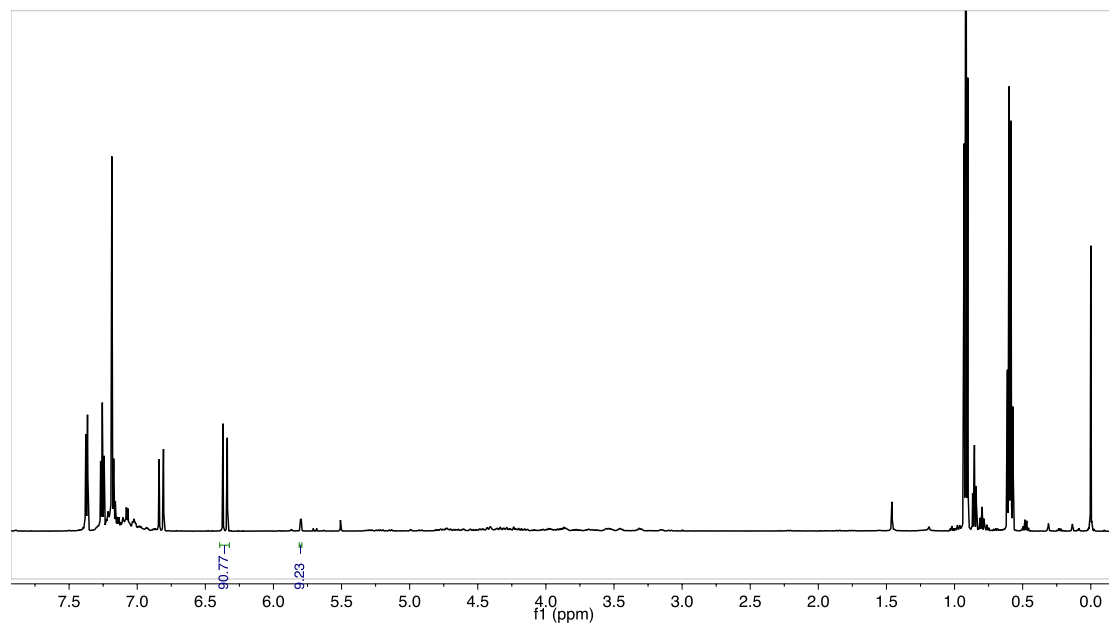
Figure S111: Crude 1 H-NMR of the reaction with ( \beta -rev-ICyD)Pt(dvtms) (CDCl 3 , 600MHz, 300K)
