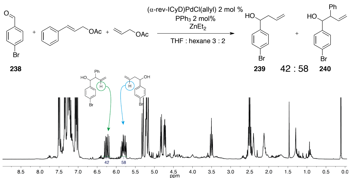
Figure IV-39: Reaction conditions for the “substrate selection” with (\alpha\text{-rev-ICyD})\text{PdCl}(\text{allyl})
