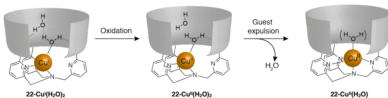
Scheme I-13: Mechanism of the redox behavior of 22
