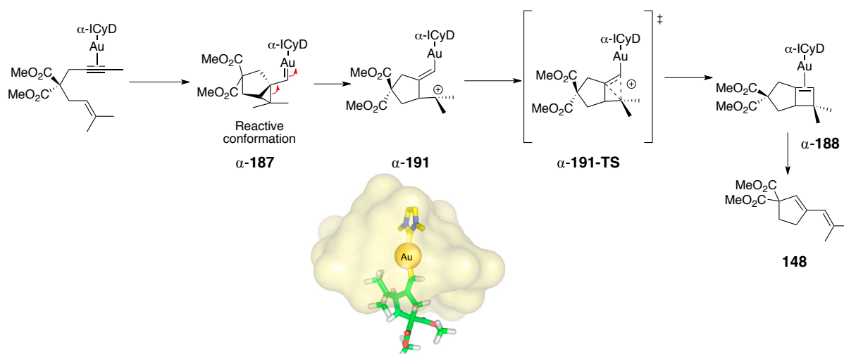
Scheme IV-3: Mechanistic pathway and TS for the (\alpha\text{-ICyD})\text{AuCl} catalyzed formation of 149
