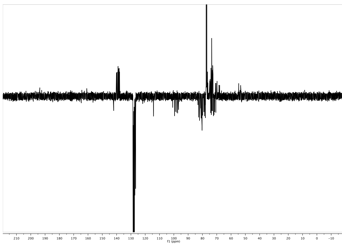
Figure S95: ^{13}\text{C-NMR} of 224 ( \text{CDCl}_3 , 151 MHz, 300 K)
