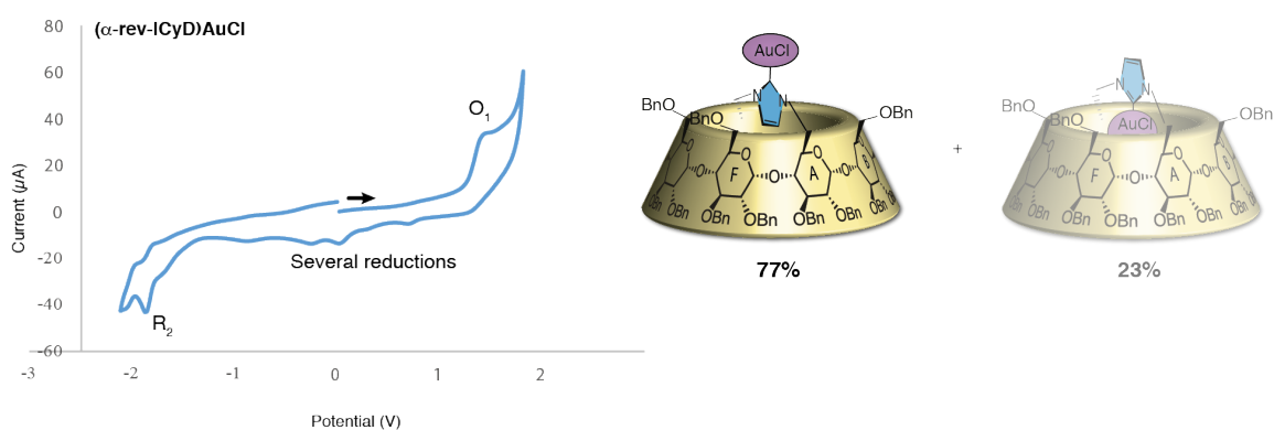
Figure III-32: Cyclic voltammogram of (\alpha\text{-rev-ICyD})\text{AuCl} complex. MeCN 0.5 V/s, [(\text{ICyD})\text{AuCl}] = 2\text{ mM} , 0.1M \text{TBAPF}_6 as supporting electrolyte.
