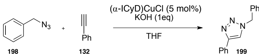
Scheme I-7: ( \alpha -ICyD)CuCl catalyzed synthesis of triazole 199
