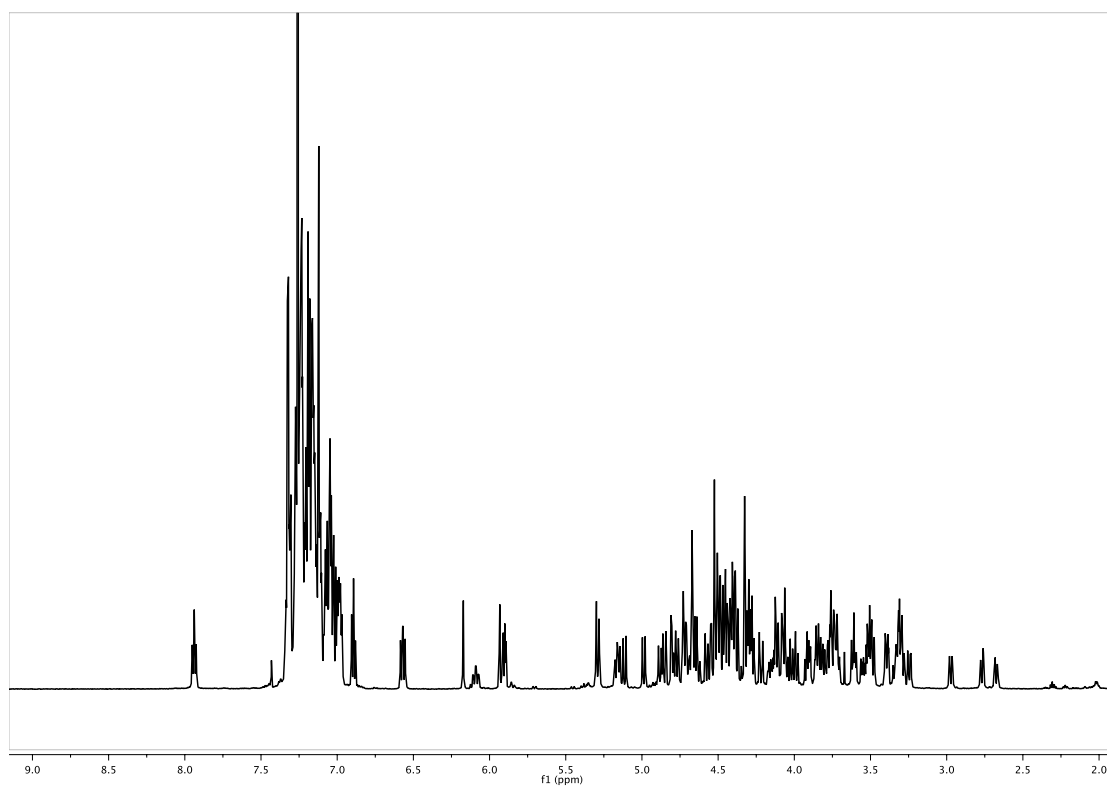
Figure S94: ^1\text{H-NMR} of 224 ( \text{CDCl}_3 , 600 MHz, 300 K)
