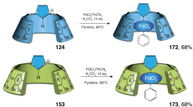
Scheme III-19: Synthesis of (γ-ICyD)PdCl 2 (pyridine) and (β-ICyD)PdCl 2 (pyridine).
