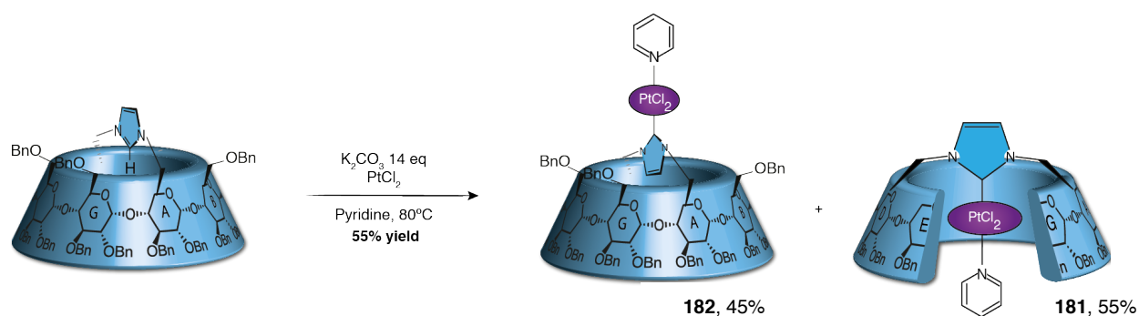
Scheme III-27: Synthesis of ( \beta -rev-ICyD)Pt(pyridine)
