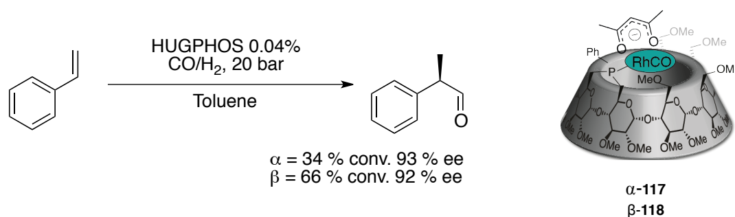
Scheme II-8 : HUGPHOS catalyzed hydroformylation of styrene.
