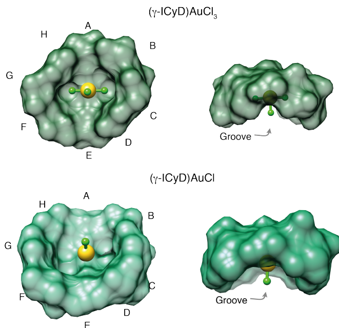
Figure III-20: Bottom and side views of the Connolly's surfaces of (\gamma\text{-ICyD})\text{AuCl}_3 and (\gamma\text{-ICyD})\text{AuCl}
