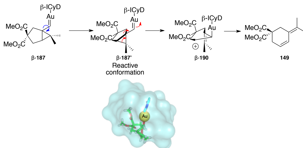
Scheme IV-4: Calculated mechanistic pathway and conformation for the (\beta\text{-ICyD})\text{AuCl} catalyzed formation of 149 .
