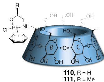
Figure II-8: Structure of (CD)Rh complexes 110 and 111
