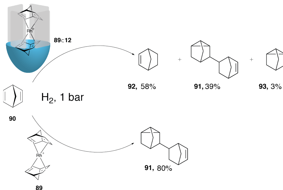
Scheme I-39: Product distribution catalyzed by 89c12
