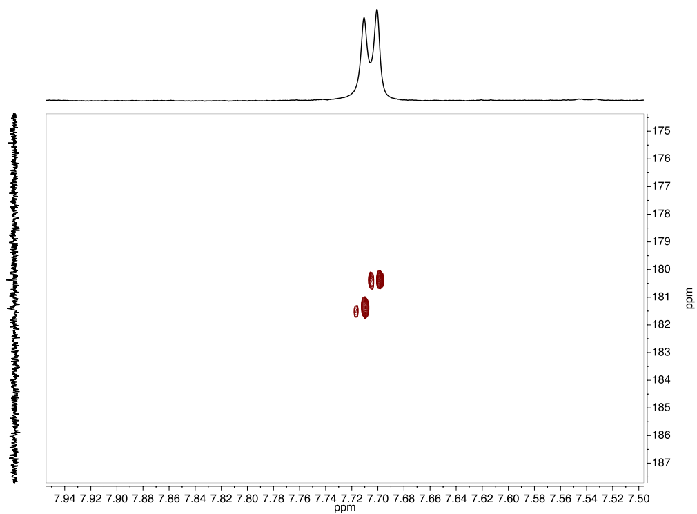
Figure S66: HMBC of 175 showing the presence of two C=Pd (CDCl 3 , 300 K)
