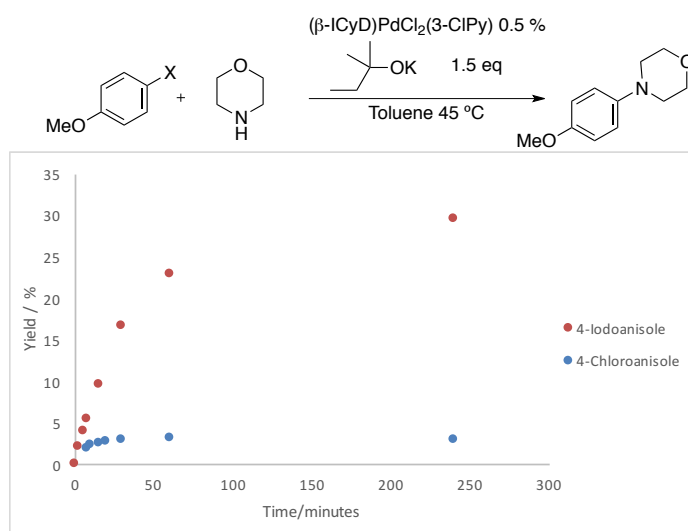
Figure IV-33: Reaction conditions and kinetic profile of the (\beta\text{-ICyD})\text{PdCl}_2(3\text{CIPy}) catalyzed Buchwald-Hartwig amination at 45 °C.
