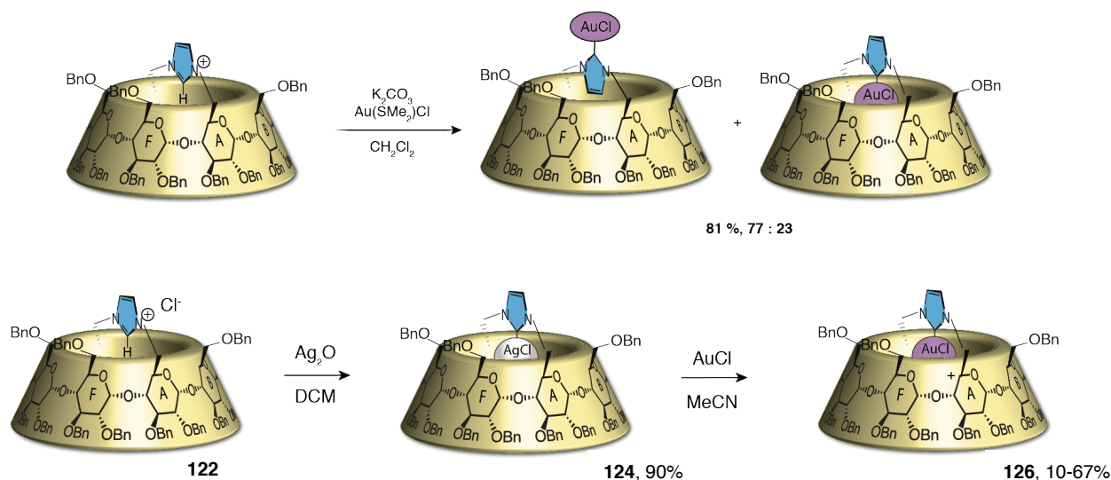
Scheme III-8: Synthesis of ( \alpha -ICyD)AuCl and ( \alpha -rev-ICyD)AuCl
