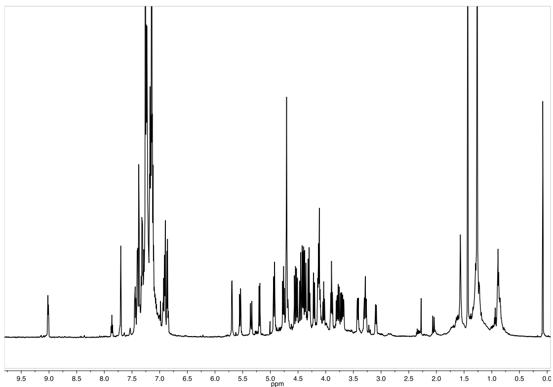
Figure S69: ^1\text{H-NMR} of (\alpha\text{-rev-ICyD})\text{PtCl}_2(\text{pyridine}) 180 ( \text{CDCl}_3 , 600 MHz, 300 K)
