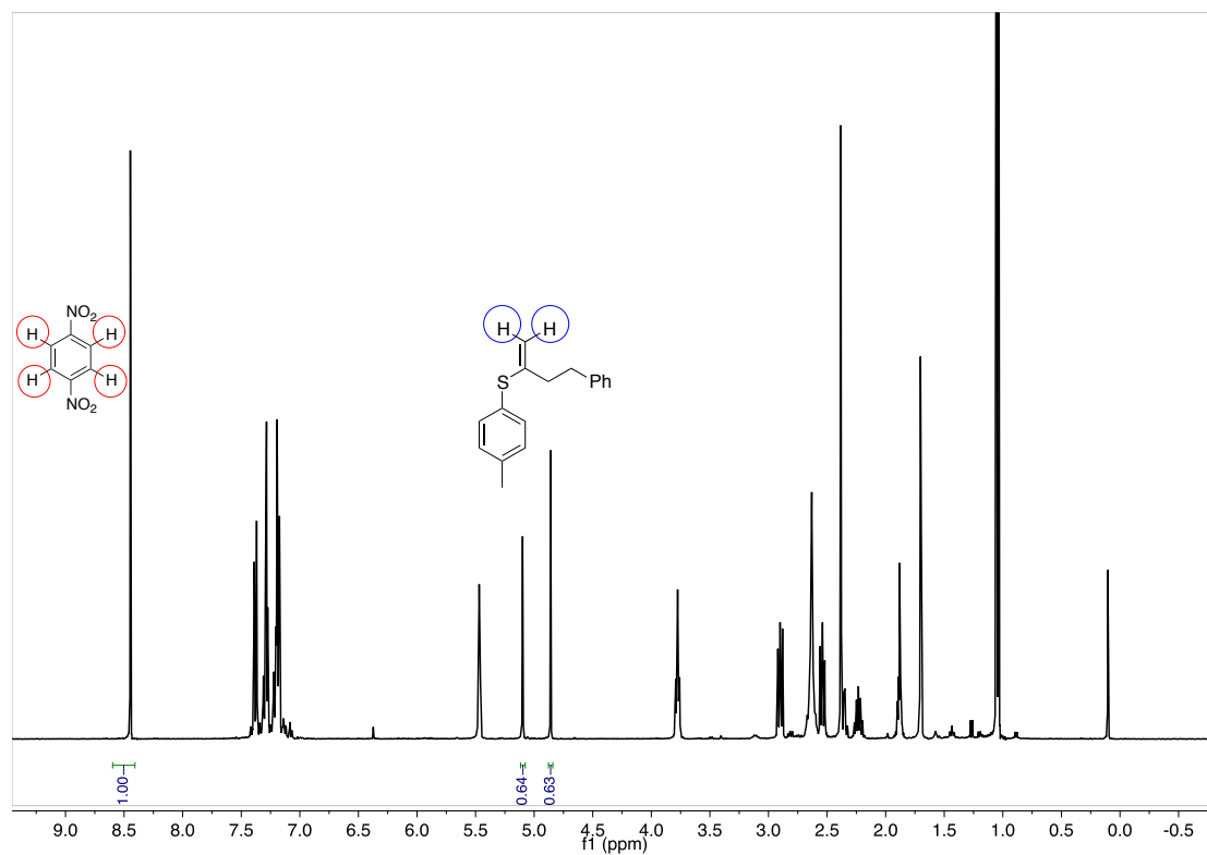
Figure S107: Crude 1 H-NMR of 209 (CDCl 3 , 400 MHz, 300 K)
