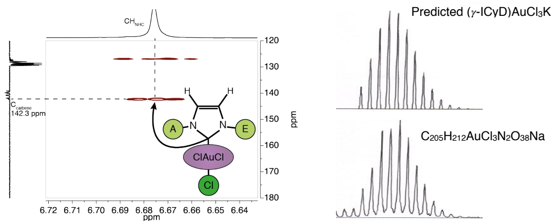
Figure III-15 : HMBC of ( \gamma -AE-ICyD)AuCl 3 showing the chemical shift of the C carbene . HMBC: CD 3 CN, 400MHz, 300K ESI-TOF: Injection in MeCN
