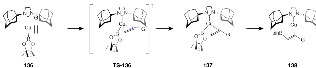
Scheme II-13: Proposed mechanism of the regiodeterminant step of (SIAd)CuCl ligands.
