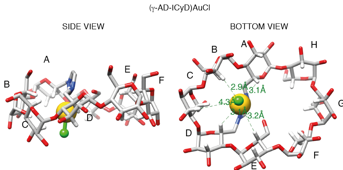
Figure II-5: Modeled structure of ( \gamma -AD-ICyD)AuCl.
