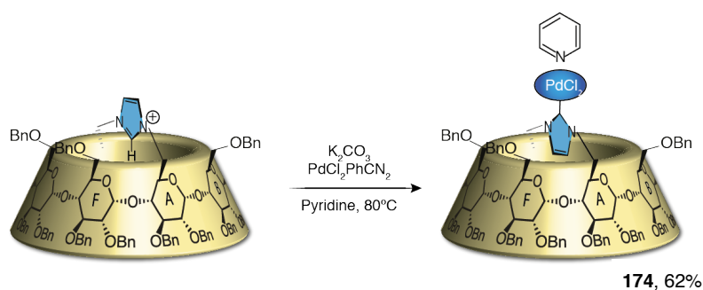
Scheme III-20: Synthesis of (α-rev-ICyD)PdCl 2 (pyridine) complex.
