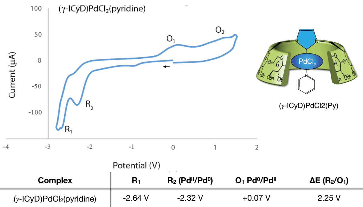
Figure III-64: Cyclic voltammogram of (\gamma\text{-ICyD})\text{PdCl}_2(\text{pyridine}) [(\text{ICyD})\text{PdCl}_2] = 1.5 \text{ mM} . TBABF 4 0.1M, GC 3 mm, CE Pt wire, SCE, 20°C, 0.5 V/s.
