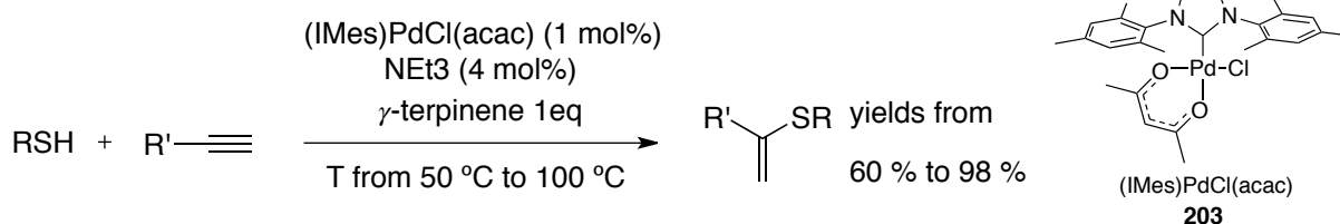
Scheme IV-8: Pd-NHC catalyzed synthesis of branched vinyl sulfides.
