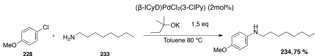
Scheme IV-32: ( \beta -ICyD)PdCl 2 (3-CIPy) catalyzed cross-coupling of octylamine with 4-Cl-anisole.
