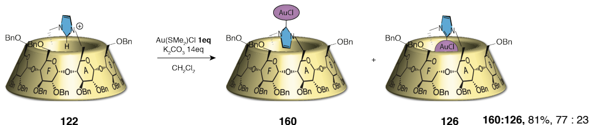
Scheme III-7: Reaction of \alpha -CyDHCl with K_2CO_3 and Au(Me_2S)Cl
