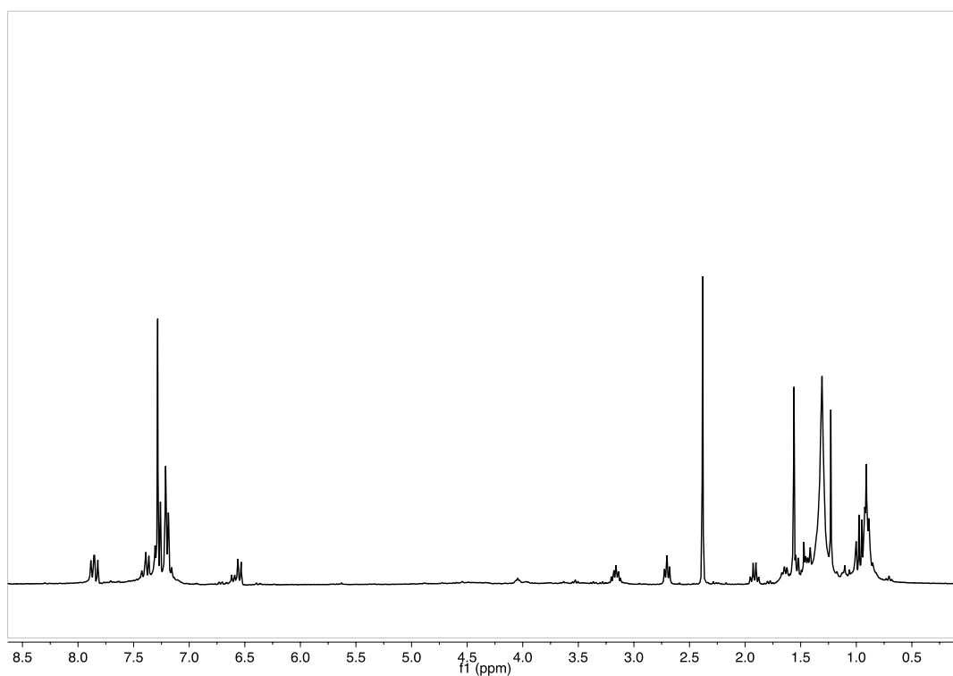
Figure S115: ^1\text{H-NMR} of 237 ( \text{CDCl}_3 , 400 MHz, 300 K)
