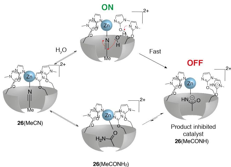
Scheme I-16: Proposed mechanism for the hydrolysis of the acetonitrile
