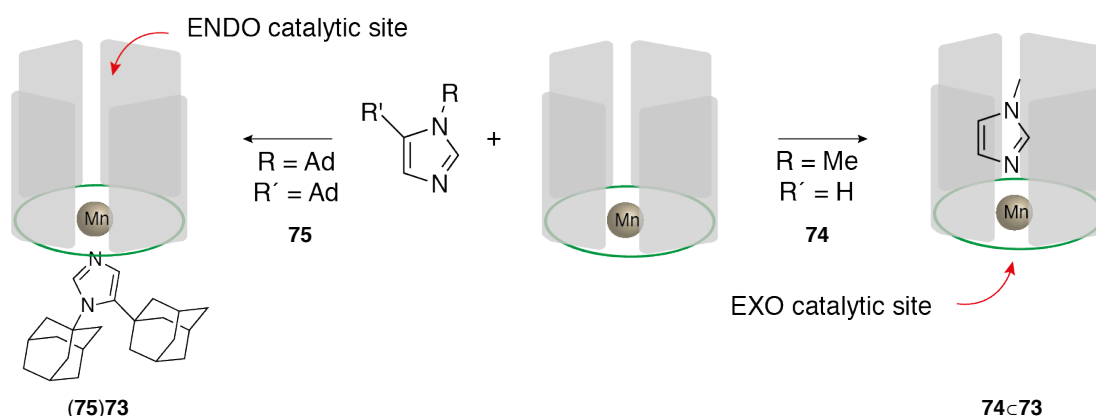
Scheme I-35: Coordination modes of 74 \subset 73 and ( 75 ) 73 .
