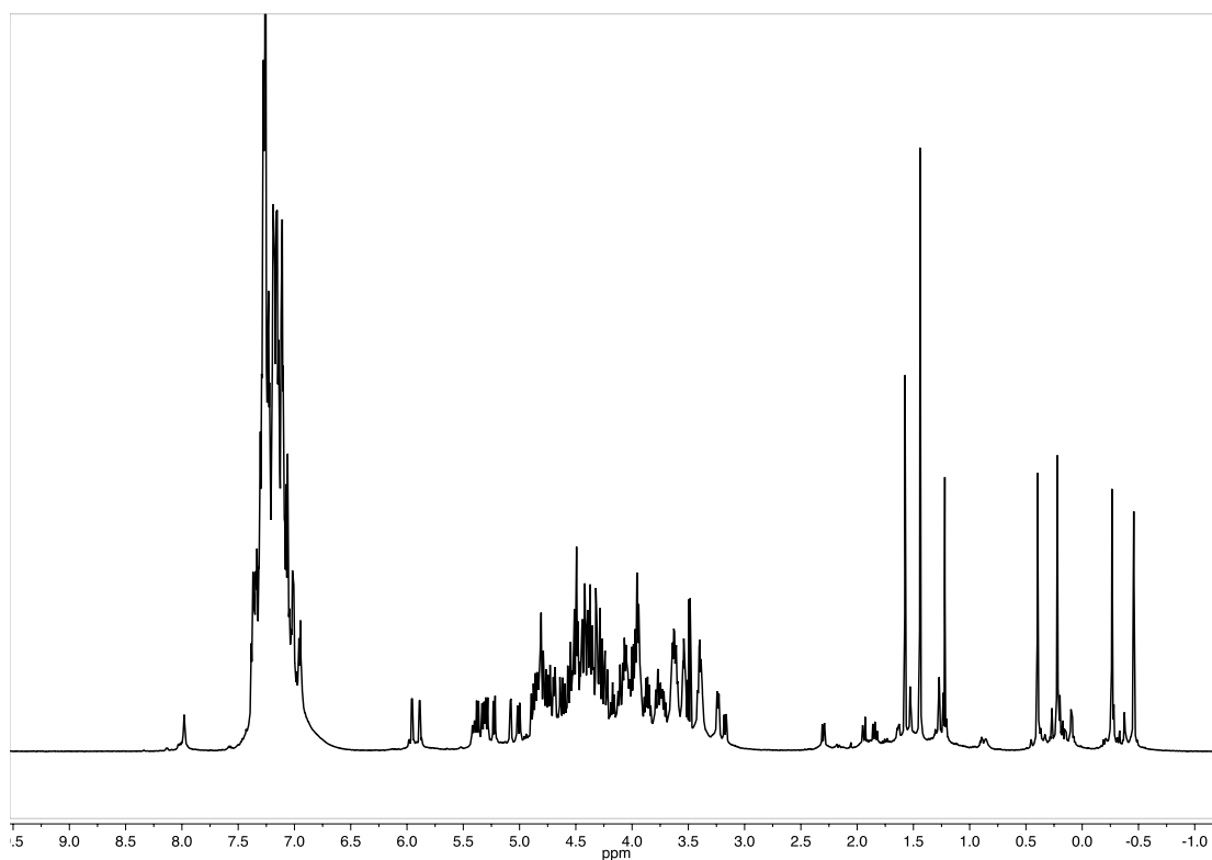
Figure S76: ^1\text{H-NMR} of (\beta\text{-rev-ICyD})\text{Pt}(\text{dvtms}) 183 ( \text{CDCl}_3 , 600 MHz, 300 K)
