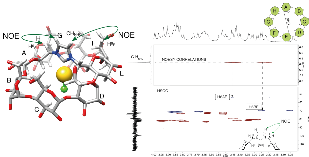
Figure III-2: NOESY (top) and HSQC (bottom) of ( \gamma -AE-ICyD)AuCl 157 complex showing cross-correlations between the C-H of the imidazole and two H6. \text{CD}_3\text{CN} , 600 MHz, 300K
