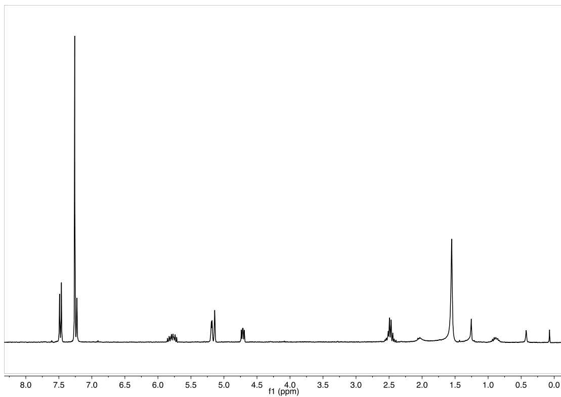
Figure S120: ^1\text{H-NMR} of 239 ( \text{CDCl}_3 , 400 MHz, 300 K)
