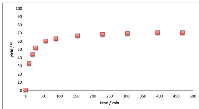
Figure IV-32: Reaction conditions and kinetic profile of the (\beta\text{-ICyD})\text{PdCl}_2(3\text{CIPy}) catalyzed Buchwald-Hartwig amination of 4-iodoanisole.
