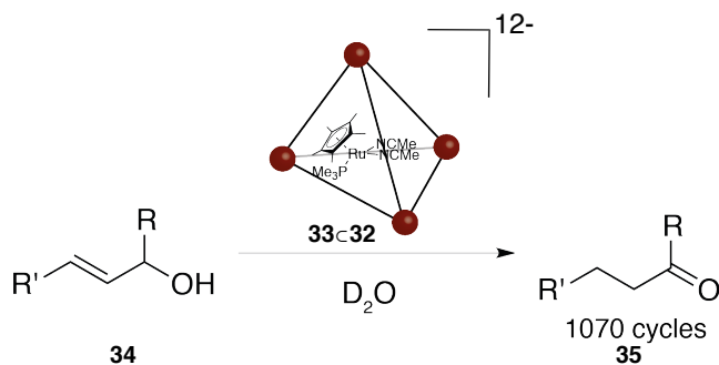
Scheme I-21: Allyl isomerization catalyzed by 33c32
