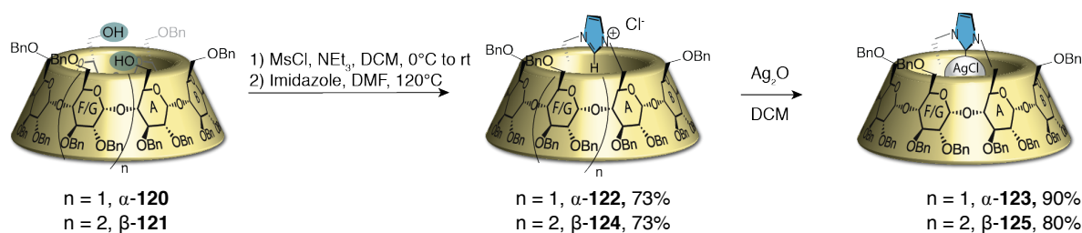
Scheme II-11: Synthesis of (α-ICyD)AgCl and (β-ICyD)AgCl.
