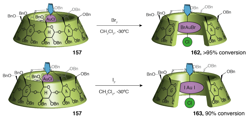
Scheme III-12 : Oxidations with \text{Br}_2 and \text{I}_2 of (\gamma\text{-ICyD})\text{AuCl}
