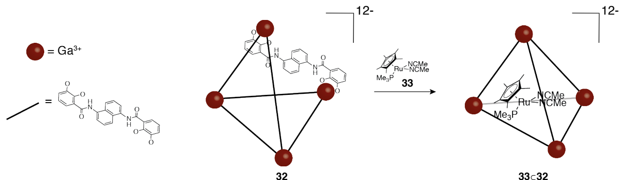
Scheme I-20: Structure and encapsulation of the 33c32
