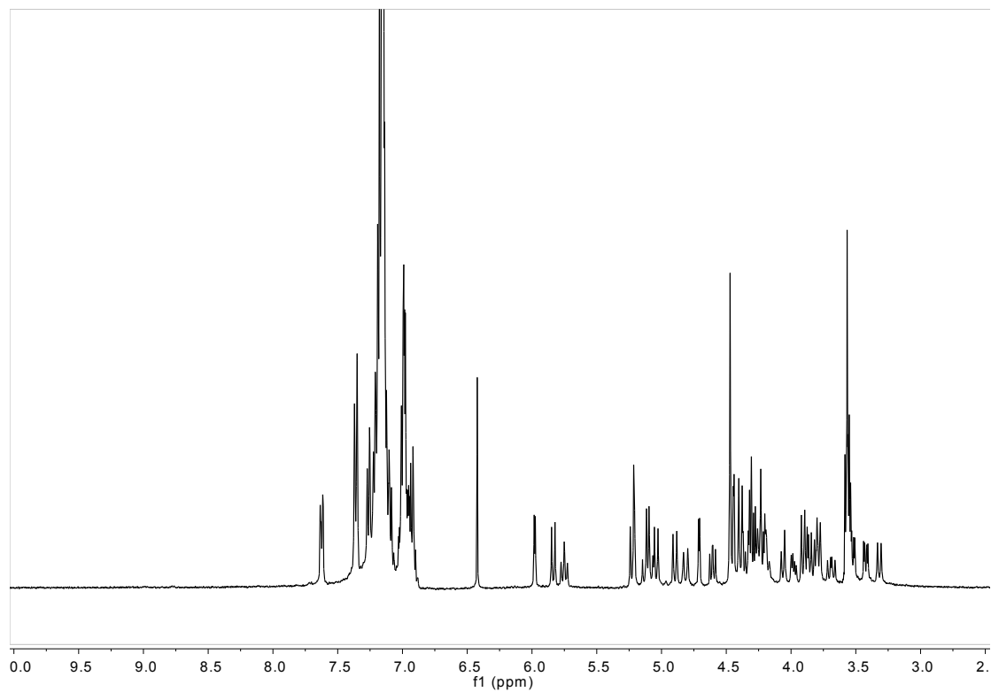
Figure S25: ^1\text{H-NMR} of \alpha\text{-ICyD 159} . ( \text{C}_6\text{D}_6 , 400 MHz, 300 K)
