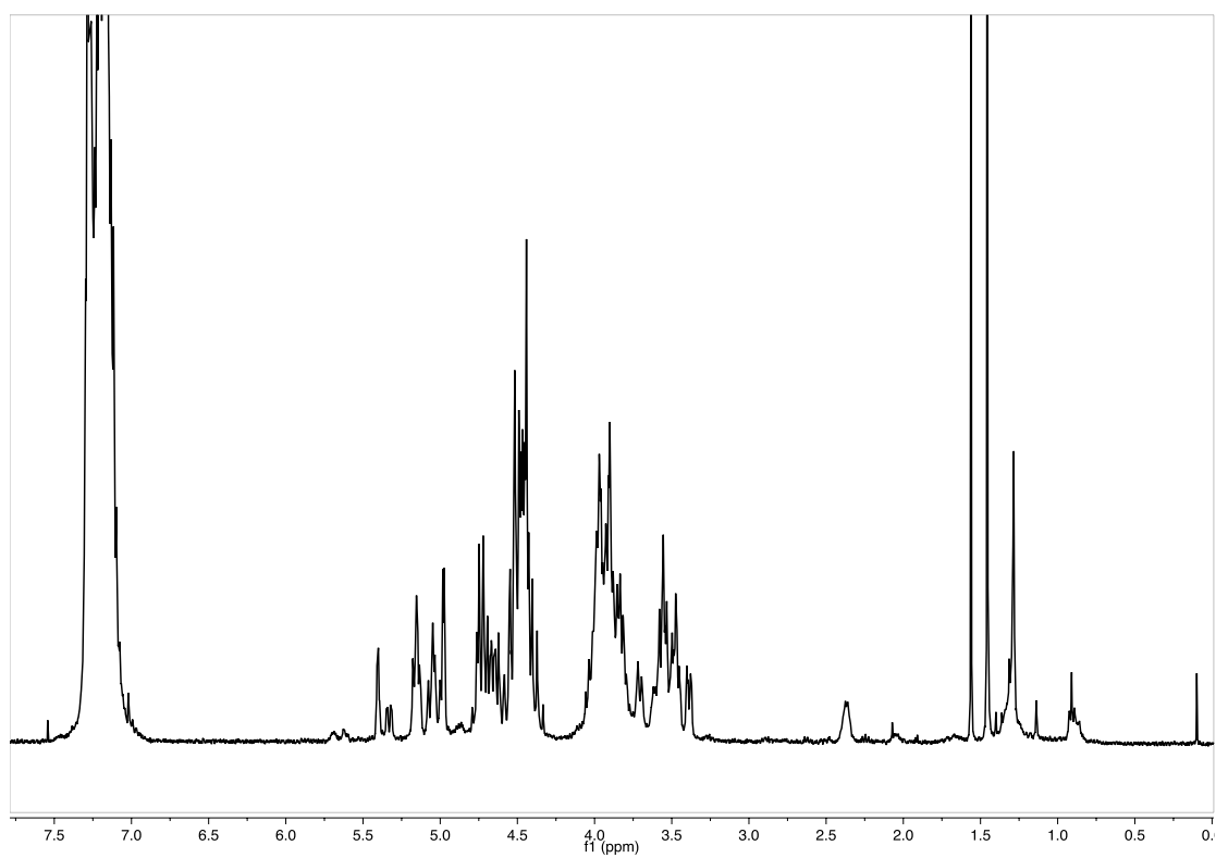
Figure S9: ^1\text{H-NMR} of the mixture of \gamma\text{-AD-CD(OH)}_2 and \gamma\text{-AE-CD(OH)}_2 150
