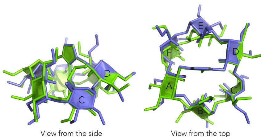
Figure II-16 : Superimposition of modeled ( \alpha -ICyD)AgCl (blue) with the DFT calculated structure (green).
