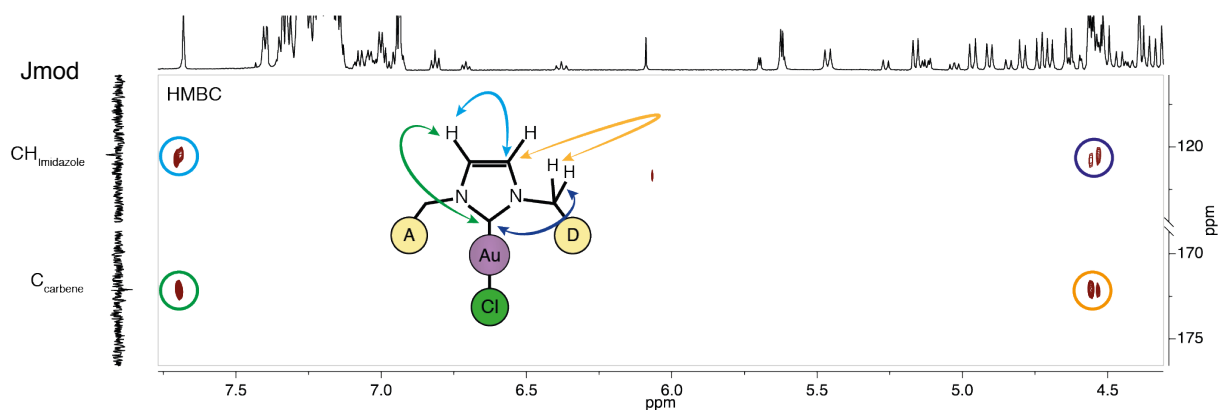
Figure III-10: Extract of HMBC showing all the cross correlations between the carbons of the NHC moiety and the surrounding protons \text{CDCl}_3 , 600 MHz, 300K
