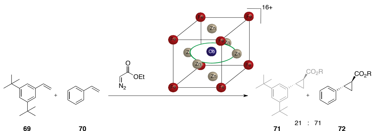
Scheme I-34: Competitive substrate selective reaction catalyzed by the Fe@Zn 16
