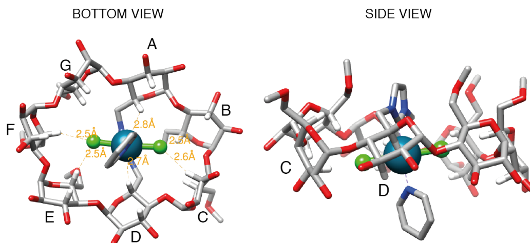
Figure III-56: Top view and side view of the modeled structures of ( \beta -ICyD)PdCl 2 (pyridine).
