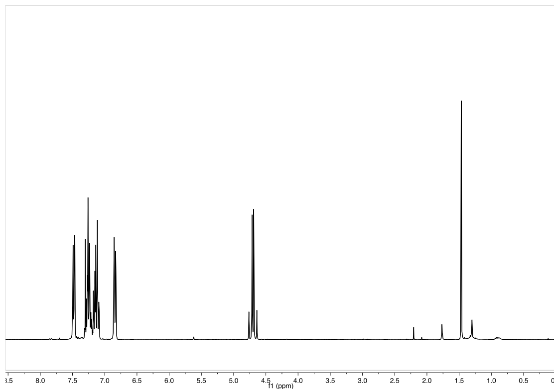
Figure S104: 1 H-NMR of 199 (CDCl 3 , 600 MHz, 300 K)
