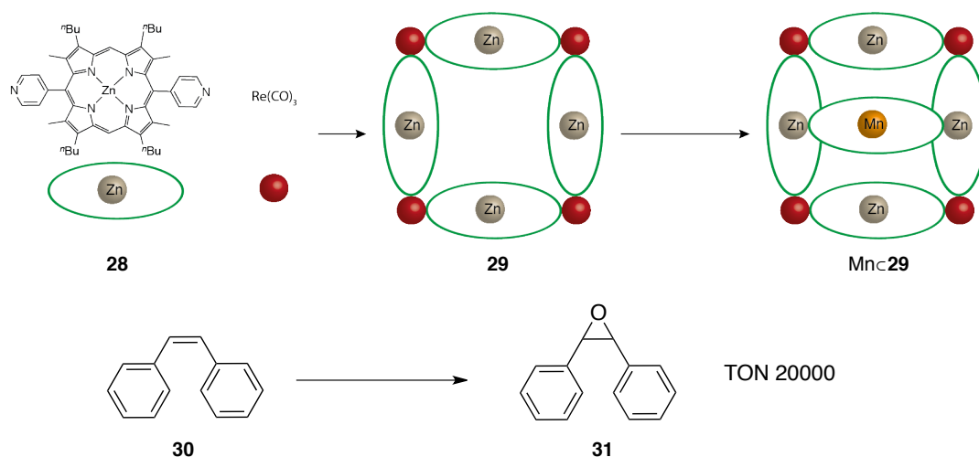
Scheme I-19: Schematic synthesis of the formation of the Mn c 29 and catalytic application.
