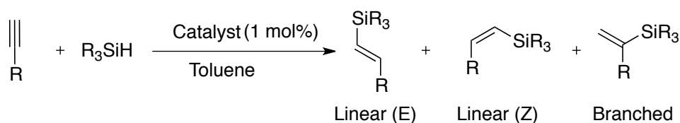
Scheme IV-10: Generic Pt(0) catalyzed hydrosilylation of alkynes
