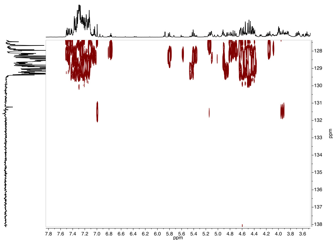
Figure S41: HMBC of ( \gamma -ICyD)Au 2 Cl 163 showing the cross correlations with the C=Au. (Acetone-d 6 , 300 K)
