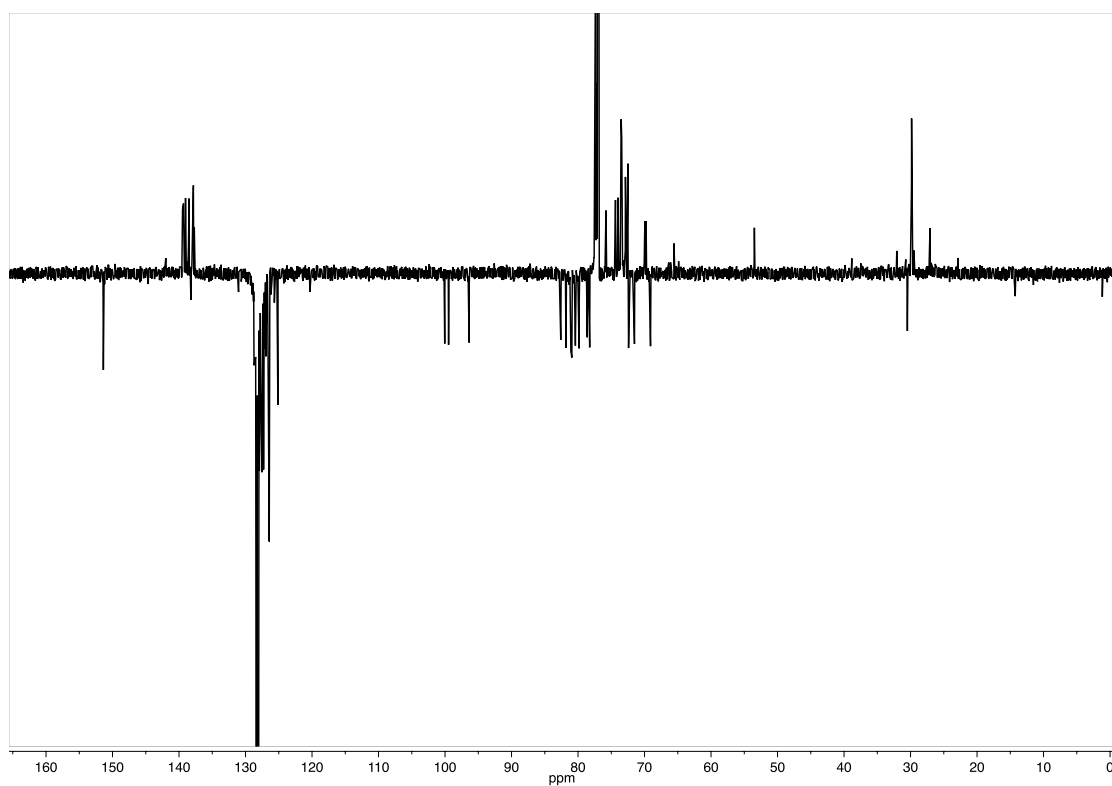
Figure S70: ^{13}\text{C-Jmod} of (\alpha\text{-rev-ICyD})\text{PtCl}_2(\text{pyridine}) 180 ( \text{CDCl}_3 , 151 MHz, 300 K)
