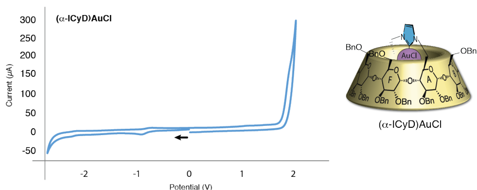
Figure III-31: Cyclic voltammogram of (\alpha\text{-ICyD})\text{AuCl} complex. MeCN, 0.5 V/s, [(\text{ICyD})\text{AuCl}] = 2\text{ mM} , 0.1M \text{TBAPF}_6 as supporting electrolyte.
