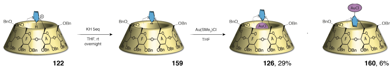
Scheme III-6 : Formation of the free \alpha -ICyD and metalation with \text{Au}(\text{Me}_2\text{S})\text{Cl} affording a mixture of (\alpha\text{-ICyD})\text{AuCl} and (\alpha\text{-rev-ICyD})\text{AuCl}
