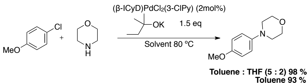
Scheme IV-29: Optimization of solvent for the (\beta\text{-ICyD})\text{PdCl}_2(3\text{-CIPy}) catalyzed Buchwald-Hartwig amination.
