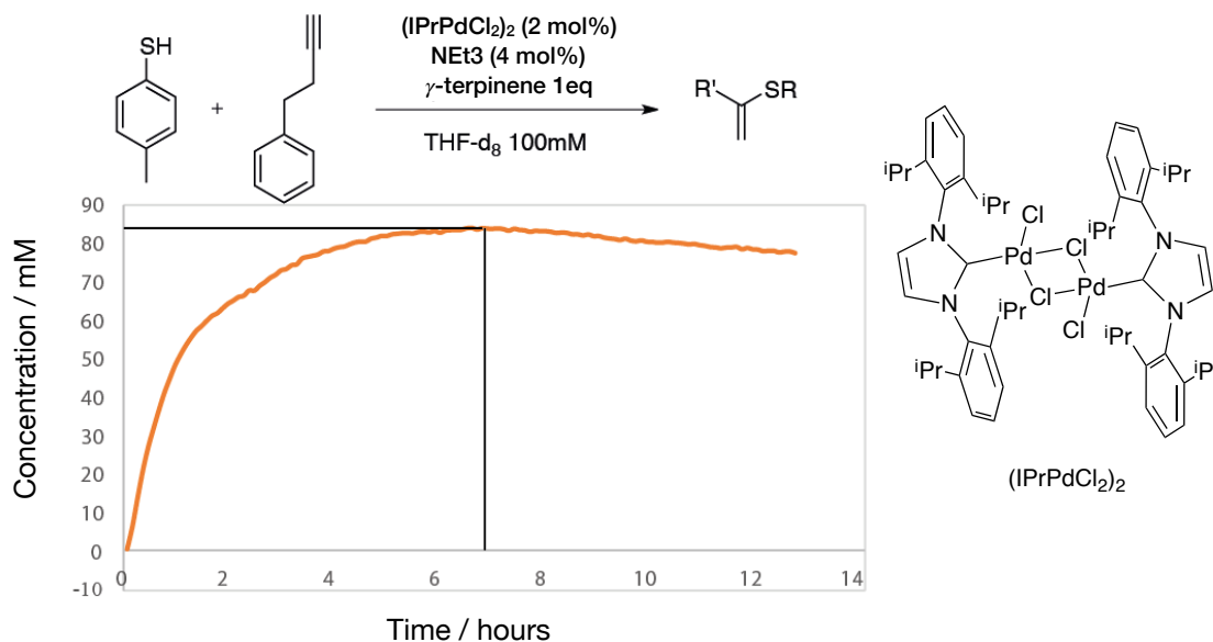
Figure IV-5 : Kinetic profile of the (\text{IPrPdCl}_2)_2 catalyzed hydrothiolation.
