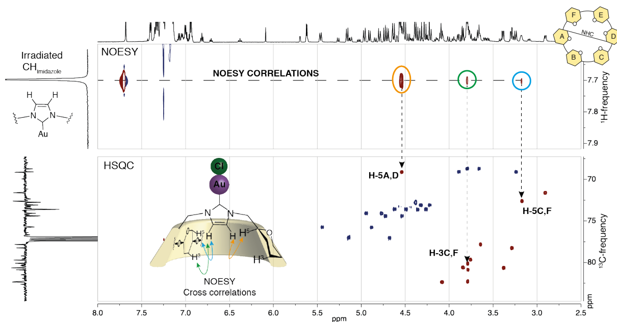
Figure III-11: Extract of NOESY experience of (\alpha\text{-rev-ICyD})\text{AuCl} stacked with the HSQC showing NOE correlations between the CH of the NHC and the intra cavity protons H3 and H5. \text{CDCl}_3 , 600 MHz, 300K
