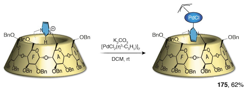
Scheme III-21: Synthesis of (α-rev-ICyD)PdCl(η 3 -allyl)
