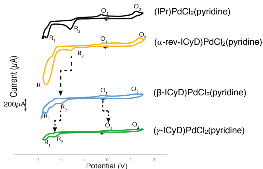
Figure III-65: Stacked cyclic voltammogram of the studied complexes. [(NHC)Pd] = 2 mM, [( \gamma -ICyD)PdCl 2 ] = 1.5 mM, TBABF 4 0.1 M, GC 3 mm, CE Pt wire, SCE, 20°C, 0.5 V/s.
