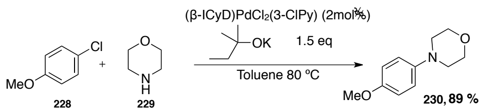
Scheme IV-30: Final conditions for the (\beta\text{-ICyD})\text{PdCl}_2(3\text{-CIPy}) reaction
