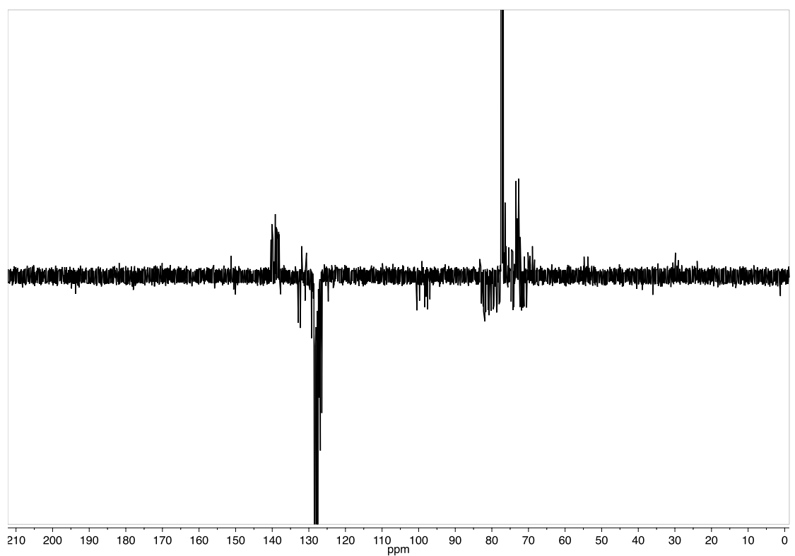
Figure S101: ^{13}\text{C-Jmod} of 227 ( \text{CDCl}_3 , 151 MHz, 300 K)
