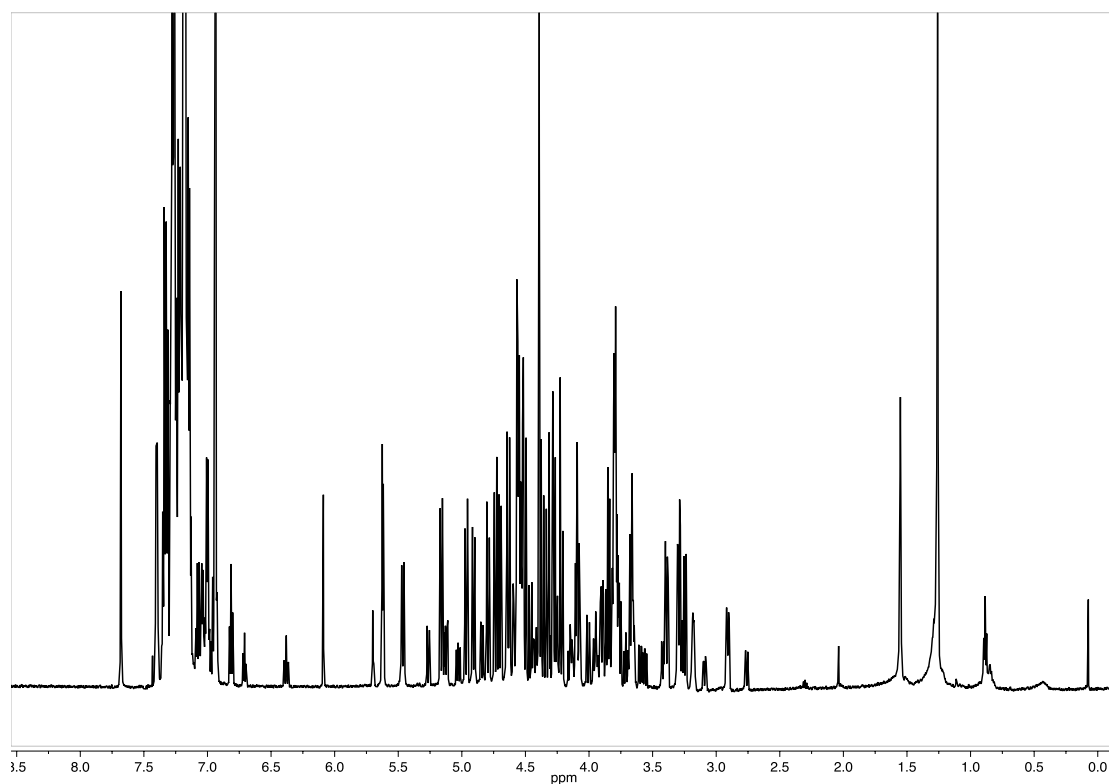
Figure S28: ^1\text{H} -NMR of the 77:23 mixture of 160:127 ( \text{CDCl}_3 , 600 MHz, 300 K)
