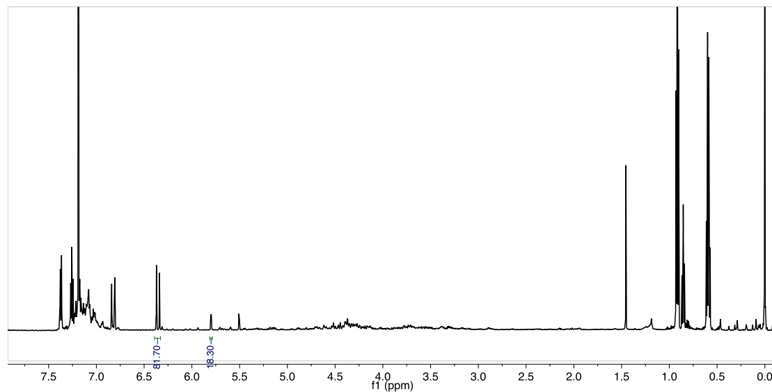
Figure S110: Crude 1 H-NMR of the reaction with ( \beta -ICyD)Pt(dvtms)(CDCl 3 , 600MHz, 300K)
