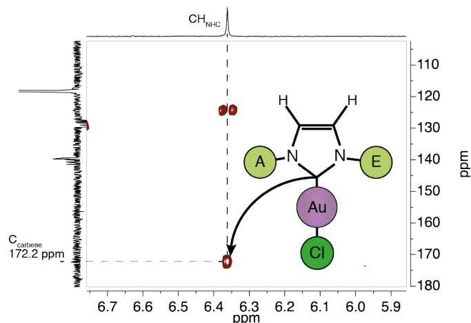
FIGURE III-1 : HMBC of ( \gamma -ICyD)AuCl 157 showing the chemical shift of the C_{\text{carbene}} . \text{CD}_3\text{CN} , 400 MHz, 300 K
