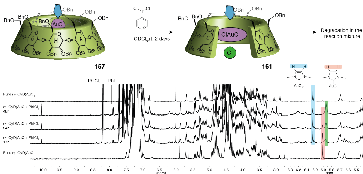
Figure III-21 : NMR monitoring of the reaction of (\gamma\text{-ICyD})\text{AuCl} with \text{PhICl}_2 . Zoom of the \text{CH}_{\text{NHC}} and anomeric region is shown on the right.
