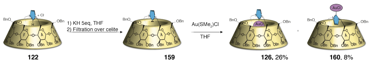
Scheme III-5: Reaction conditions of the formation of the free NHC and metallation with Au(SMe 2 )Cl
