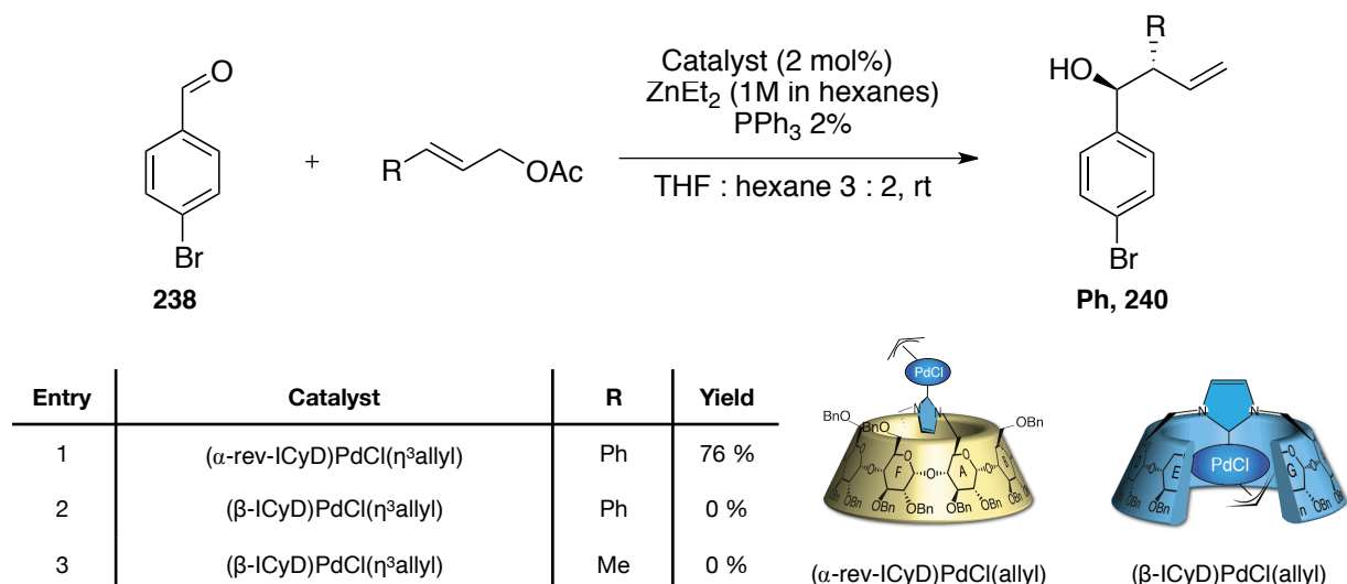
Scheme IV-38: (ICyD)PdCl(allyl) catalyzed allylation of 4-bromobenzene.
