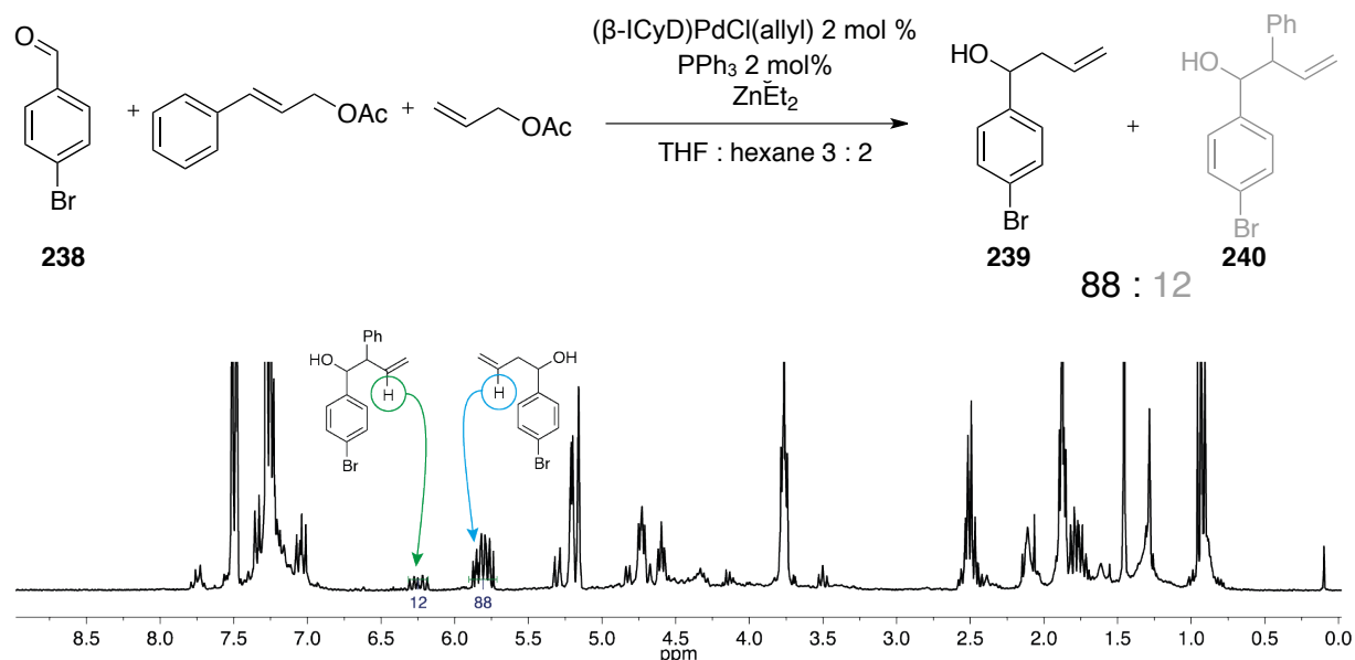
Figure IV-40: Reaction conditions for the substrate selection with (\beta\text{-ICyD})\text{PdCl}(\eta^3\text{-allyl})
