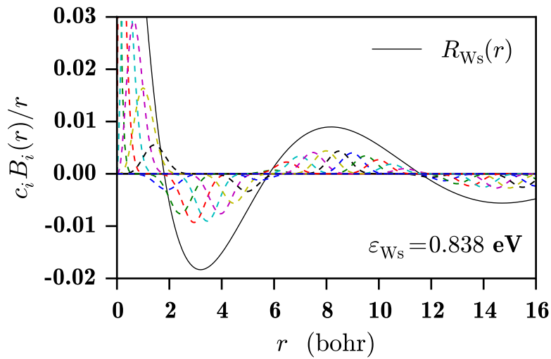
Figure 3.11: Weighted B-spline decomposition of a given continuum radial wave function of symmetry “s”. B-spline parameters: N = 400 , k = 8 , r_{\max} = 200 bohr and linear sequence of breakpoints.
