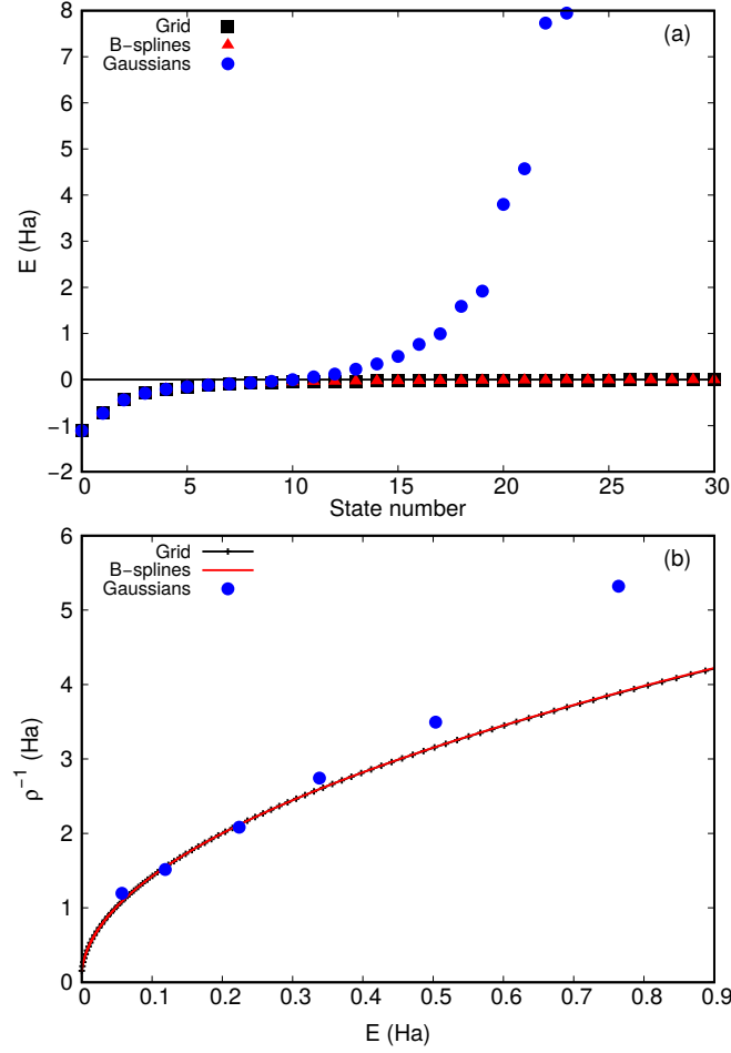
Figure 5.2: (a) Eigenvalues of H_2^+ up to the 30th eigenstate. (b) Inverse of the normalized density of continuum states.
