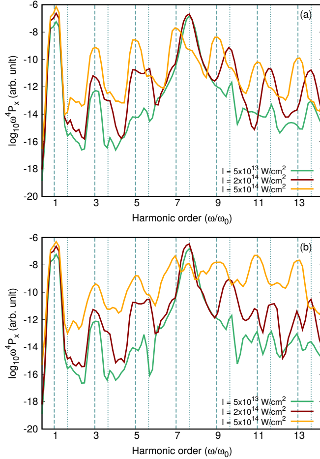
Figure 5.12: HHG spectra in the dipole form at the equilibrium internuclear distance of R = 2.0 au up to the 13th harmonic with laser intensities : I = 5 \times 10^{13} W/cm 2 , I = 2 \times 10^{14} W/cm 2 , and I = 5 \times 10^{14} W/cm 2 for (a) grid and (b) Gaussian basis sets. For each HHG spectrum, the dashed line indicates the position of the harmonics and the dotted line indicates the hyper-Raman lines at position \tilde{\omega} \pm 2k\omega_0 [Gauthey 95] where k is an integer and \tilde{\omega} = 7.65\omega_0 is the resonance of the first excited state.
