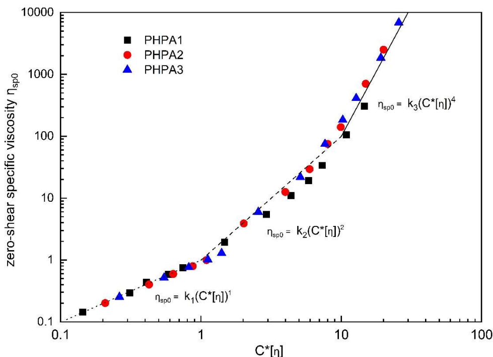
Figure 2.17 : The master curve of zero-shear specific viscosity versus the overlap parameter for the three PHPAs prepared in 5 g/l NaCl water and at 25°C.
