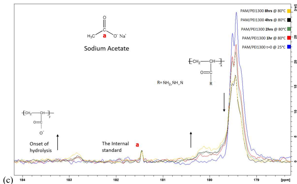
Figure 5.8 : (a) Proton “ ^1\text{H} ” and (b-c) Carbon “ ^{13}\text{C} ” NMR spectra of PAM/PEI1300 mixture cured at 80 °C for different reaction times.
