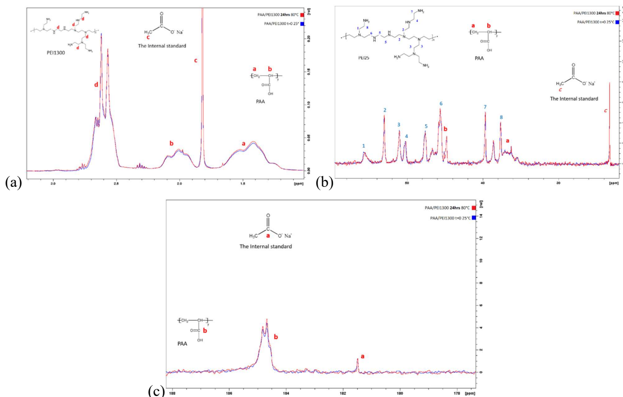
Figure 5.7 : (a) Proton “ ^1\text{H} ” and (b-c) Carbon “ ^{13}\text{C} ” NMR spectra of PAA/PEI1300 mixture recorded at t=0 ( 25^\circ\text{C} ) and at 24 hours (after curing at 80^\circ\text{C} ).
