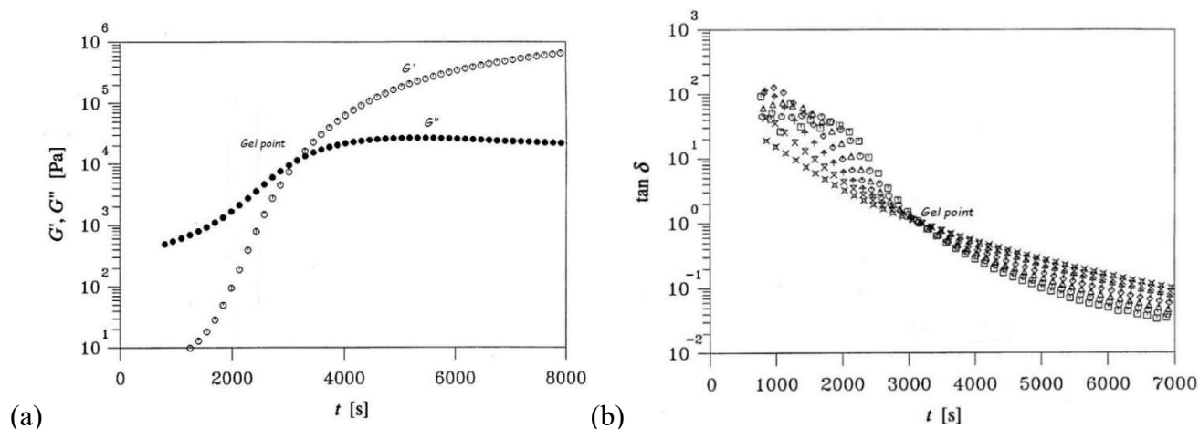
Figure 1.35 : Gelation time determination as defined by (a) Tung and Dynes, (b) Winter and Mours.[176].
