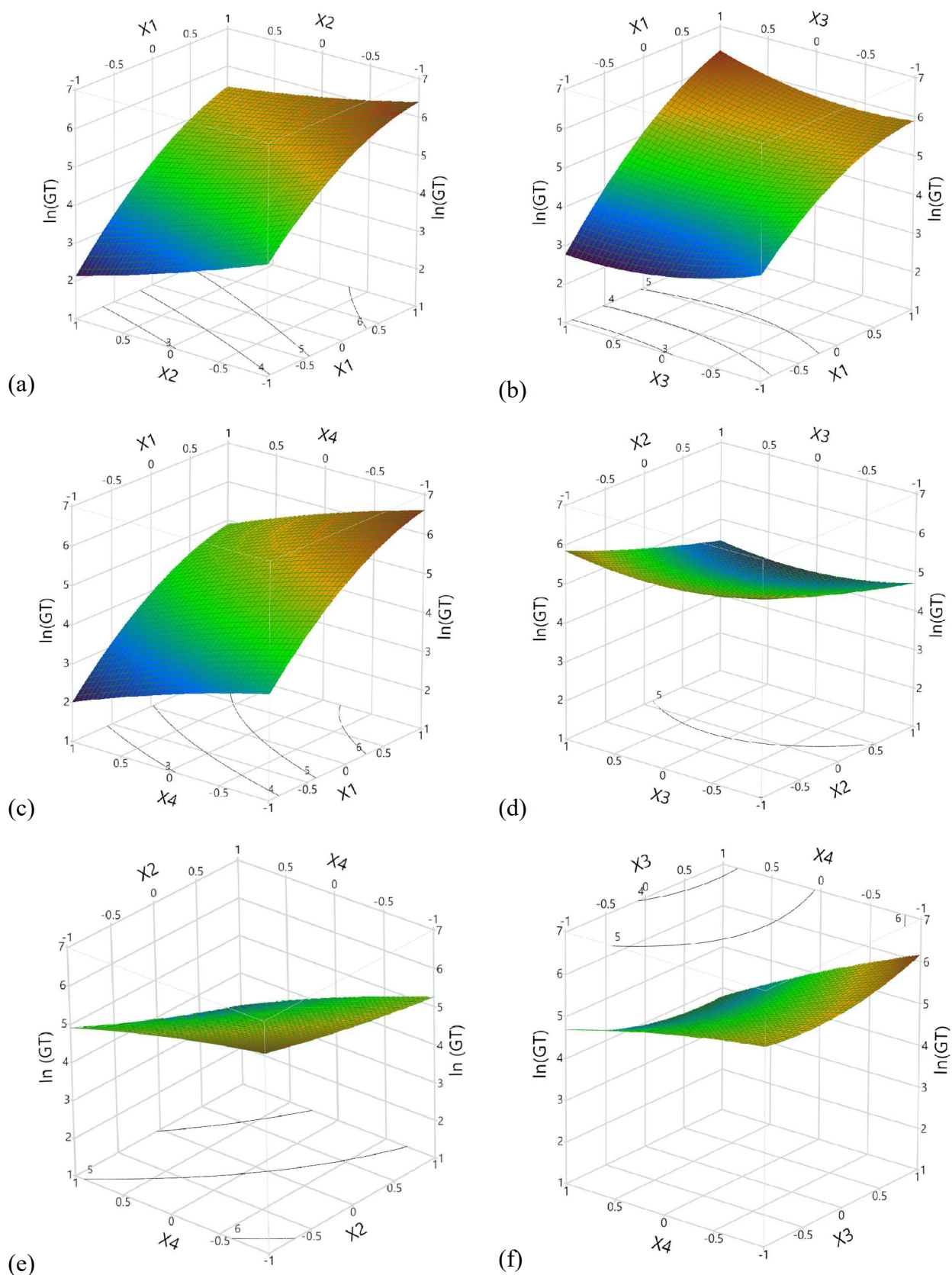
Figure 4.8 : 3D response surface plots of \ln(GT) showing combined effect of NaCl concentration " X_1 ", polymer concentration " X_2 ", crosslinker concentration " X_3 " and Temperature " X_4 ".
