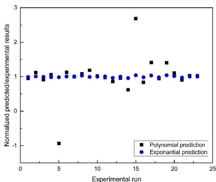
Figure 4.6 : normalized predicted/experimental results for each experimental run using the polynomial and the exponential models.
