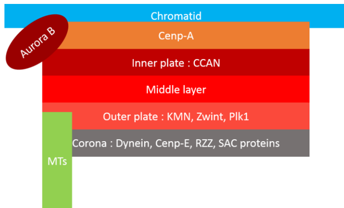
Figure 7 : Kinetochore structure
