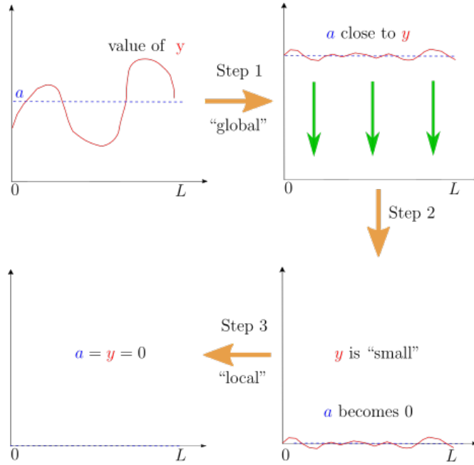
Figure 1.1: Small-time global stabilization by steps.
