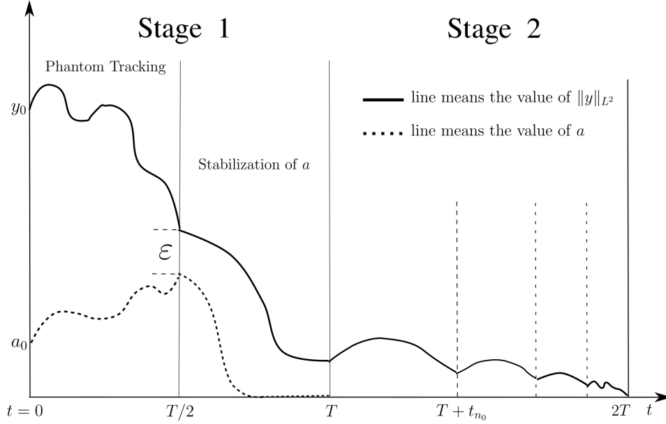
Figure 5.1: Small-time global stabilization of (y, a) .
