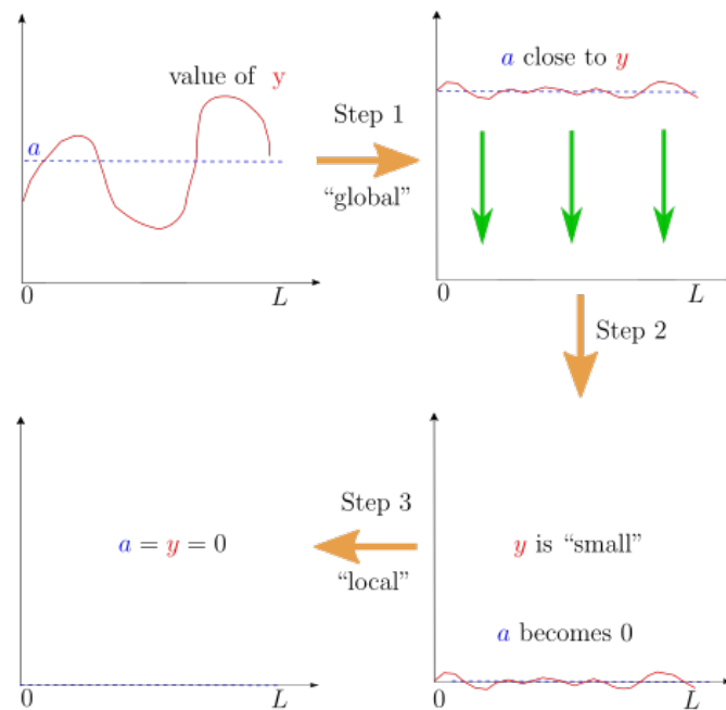
Figure 1.1: Small-time global stabilization by steps.
