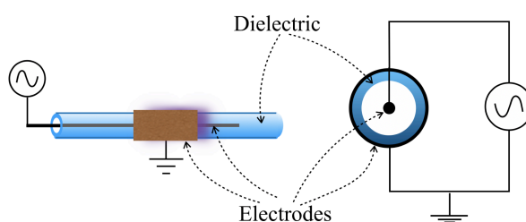
Figure II-3 Scheme of the DBD reactor used in this study.
