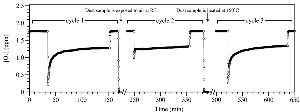
Figure III-7 Profiles of gas phase ozone concentration monitored along cyclic experiments of uptake onto 90 \pm 1 mg of Gobi dust ( [O_3]_0 = 1.7 \pm 0.1 ppm, dry air, T = 296 K, P = 1013 mbar).
