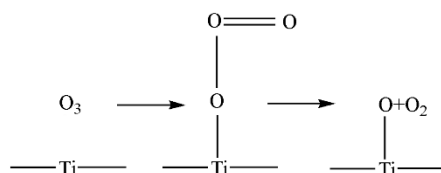
Figure I-10 Schematic diagram to illustrate the mechanism of ozone decomposition on the surface of \text{TiO}_2 adapted from the work of K. M. Bulanin et al. [143].
