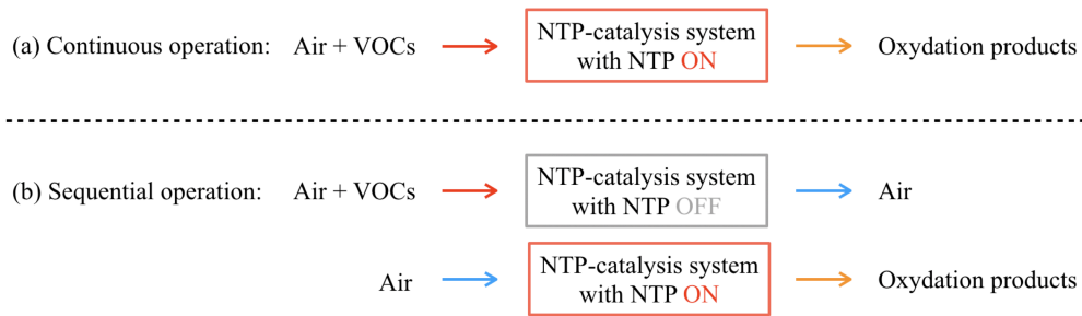
Figure I-29 Schematic of (a) continuous operation and (b) sequential operation of plasma-catalysis for VOC abatement.
