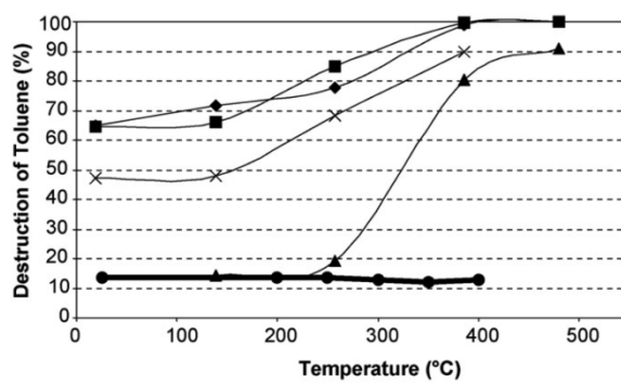
Figure I-25 Comparison of catalyst performance for the plasma-catalytic destruction of toluene at varying temperatures, using ( \blacklozenge ) \gamma\text{-Al}_2\text{O}_3 , ( \blacksquare ) \text{Ag}/\gamma\text{-Al}_2\text{O}_3 , ( \blacktriangle ) \text{TiO}_2 and ( \times ) \text{Ag/TiO}_2 catalysts and supports, in a one-stage configuration. The thick black line shows plasma alone results, with no catalyst. (The figure is retrieved directly from A. M. Harling et al. [184].)
