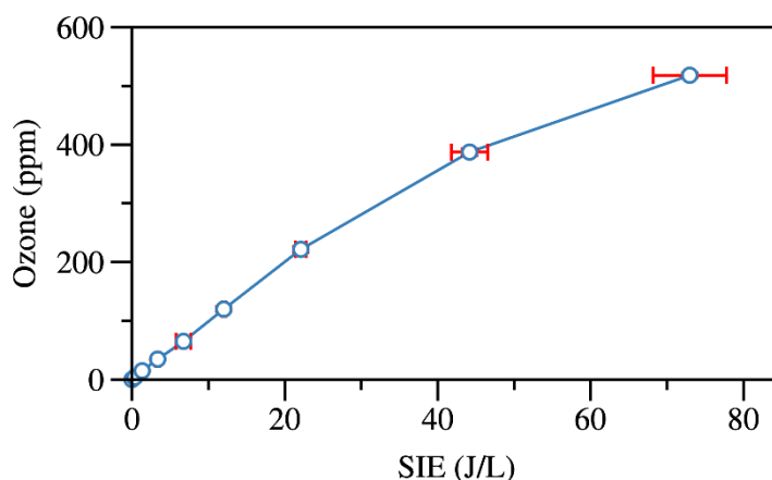
Figure II-4 Ozone production as a function of the SIE for the DBD reactor used in this study.
