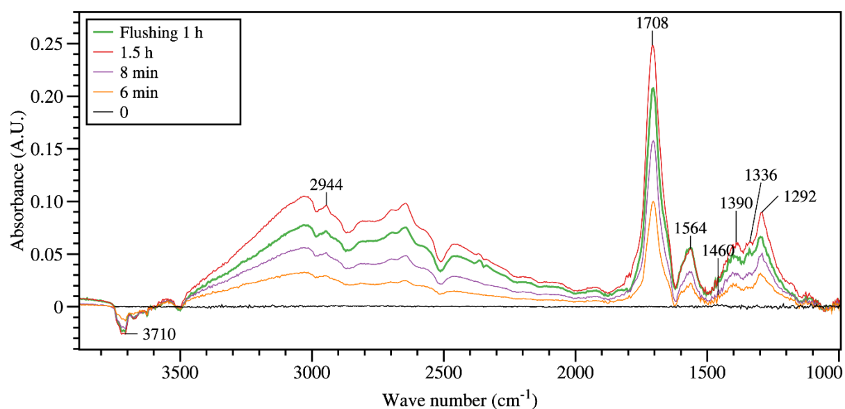
Figure IV-10 Chronological DRIFT spectra of the surface of Gobi dust during the exposure to AcA and after flushing by zero air flow for 1 hour ( [\text{AcA}] = 10 \pm 0.5 \text{ ppm} , dry condition, T = 296 \text{ K} , P = 1013 \text{ mbar} ).
