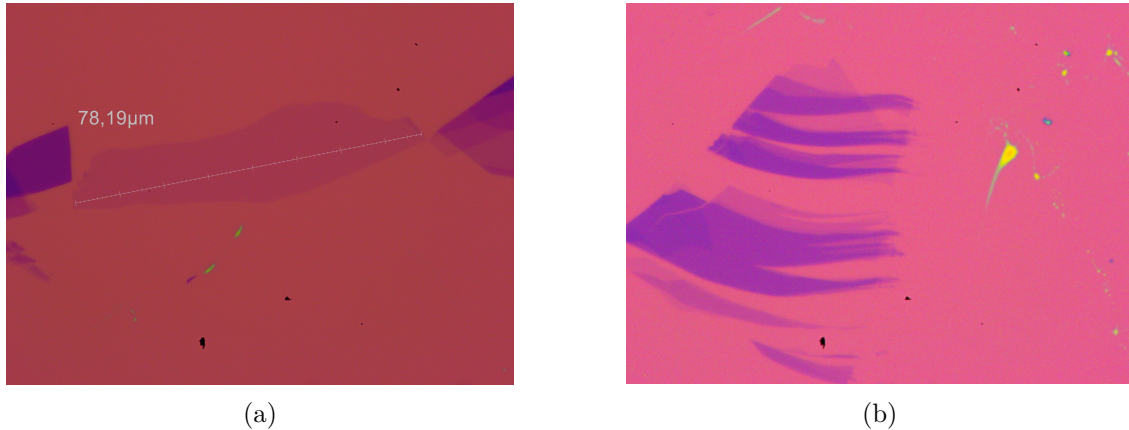
Figure 1.11: Optical microscope observations of my exfoliation of graphene monolayer, and few layers graphite deposited on silicium chip with a 300\text{nm} thick \text{SiO}_2 oxyde. (a) Big monolayer graphene flake. (b) Crystal with graphene (light purple), bi-layer, and few layers graphite. The darker the more layer there are.
