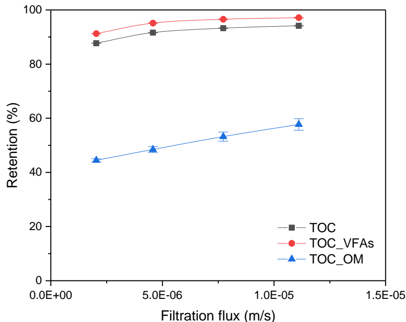
Figure VI-10 The retentions of the TOC of real fermentation broth (TOC all ), the TOC of the three VFAs (TOC VFAs ), and the TOC of the organic matters/impurities (TOC OM ) using XLE membrane at pH 5.7.
