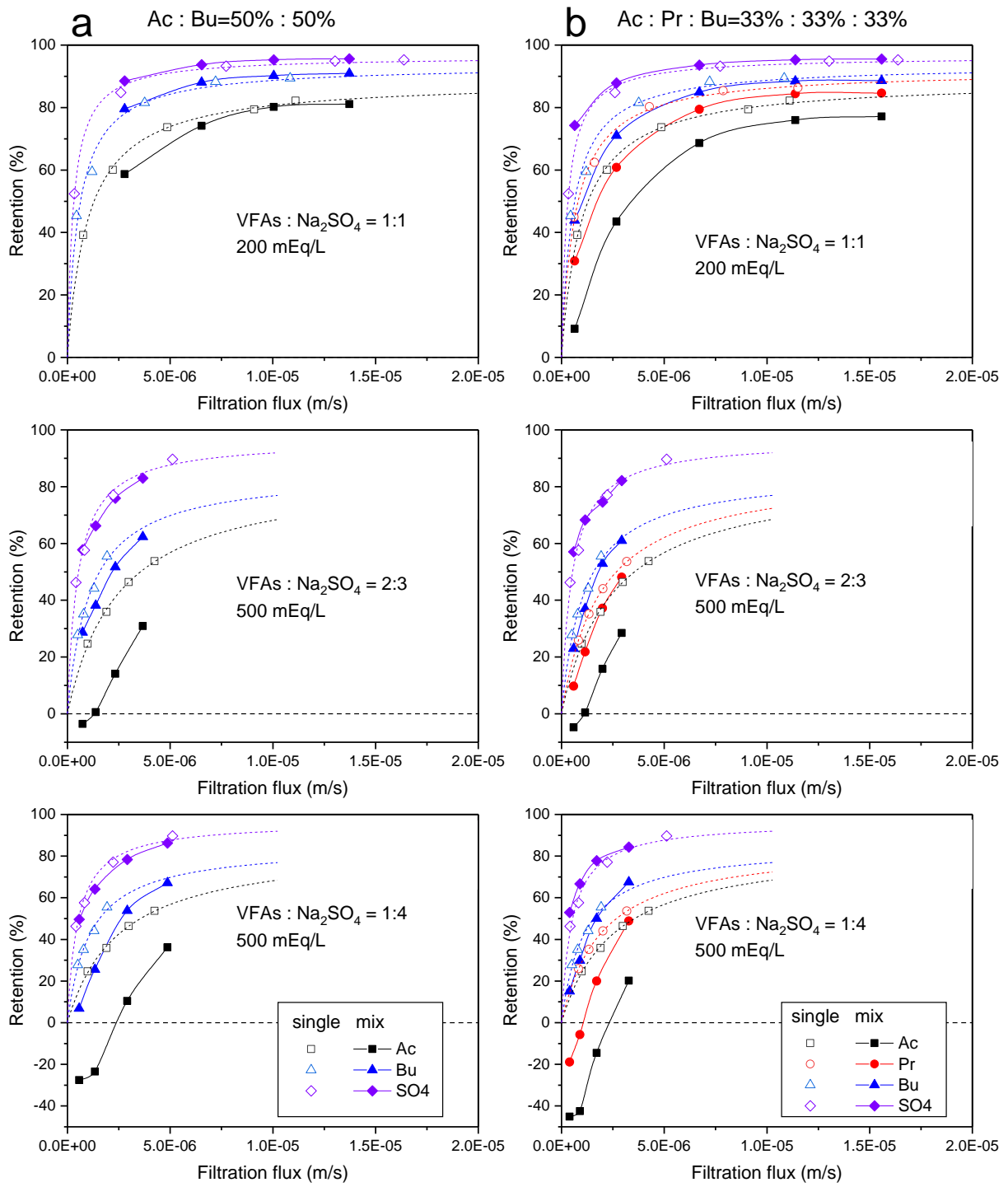
Figure IV-3 Retention of individual anions at different compositions: (a) Ac/Bu binary solution with Na 2 SO 4 , (b) Ac/Pr/Bu ternary solution with Na 2 SO 4 , using NF-45 membrane.
