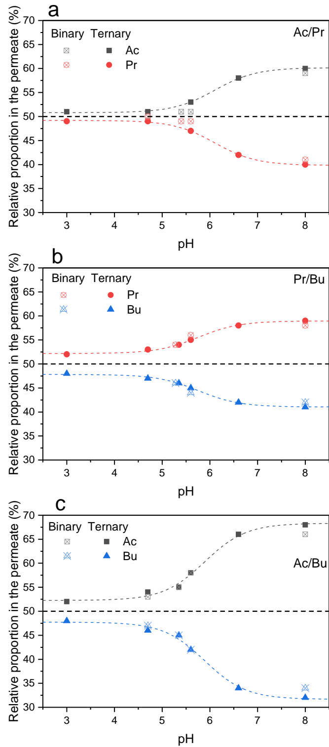
Figure V-13 Relative proportions of Ac, Pr, and Bu for the couples of (a) Ac/Pr, (b) Pr/Bu and (c) Ac/Bu, in the permeate versus solution pH in the binary (Ac:Pr=50%:50%, Pr:Bu=50%:50%, Ac:Bu=50%:50%) and ternary (Ac:Pr:Bu =33%:33%:33%) solutions, using NF-45 membrane.
