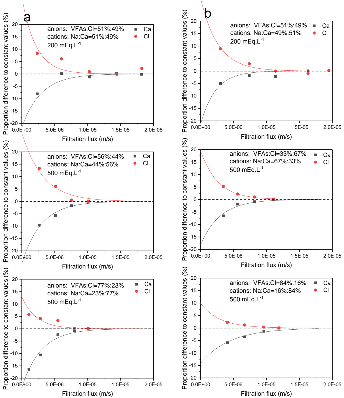
Figure IV-12 The difference of the permeate proportion to the constant values (proportion difference = P_i^{P^*} - P_i^P ) for \text{Ca}^{2+} and \text{Cl}^- in (a) Ac/Bu binary solution with \text{CaCl}_2 , (b) Ac/Pr/Bu ternary solution with \text{CaCl}_2 , using NF-45 membrane, at pH 8.
