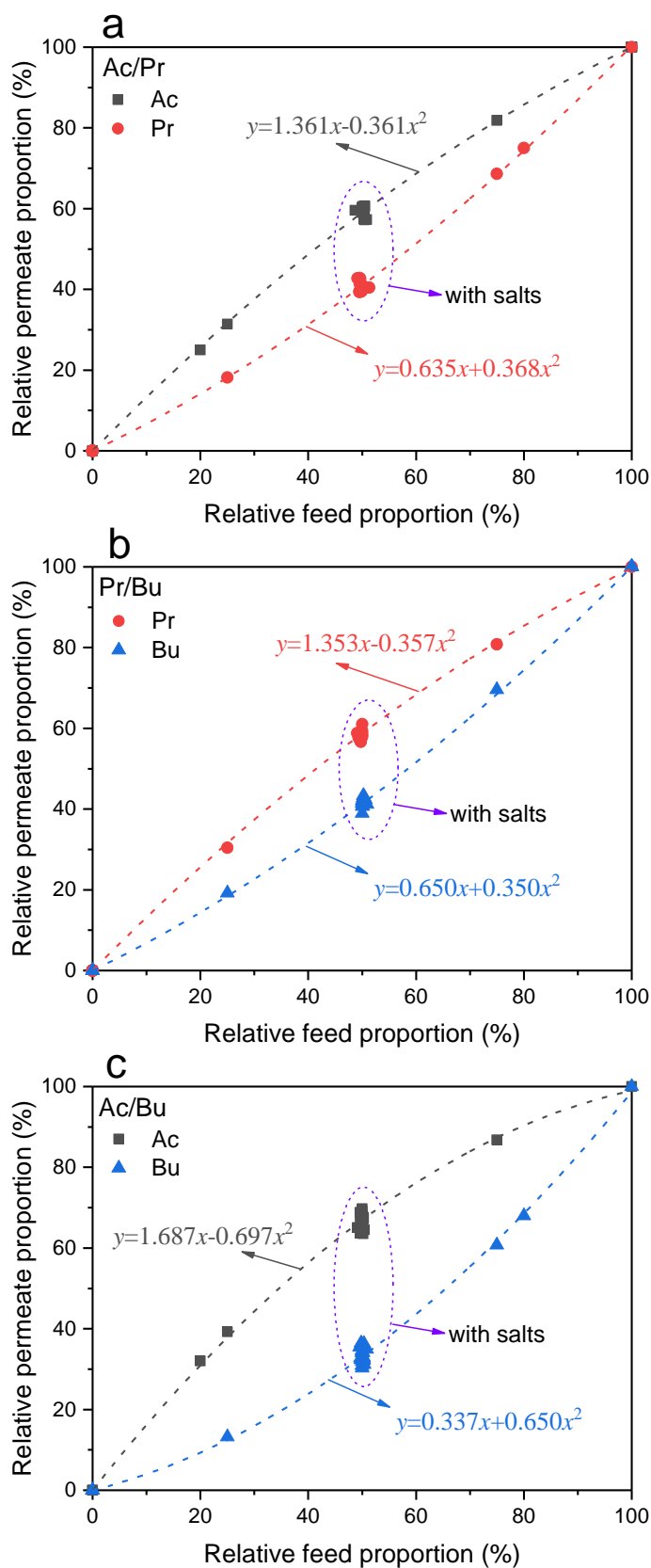
Figure IV-14 Relative proportions of VFAs in the couples of (a) Ac/Pr, (b) Pr/Bu, and (c) Ac/Bu, for all the compositions investigated, using NF-45 membrane at pH 8.
