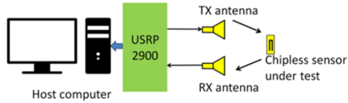
Figure 6.31: Schematic diagram of the experimental setup for the sensing system
