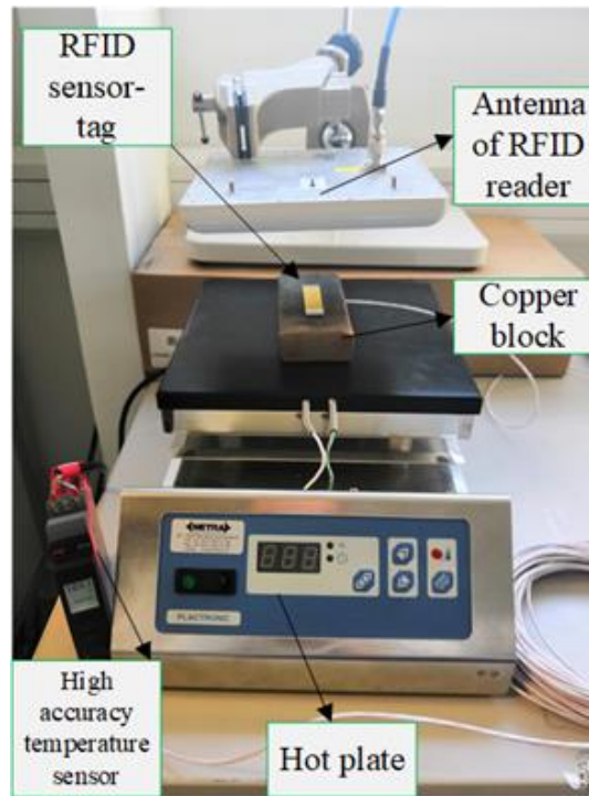
Figure 5.12: Experimental setup for temperature measurement
