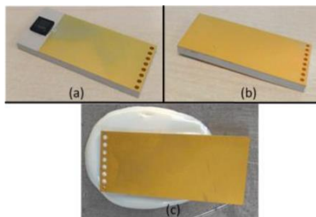
Figure 7.15: Fabricated RFID sensor tag (a) bottom view (b) top view (c) placement with the glue
