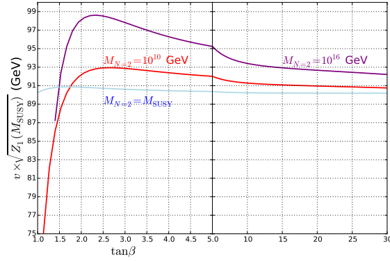
Figure 2.2: v \times \sqrt{Z_1(M_{\text{SUSY}})} against \tan\beta for M_{N=2} = M_{\text{SUSY}}, 10^{10} GeV and 10^{16} GeV, which corresponds to the “tree-level” value of the Higgs mass before running from M_{\text{SUSY}} is taken (or equivalently the SUSY corrections at M_Z ) into account (we take v = 246 GeV in the figure). One sees that increasing M_{N=2} increases the Higgs mass, particularly for small \tan\beta > 1.5 .
