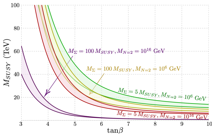
Figure 2.13: M_{SUSY} against \tan\beta for a Higgs mass of 125 GeV at m_t and where Q = 600 GeV, plotted for values of M_\Sigma = 5, 100 M_{SUSY} and M_{N=2} = 10^6 and 10^{16} GeV.
