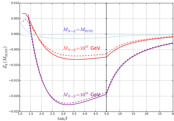
Figure 2.3: Z_6(M_{\text{SUSY}}) against \tan\beta for M_{N=2} = M_{\text{SUSY}}, 10^{10} GeV and 10^{16} GeV, which corresponds to just the contributions to Z_6 from the running of \lambda_{S,T} and the threshold corrections. The solid lines show the full value of Z_6 , while the dashed lines are just those given by equation (2.4.3), i.e. without threshold corrections.
