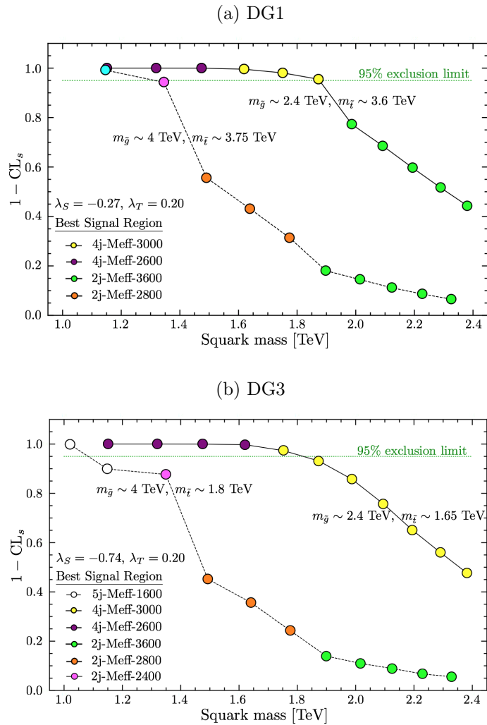
Figure 3.8: 1-\text{CL}_s values in the best signal regions from all proton-proton processes as a function of squark mass for (a) DG1 and (b) DG3. The solid lines are for m_{\tilde{g}} \sim 2.4 TeV, while the dashed lines are for m_{\tilde{g}} \sim 4 TeV. (Since the input parameters are the soft masses, m_{\tilde{t}} and m_{\tilde{b}} vary slightly in the two cases.)
