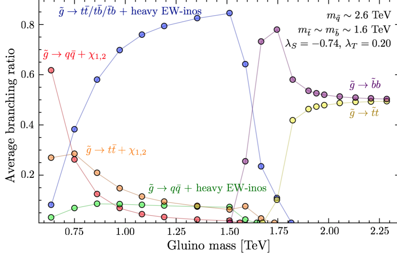
Figure 3.3: Branching ratios of gluino decays (averaged over \tilde{g}_1 and \tilde{g}_2 ) for DG3 as function of the gluino mass, for m_{\tilde{q}} \approx 2.6 TeV.
