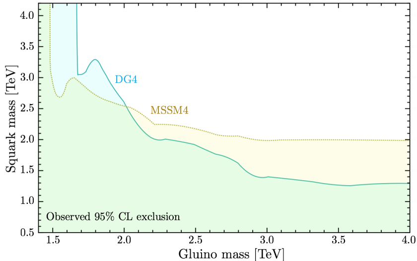
Figure 3.9: 95% CL exclusion limits in the gluino vs. squark mass plane for DG4, and comparison to MSSM4.
