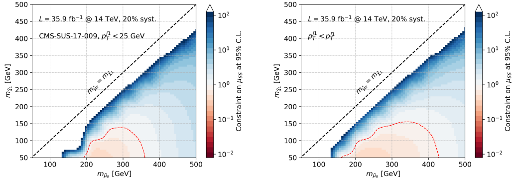
Figure 4.4: Exclusion contours on the signal strength \mu_{SS} for smuon pair production in the (m_{\tilde{\chi}_1}, m_{\tilde{\mu}_R}) plane with \mathcal{L} = 35.9 \text{ fb}^{-1} , for (a) the static jet veto analysis based on ref. [219], with p_T^{\text{Veto}} = 25 \text{ GeV} , and (b) the dynamic jet veto analysis with p_T^{\text{Veto}} = p_T^{\ell_1} .
