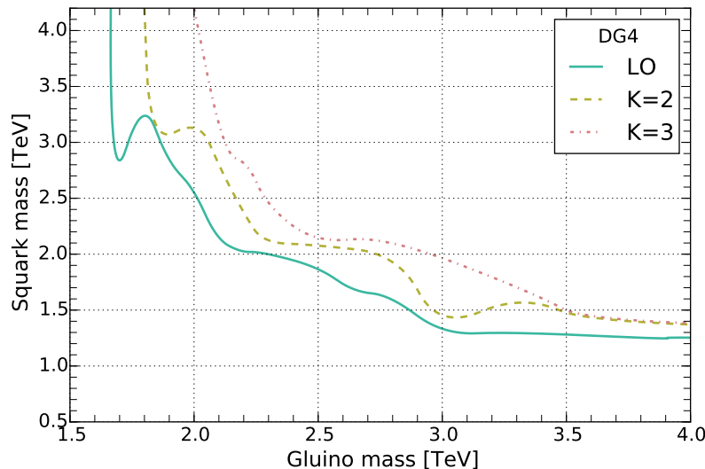
Figure 3.10: 95% CL exclusion limits in the gluino vs. squark mass plane for benchmark DG4 with K-factors 1 (LO), 2 and 3.
