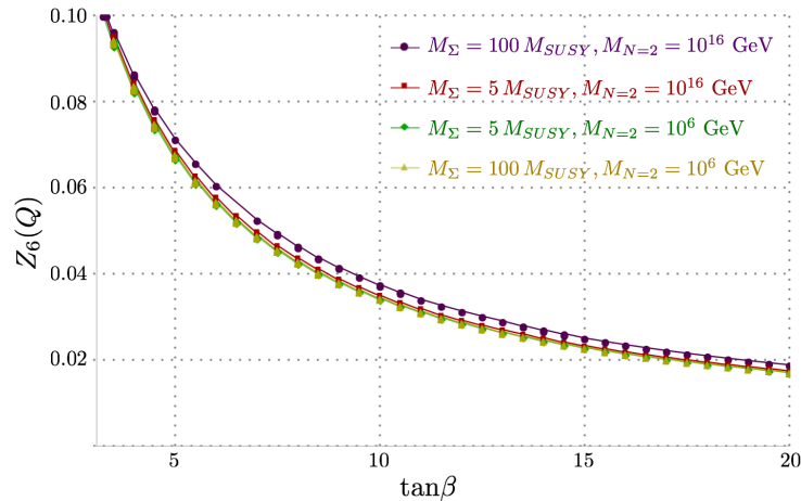
Figure 2.12: Z_6(Q) against \tan\beta for a Higgs mass of 125 GeV at m_t , for values of M_\Sigma = 5, 100 M_{SUSY} and M_{N=2} = 10^6 and 10^{16} GeV.
