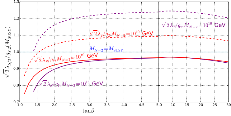
Figure 2.1: Variation of the ratios \sqrt{2}\lambda_S/g_Y and \sqrt{2}\lambda_T/g_2 at the scale M_{\text{SUSY}} with \tan\beta , for M_{N=2} = M_{\text{SUSY}}, 10^{10} GeV and 10^{16} GeV.
