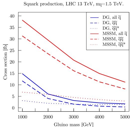
Figure 3.1: Squark production cross-sections at leading order (LO) for the 13 TeV LHC as a function of the gluino mass in the MSSM (in red) and in the DG case (in blue), for m_{\tilde{q}} = 1.5 TeV, assuming an 8-fold squark degeneracy ( \tilde{q} = \tilde{u}, \tilde{d}, \tilde{c}, \tilde{s} ). The dashed, dotted and full lines show the squark-squark, squark-antisquark and total squark production cross-sections, respectively.
