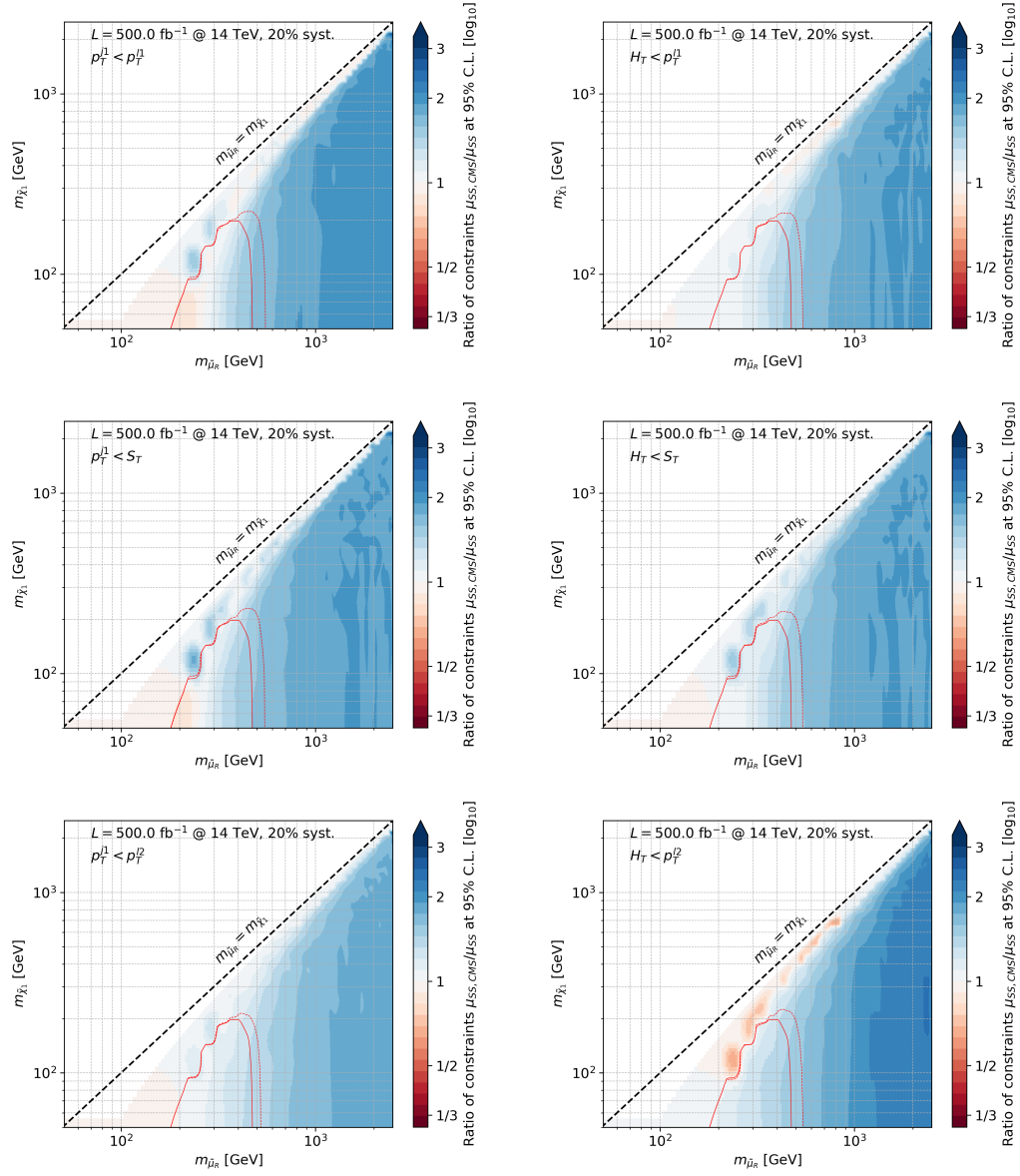
Figure 4.5: The ratio of signal strengths ( \mu_{SS} ) for (a) p_T^{\text{Veto}} = p_T^{\ell_1} , (b) H_T^{\text{Veto}} = p_T^{\ell_1} , (c) p_T^{\text{Veto}} = S_T , (d) H_T^{\text{Veto}} = S_T , (e) p_T^{\text{Veto}} = p_T^{\ell_2} , and (f) H_T^{\text{Veto}} = p_T^{\ell_2} , compared with the CMS reference analysis using \mathcal{L} = 500 \text{ fb}^{-1} . The solid red line shows the 95% exclusion for \mu_{SS} = 1 for the benchmark CMS analysis, and the dashed red line the same exclusion for the dynamic analysis.
