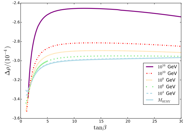
Figure 2.7: \Delta\rho calculated at one-loop in the low-energy theory, for different values of M_{N=2} given in the legend. One sees that the magnitude is roughly equal to the experimental error, and the model value is always well within 3\sigma of the experimental central value (which is anyway above the Standard Model value by 1.6\sigma ).
