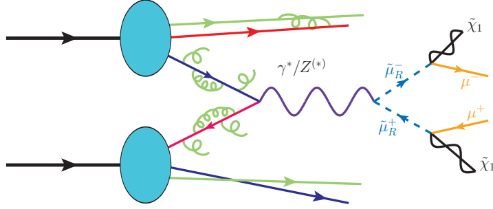
Figure 4.1: Drell-Yan production of a pair of right-handed smuons ( \tilde{\mu}_R^+\tilde{\mu}_R^- ) decaying into a pair of muons ( \mu^\pm ) and lightest neutralinos ( \tilde{\chi}_1 ). Generated with JAXODRAW [253].
