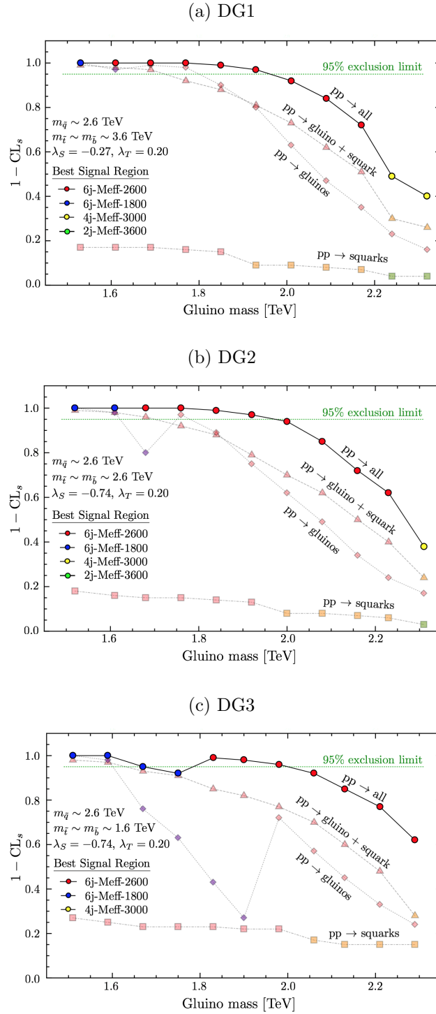
Figure 3.6: 1-\text{CL}_s values in the best signal regions from all proton-proton processes as a function of gluino mass for (a) DG1, (b) DG2, (c) DG3; m_{\tilde{q}} \sim 2.6 TeV in all three cases. Individual contributions to the total \text{CL}_s (denoted by the solid black line labelled pp \rightarrow \text{all} ) are given by the faint dashed lines, namely gluino-pair production (diamonds); squark-pair production (triangles) and gluino-squark production (squares). The best signal region at each gluino mass value is identified by the colour code as indicated in the plot legends.
