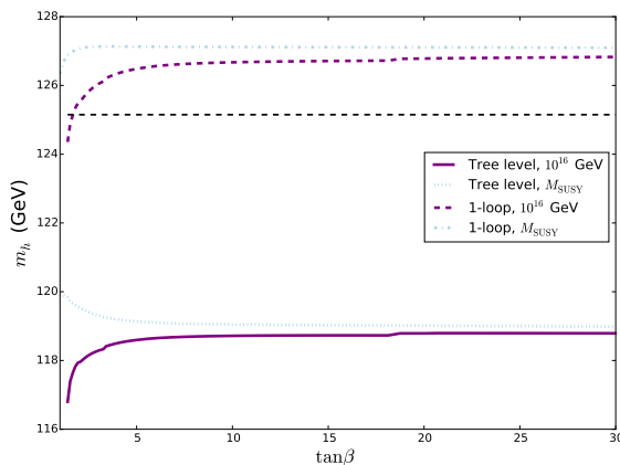
Figure 2.5: Effect of loop corrections in the low-energy theory on the Higgs mass. The tree-level and one-loop values for the Higgs mass are shown against \tan\beta for \mathcal{N} = 2 scales of the stop scale ( M_{\text{SUSY}} ) and 10^{16} GeV; the two-loop value of the Higgs mass is fixed to the black dotted line.
