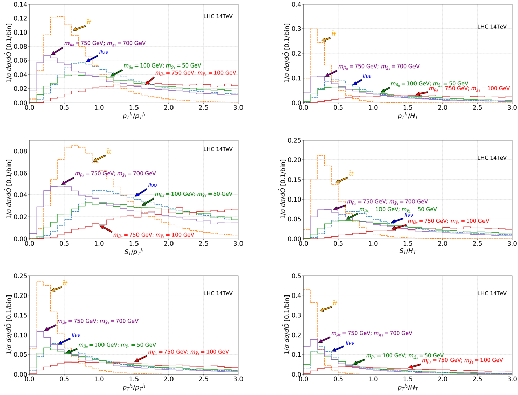
Figure 4.3: Ratios of measures of hadronic and leptonic activity for representative signal (solid) and background (dashed) samples used in the dynamic veto analysis, showing (a) p_T^{\ell_1}/p_T^{j_1} , (b) p_T^{\ell_1}/H_T , (c) S_T/p_T^{j_1} , (d) S_T/H_T , (e) p_T^{\ell_2}/p_T^{j_1} , (f) p_T^{\ell_2}/H_T .
