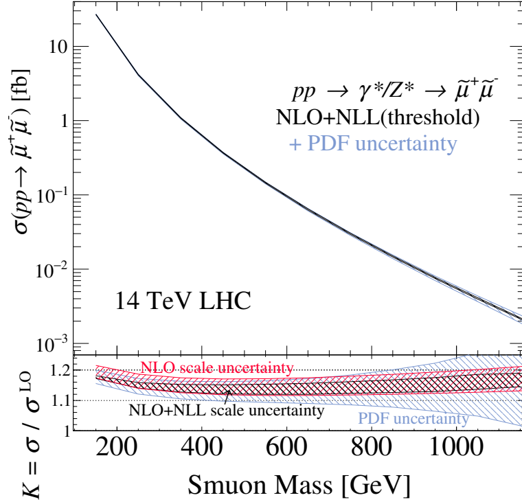
Figure 4.2: Upper: totally inclusive neutral-current DY production cross section of \tilde{\mu}_R^+ \tilde{\mu}_R^- pairs at NLO+NLL, and at a center-of-mass energy \sqrt{s} = 14\text{TeV} with scale uncertainty (black band) and PDF uncertainty (lightest band). Lower: NLO+NLL (black band) and NLO (lighter band) QCD K -factor, with PDF uncertainty (lightest band).
