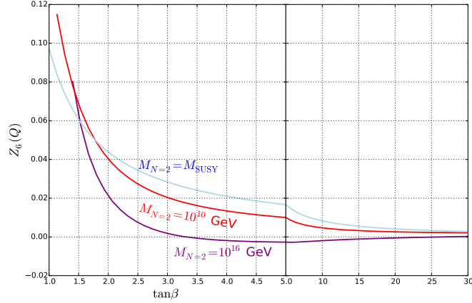
Figure 2.4: Z_6(Q) against \tan\beta , where Q = 400 GeV is our low-energy matching scale. One finds that the model shows good alignment for all values of \tan\beta > 1.5 , with the surprising conclusion that raising the \mathcal{N} = 2 scale improves the alignment.
