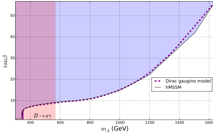
Figure 2.8: Bounds from pp \rightarrow H/A \rightarrow \tau^+\tau^- (blue region) and B \rightarrow s\gamma (red region, m_A \lesssim 568 GeV) interpreted in the m_A/\tan\beta plane for the hMSSM (taken from [177]) and our model.
