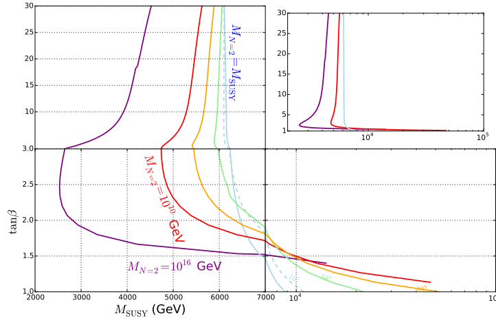
Figure 2.6: SUSY scale that fits m_h = 125.2 GeV against \tan\beta . The cases M_{N=2} = \{M_{\text{SUSY}}, 10^{10} \text{ GeV}, 10^{16} \text{ GeV}\} are the solid lines in blue, red and purple respectively and are labelled in full; the cases M_{N=2} = \{10^4, 10^6, 10^8\} GeV are respectively shown in blue dashed, solid green and solid orange curves and only labelled with \{10^4, 10^6, 10^8\} . Due to the large range of scales M_{\text{SUSY}} values for small \tan\beta and the little change for large \tan\beta the plot has been split into three quadrants to show the values more clearly, but for comparison an inset graph is given showing the three curves M_{N=2} = \{M_{\text{SUSY}}, 10^{10} \text{ GeV}, 10^{16} \text{ GeV}\} with M_{\text{SUSY}} (GeV) on a logarithmic scale on the abscissa and \tan\beta on a linear scale on the ordinate.
