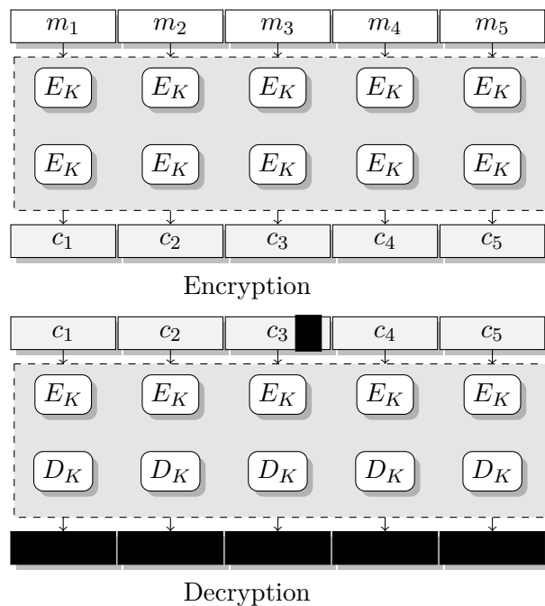
Figure 2.8: Malleability attack on WBTC using a blockcipher (E_K, D_k) where D_k = E_k^- . Bit flipping ("X") in the i -th ciphertext block affects all the plaintext (black blockq) after decryption.
