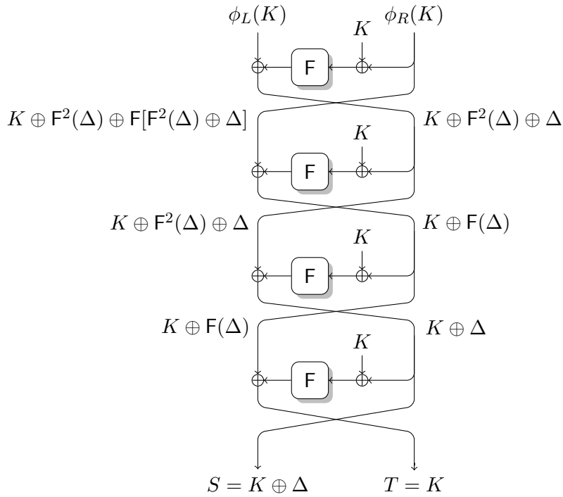
Figure 4.17: Details of the Sliding attack on 4-round KAF (same keys and same round function).
