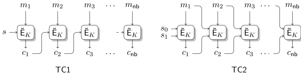
Figure 3.5: Description of the TC1 and TC2 modes of operations where \tilde{E} is a tweakable blockcipher. In FDE context, the tweak can be the sector number s (for TC2, s_0 || s_1 = P(s) where P is a permutation).
