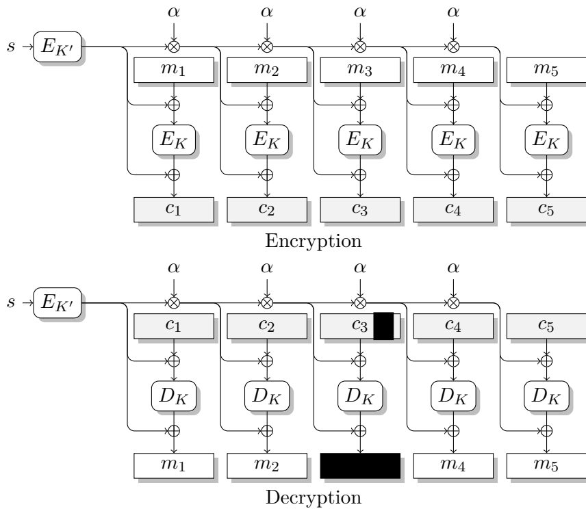
Figure 2.7: Malleability attack on XTS (here without ciphertext stealing) using a blockcipher (E_K, D_k) where D_k = E_k^- . Bit flipping ("X") in the i -th ciphertext block affects the i -th plaintext block (black block) after decryption.
