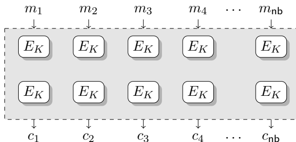
Figure 3.8: WTBC where E_K is either a blockcipher or a tweakable blockcipher. WTBC can use several calls to E_K to process one message block.
