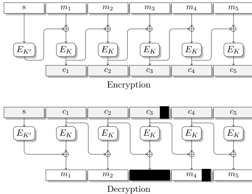
Figure 2.6: Malleability attack on CBC-ESSIV using a blockcipher (E_K, D_k) where D_k = E_k^- . Bit flipping ("X") in the i -th ciphertext block affects the entire i -th block and exactly one bit in the i+1 -th block.
