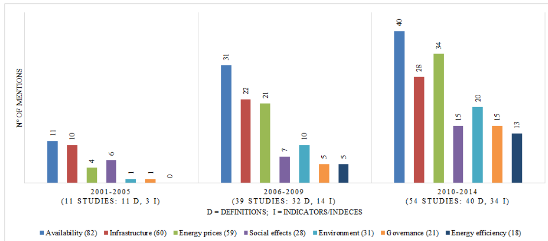
Figure 3.2 – Dimensions of energy security by period (2001-2014)
