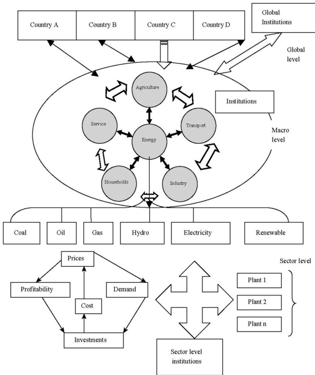
Figure 2.5 – Multidimensional relations in the energy sector
