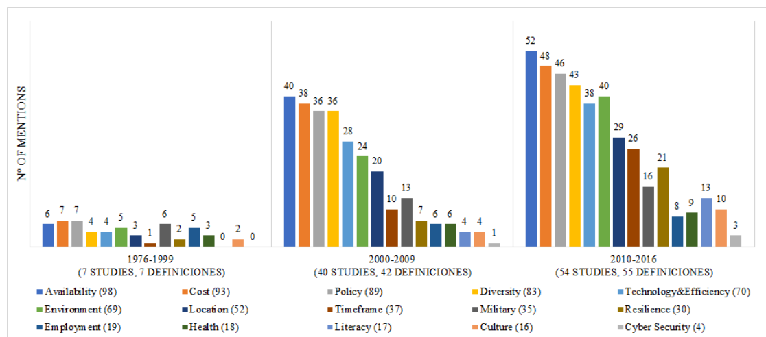
Figure 3.3 – Dimensions of energy security by different periods (1970-2016)
