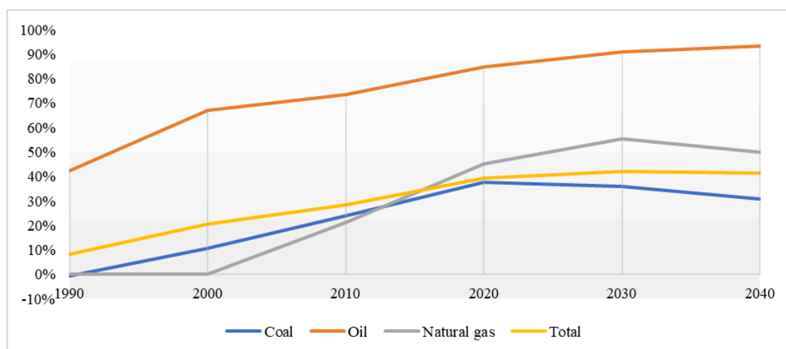
Figure 7.2 – Dependency on fossil fuels 1990-2040 (%)
