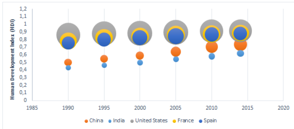
Figure 3.7 – Link between energy consumption per capita and human development
