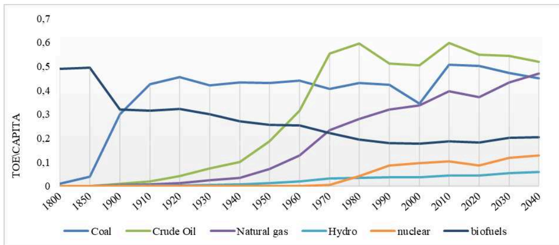
Figure 2.4 – Evolution of World energy consumption per capita (1800-2040)
