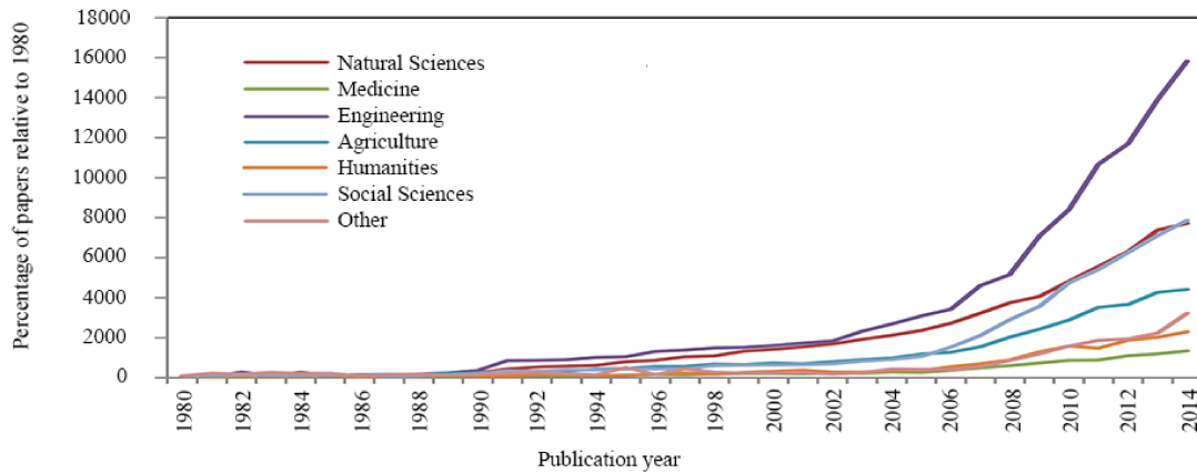
Figure 3.4 – Field-specific relative increase in climate change related papers published since 1980, based on the main OECD categories (the number of papers published in 1980 equals 100%).
