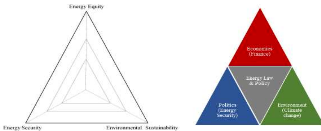
Figure 3.1 – Energy trilemma and Energy triangle
