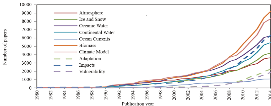
Figure 3.5 – Time evolution of the papers of the major subfields within climate change research
