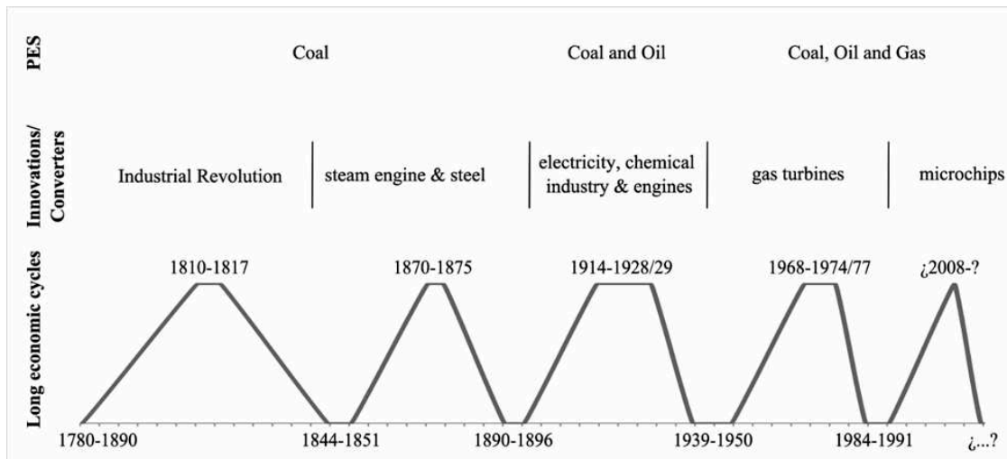
Figure 2.2 – Long economic cycles–Technological innovations–PES
