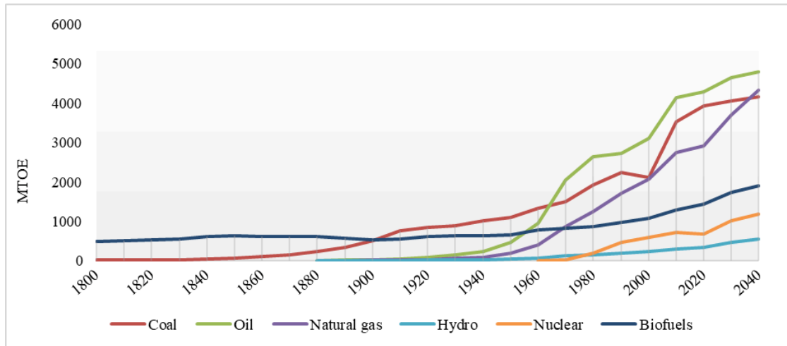
Figure 2.3 – Evolution of World energy consumption (1800-2040)
