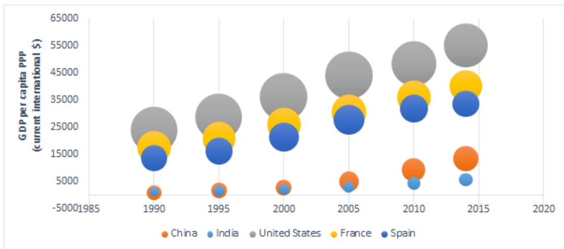
Figure 3.6 – Link between energy consumption and national income (per capita)
