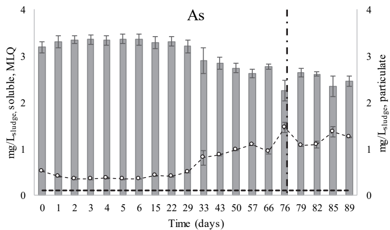
Figure 12. Examples of soluble (dashed line with circles) and particulate (bars) elements' concentration over time. The bold horizontal dashed line is the method limit of quantification (MLQ) for soluble elements whereas the vertical dashed line indicates the beginning of forced aeration.
