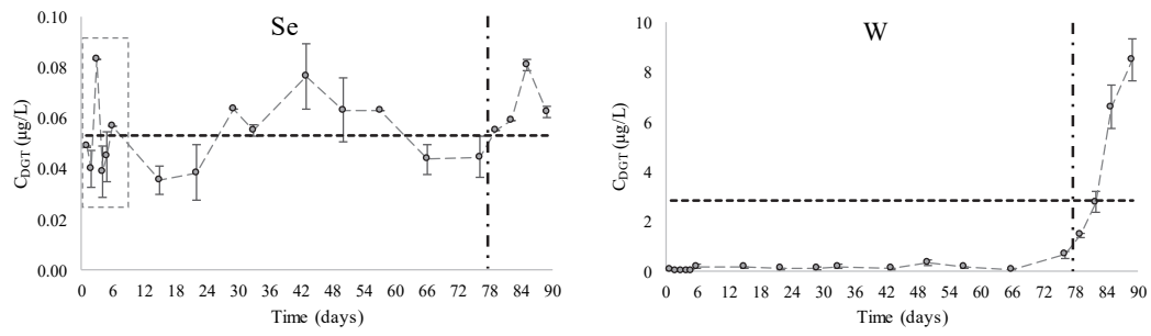
Figure A5. Labile trace elements (grey dashed line with grey circles) monitored over time in digested sewage sludge. The bold horizontal dashed line is the MLD_{DGT} or MLQ_{DGT} whereas the vertical dashed line indicates the beginning of forced aeration (Paper III).
