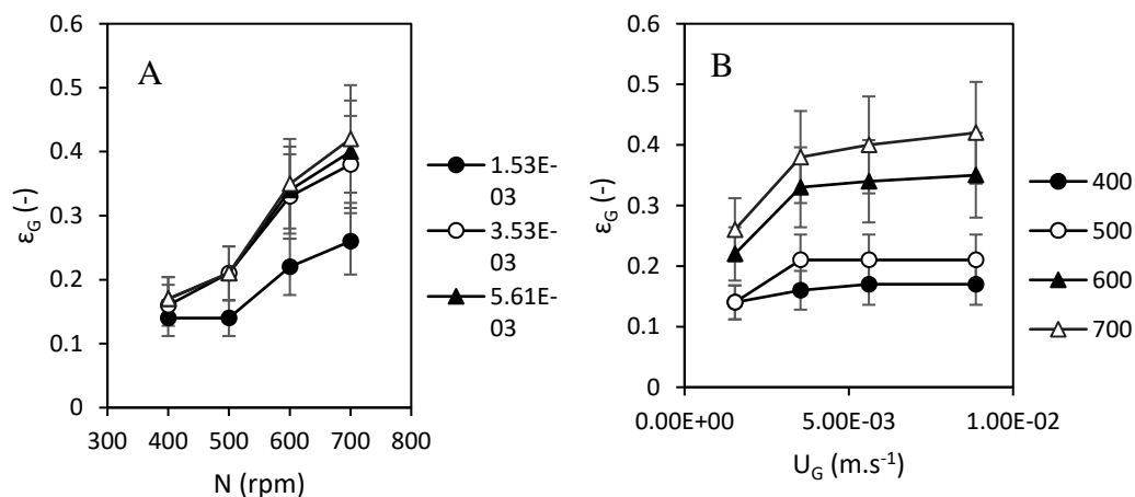
Figure S8 Gas holdup at 20% w/v clay concentration; A: Effect of stirring speed for different air superficial velocities (in m.s-1); B: Effect of air superficial velocity for different stirring speeds (in rpm)
