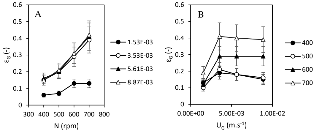
Figure S2 Gas holdup at 0.1% w/v clay concentration; A: Effect of stirring speed for different air superficial velocities (in m \cdot s^{-1} ); B: Effect of air superficial velocity for different stirring speeds (in rpm)
