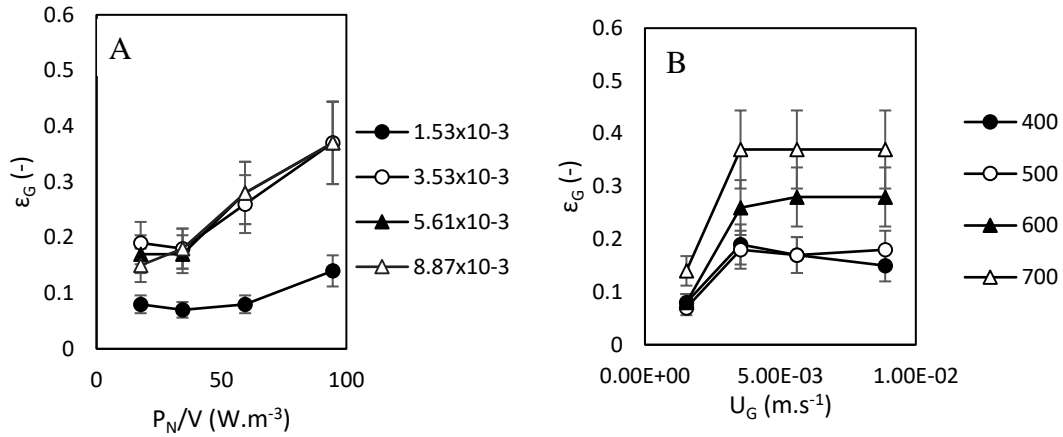
Figure S1 Gas holdup for tap water; A: Effect of power input for different air superficial velocities (in m \cdot s^{-1} ); B: Effect of air superficial velocity for different stirring speeds (in rpm)
