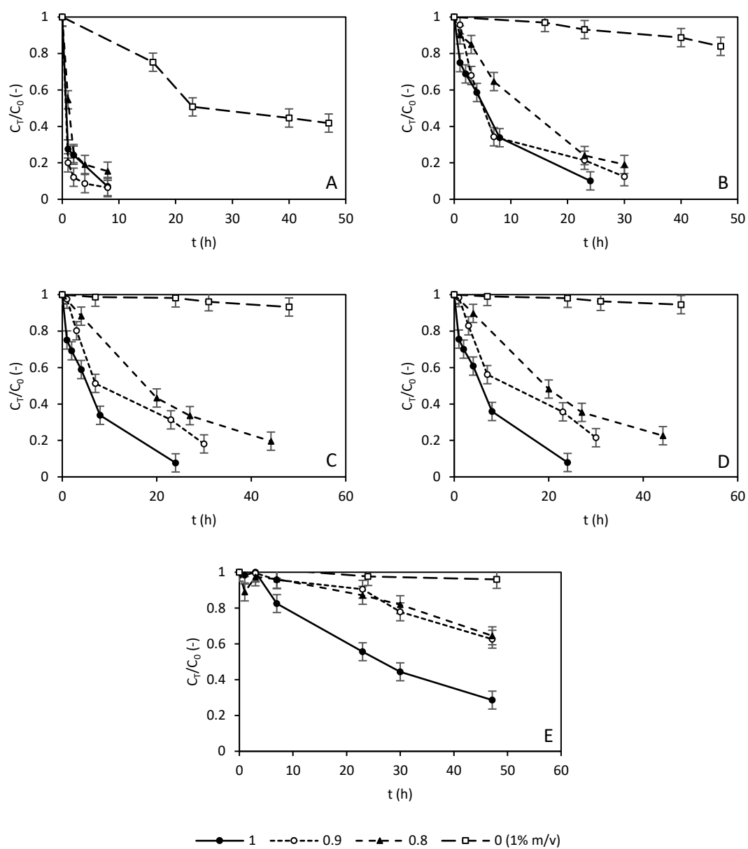
Figure 4.4 Desorption curves at different clay mass fractions for (A) naphthalene; (B) phenanthrene; (C) fluoranthene; (D) pyrene; and (E) benzo(a)pyrene
