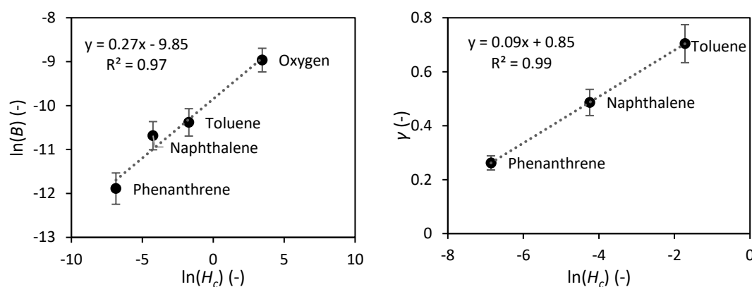
Figure 3.7 Linear correlations between the parameters in Eq. 33 and \ln(H_C)
