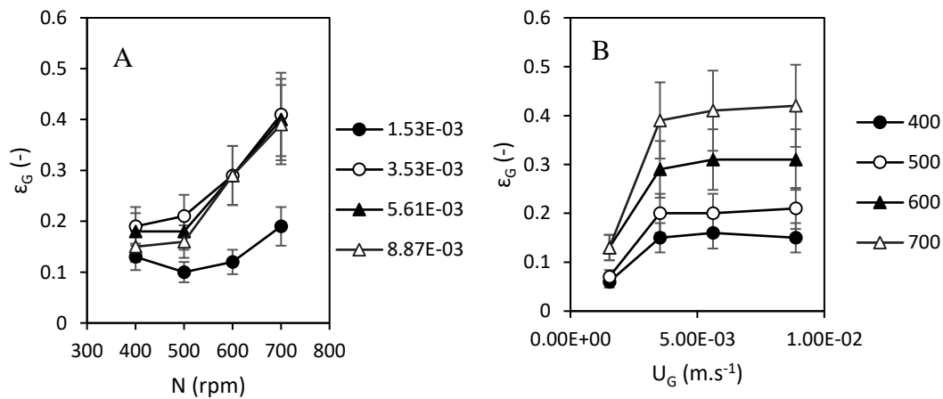
Figure S3 Gas holdup at 0.5% w/v clay concentration; A: Effect of stirring speed for different air superficial velocities (in m \cdot s^{-1} ); B: Effect of air superficial velocity for different stirring speeds (in rpm)
