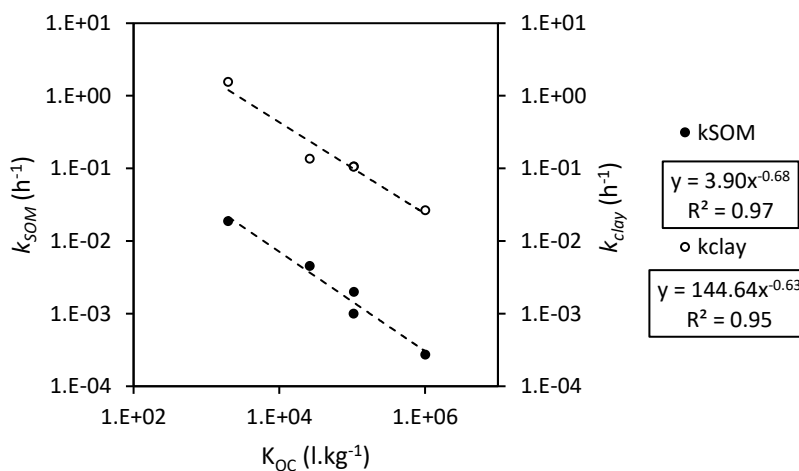
Figure 4.9 Estimated desorption kinetic constants for the pure fractions as a function of K_{OC} (from NJDEP, 2008 [24])
