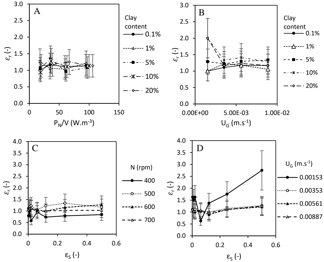
Figure 2.5 Effect of operational parameters on the relative gas holdup; (A) Effect of power input for different clay contents (% w/v) at U_G = 8.83 \times 10^{-3} \text{ m.s}^{-1} ; (B) Effect of air superficial velocity for different clay contents (% w/v) at N = 500 \text{ rpm} ; Effect of the solid volume fraction on the relative gas holdup (C) at different stirring speed (rpm) at U_G = 3.53 \times 10^{-3} \text{ m.s}^{-1} ; (D) at different air superficial velocities ( \text{m.s}^{-1} ) at N = 600 \text{ rpm} .
