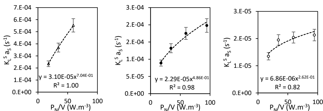
Figure 3.6 Influence of Power input on the surface mass transfer coefficient for (Δ) Toluene, (●) Naphthalene and (○) Phenanthrene
