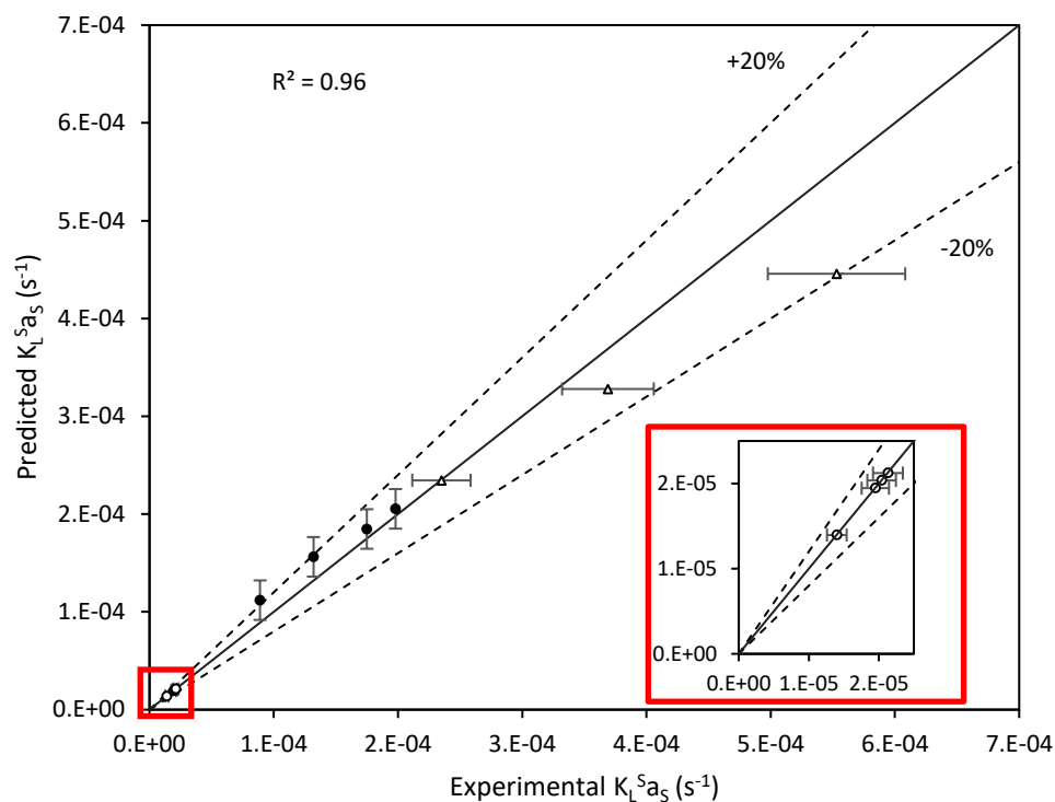
Figure 3.8 HOC mass transfer coefficients correlation for the PC model coefficient for (Δ) Toluene, (●) Naphthalene and (○) Phenanthrene
