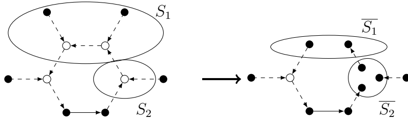
Figure 5.21 – Construction of \Gamma_{S_1, S_2} for some degree 5 BCR diagram
