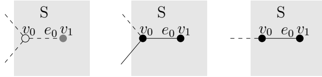
Figure 5.7 – The second property in the definition of \mathcal{H}_1(\Gamma)
