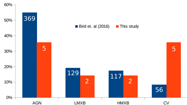
Fig. 3. Distribution of the 14 sources presented in this paper, alongside the 671 identified IGR sources presented in Bird et al. (2016). The left axis is normalized to the fraction (%) of the sources with respect to the total number of sources in their study, while the actual number of sources are indicated in white.
