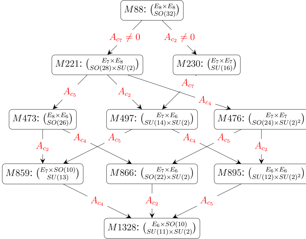
Figure 8.6: Links between various reflexive polyhedra. Going upward from M1328 amounts to removing points in the polytope M1328 , or equivalently monomials in the hypersurface equations (8.2) and (8.3). Going downward corresponds to adding a complex modulus A_{c\#} .
