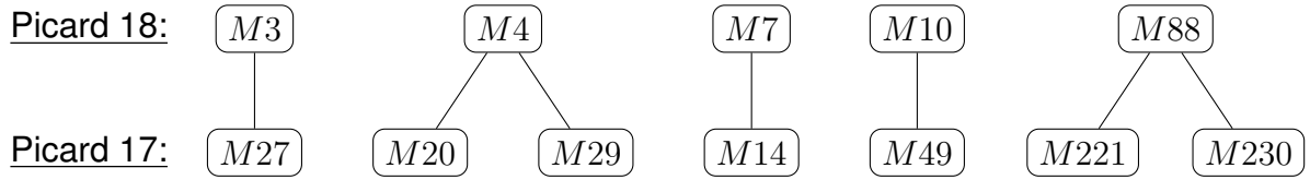
Figure 8.5: Links between polytopes with Picard 18 and 17. Going from Picard 17 to 18 amounts to removing a point in the polytope in the M lattice (i.e. a monomial in the hypersurface equation which defines the K3 surface).
