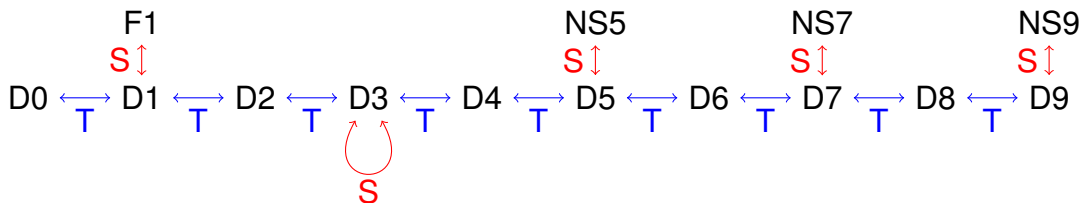
Figure 4.1: T and S duality relations between Type IIA and IIB branes.
