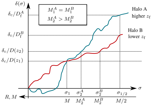
Figure 4. Pictorial representation of the interplay between accretion rate and formation time as inferred from excursion sets. Two haloes A and B upcross the threshold \delta_c/D(z_1) at the same \sigma . At redshift z_1 , they have therefore the same mass. Halo A has a steeper slope than halo B, and has thus a lower accretion rate. At a slightly larger redshift z_2 , halo A crosses the higher threshold \delta_c/D(z_2) at a lower \sigma , and its mass is thus larger than halo B's: halo A assembles its mass earlier, consistent with its lower accretion at z_1 . At the half-mass scale \sigma_{1/2} = \sigma(M/2) , the trajectory of halo A is higher: its threshold \delta_c/D_f has a value of D_f lower than halo B's at the same \sigma_{1/2} . Halo A has thus assembled half of its mass at a redshift z_f higher than halo B.
