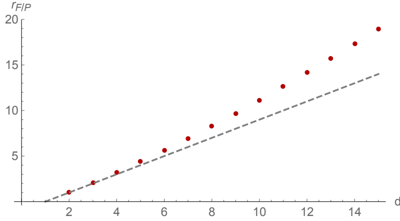
Figure 4.A.2: The ratio of peak to filament merger as a function of d . For reference, the first diagonal is shown as a dashed grey line as well. The ratio is approximately fitted as d - 1 + ((2d - 4)/7)^{7/4}/2 and shown as red dots. The dashed line is the identity.
