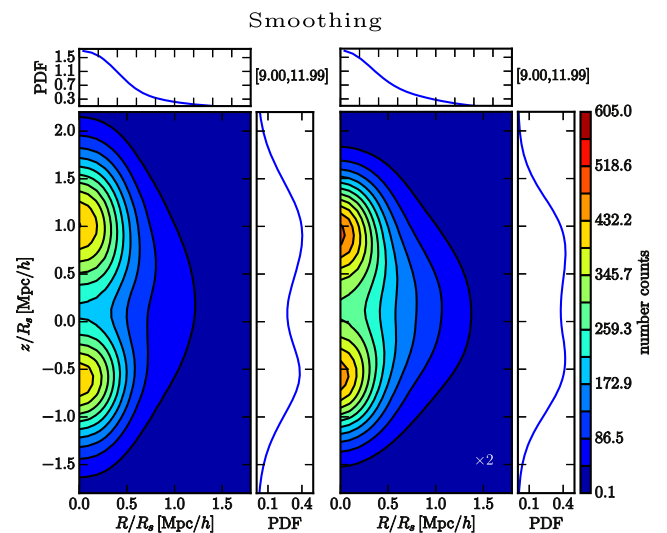
Figure A1. Galaxy number counts in the frame of the saddle (curvilinear coordinates) for all masses in the range 10^{9.0}-10^{12.0} M_{\odot} at redshift zero (left) compared to the smoothing twice as big (right). Note that the R - and z -axes have been rescaled by the smoothing length. Similarity of the contours suggest that the measured distributions are relatively insensitive to the choice of the smoothing length.
