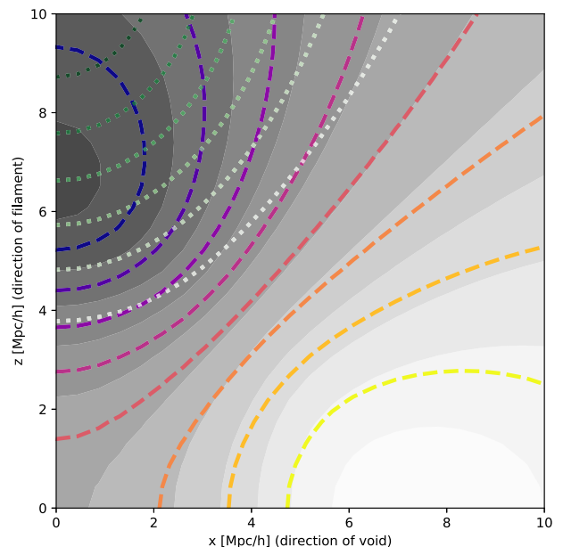
Figure 13. Isocontours of constant typical redshift z = 0 mean density (filled contours), mass (dotted lines) and accretion rate (dashed lines) in the frame of a filament (along the Oz axis) in Lagrangian space (initial conditions) from low (light colours) to high values (dark colours). The saddle is at coordinate (0,0) while the induced peak and void are at coordinates (0, \pm 7) and (\pm 8, 0) h^{-1} Mpc, respectively. As argued in the main text, this figure shows that the contours, hence the gradients of the three fields, are not parallel (the contours cross). The choice of scale sets the units on the x - and z -axis (chosen here to be 5 h^{-1} Mpc, while the mass and accretion rates are computed for a local smoothing of 0.5 h^{-1} Mpc). At lower redshift/smaller scales, one expects the non-linear convergence of the flow towards the filament to bring those contours together, aligning the gradients (see Fig. 14).
