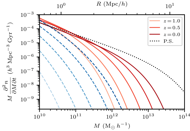
Figure 4.5.1: PDF of the halo merger rate (solid red lines) and the wall merger rate (dashed blue lines) as a function of redshift of formation (from dark to light at z = 0, 0.25, 0.5, 0.75, 1 ), see the text for details, up to a renormalisation. For the sake of clarity, only the redshifts z = 0, 0.5, 1 appear in the legend. For small masses the merger rate follows the Press-Schechter (Press and Schechter, 1974) halo mass function up to a renormalisation (black dotted line), while at larger masses the halo merger rate decays significantly faster. As expected, the transition mass increases with time. The same evolution is found for void mergers.
