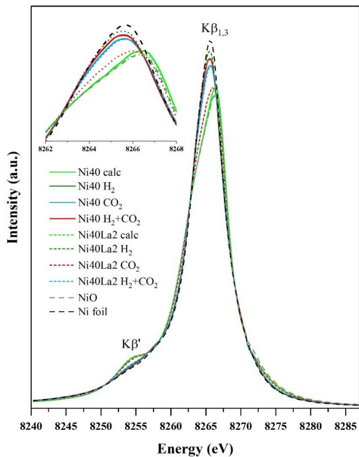
Figure 10.5 Ni Kβ core-to-core XES spectra of both catalysts under various conditions together with NiO and Ni foil as standards.
