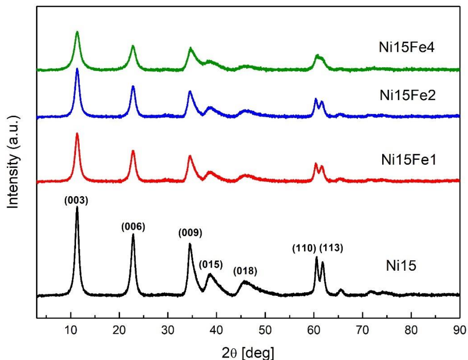
Figure 8.1 XRD patterns of as-synthesized Ni and Ni-Fe hydroxaltes-like materials
