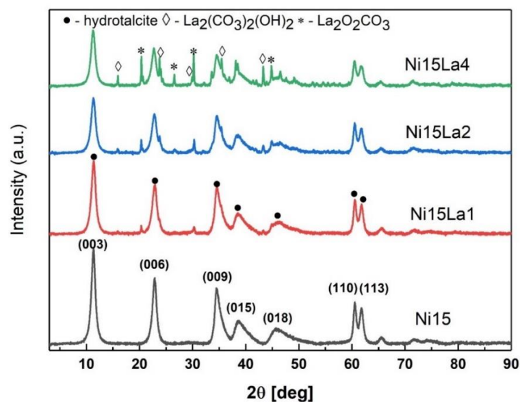
Figure 8.8 XRD patterns of the as-synthesized hydrotalcite-like materials
