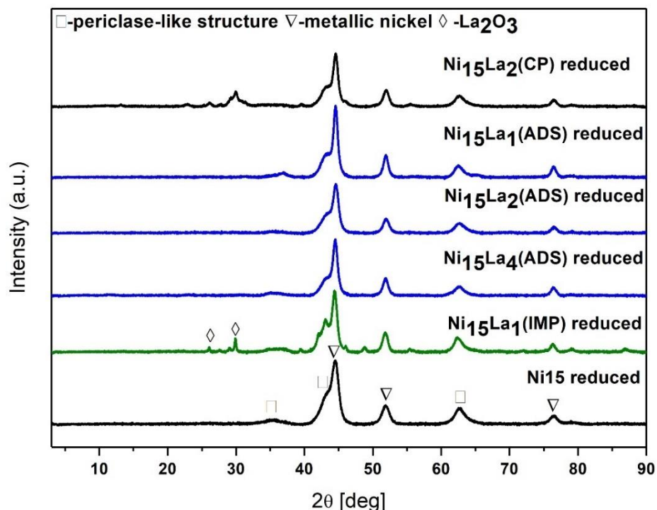
Figure 8.18 XRD patterns for the reduced catalysts, reduction conditions: 900°C for 1h in 100ml/min of 10% H_2 /Ar
