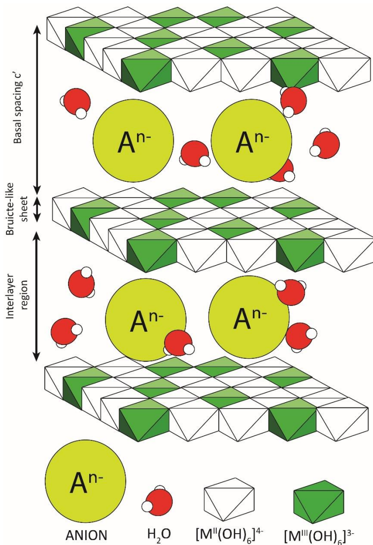
Figure 5.1 Scheme of the hydrotalcite structure
