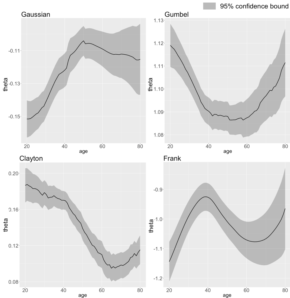
Fig. 3.3: For each copula family, mean value of the conditional copula parameter as a function of the age x ( h = 20 , n = 10000 , 100 repetitions). As we notice in Section 3.4.2, the Gumbel copula and the Clayton copula don't vary in the same direction as the Gaussian copula and the Frank copula.
