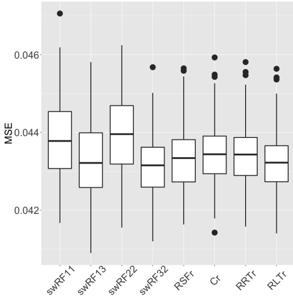
Fig. 4.4: Boxplot of the performances (MSE) of the models; \phi = \phi_{ch} , with RSF weights.
