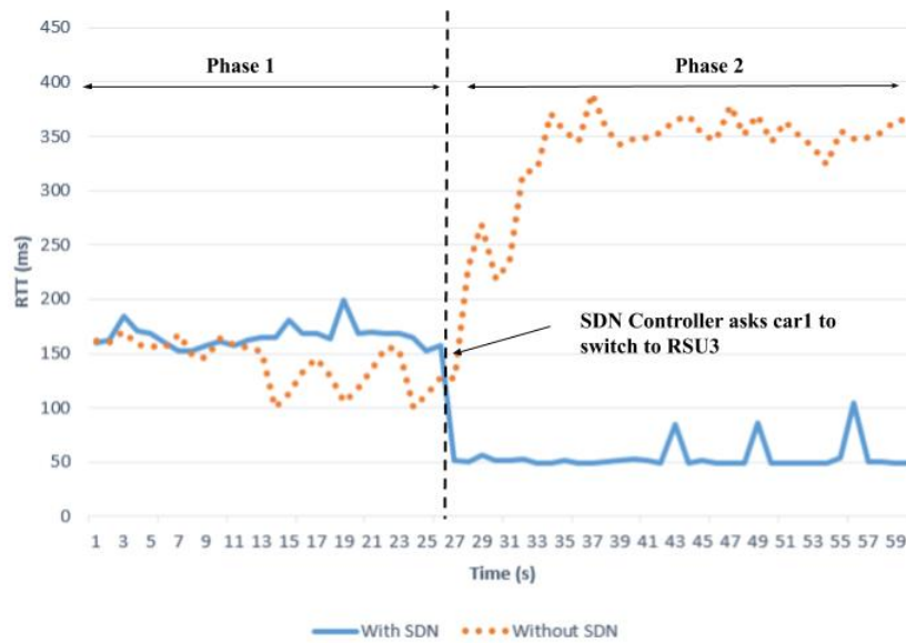
FIGURE 1.13: Délai de transmission aller-retour RTT
