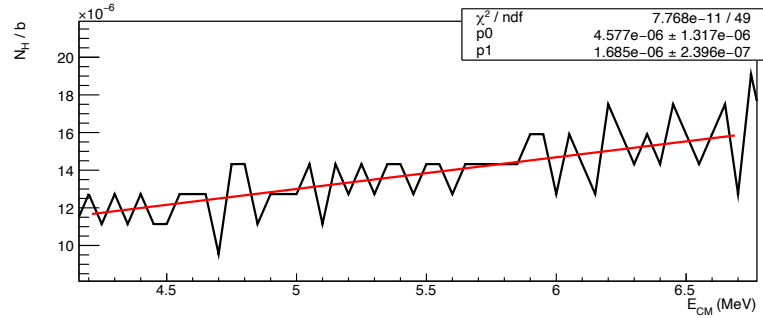
Figure 2.20: Number of hydrogen atoms per barn as a function of the CM energy at which the elastic reaction took place.
