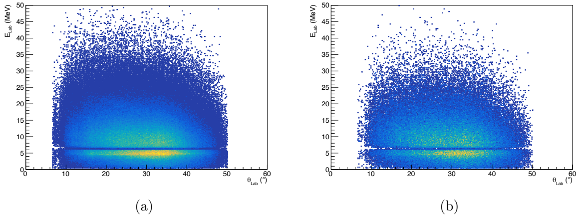
Figure 3.24: Measured energy of the two-proton events as a function of their measured angle in the laboratory. For a CH_2 target on the left (target n°3) and for a ^{nat}C target on the right. As it can be observed, except for the difference of statistics, the two histograms are similar.
