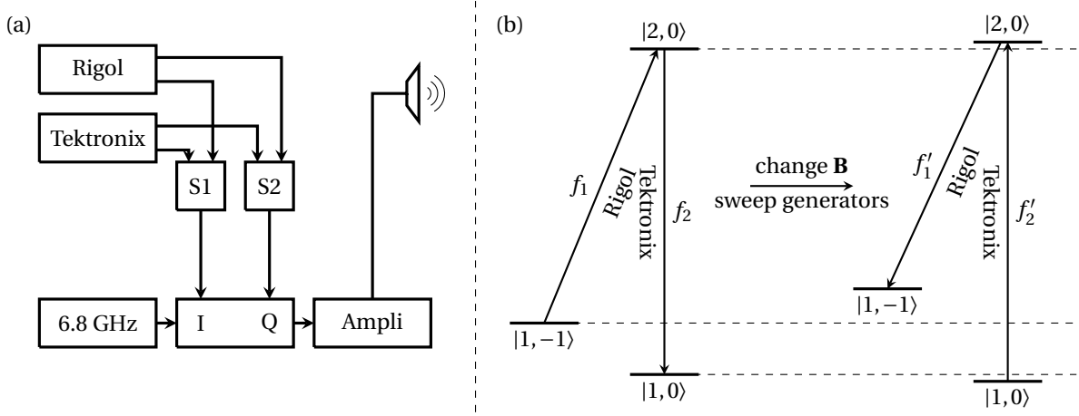
Figure 3.3: Left: scheme of the MW chain: each generator delivers two signals in quadrature that are mixed by an IQ mixer. Two switches S1 and S2 let either one or the other generator access to the IQ mixer. This is mixed with a 6.8 GHz source in order to create a signal at \sim 6.834 GHz, which is then amplified and sent to the atoms. Right: scheme to perform 4 transitions: we first operate f_1 with Rigol and f_2 with Tektronix in order to arrive to |1, 0\rangle . The two generators are then swept to the new relevant frequencies f'_1 and f'_2 while the magnetic fields are changed to their final values. Then, Tektronix transfers atoms back to |2, 0\rangle and Rigol transfers them back to |1, -1\rangle .
