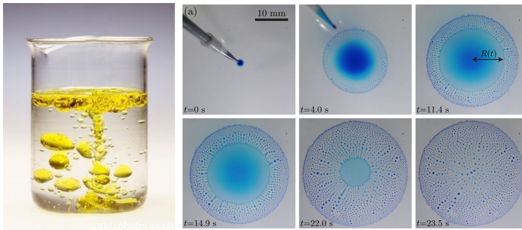
Figure 5.1: Oil and water are immiscible (left). However, when alcohol is added to water in sufficient quantity (right), the situation changes dramatically: such a droplet quickly expands over the oil surface, before receding due to alcohol evaporation. As the layer is thicker in the centre, the alcohol tends to evaporate faster on the edge. This translates into a gradient of surface tension towards the rim, which causes an accumulation of liquid there. Due to a Plateau-Rayleigh-like instability, this bulge collapses into a multitude of small droplets, whose exact size depends on the concentration of alcohol in the mixture. Figure taken from [118].
