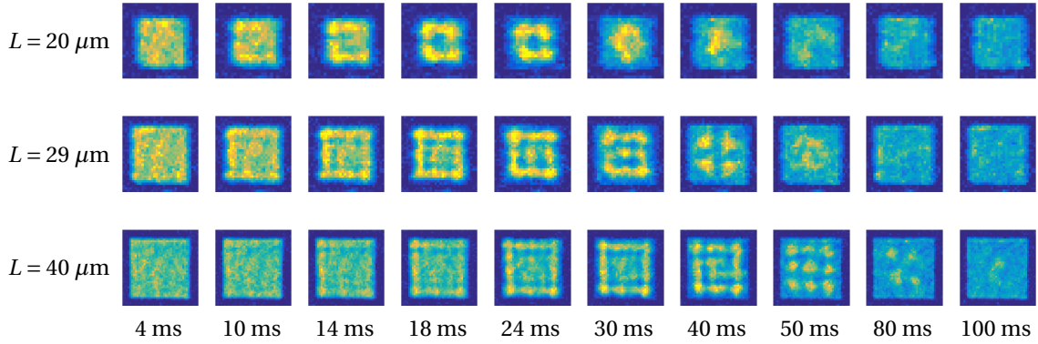
Figure 8.6: Time evolution of the |2, 0\rangle density for L = 20, 29, and 40 \mu\text{m} . All the densities are close to each other (typically 82 \mu\text{m}^{-2} ). We observe more or less equivalent k at equivalent times.
