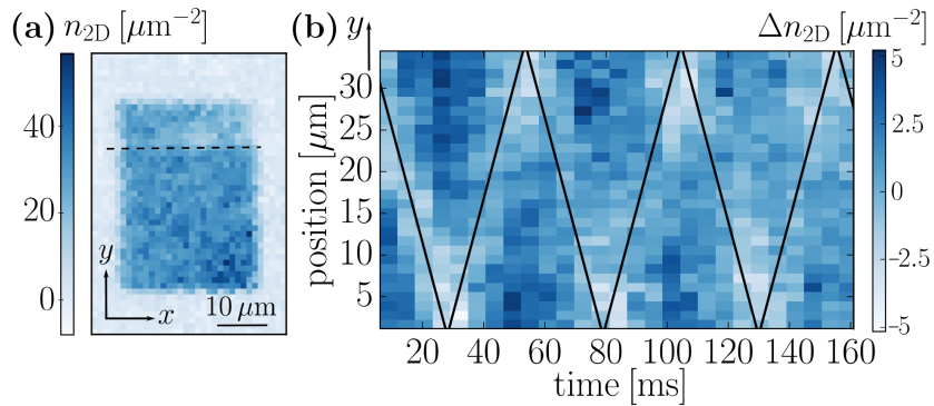
Figure 2.1: Excitation of sound waves. An extra potential step is added on our uniform gas, creating a perturbation that is free to propagate in the atomic box (a). By integrating the atomic density along x for different times (b), one can monitor the displacement of the wave front, and measure the speed of sound. Figure taken from [77].
