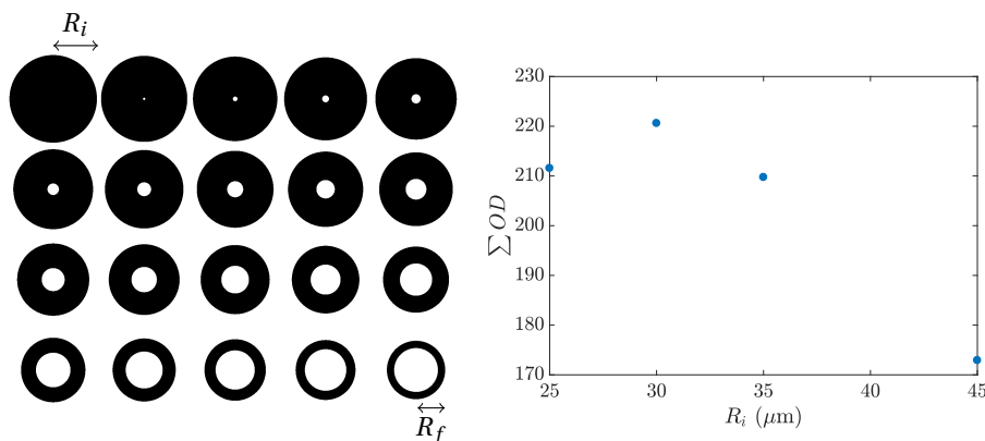
Figure 7.1: Left: images used for the movie: a disk of initial radius R_i is transformed into a ring of outer radius R_f = 20 \mu\text{m} (the inner radius here is 15 \mu\text{m} ). Right: effect of R_i on the ring’s loading: we vary R_i and compute in each case the sum of all the pixels’ OD. We find that for this R_f , it is maximal for R_i = 30 \mu\text{m} .
