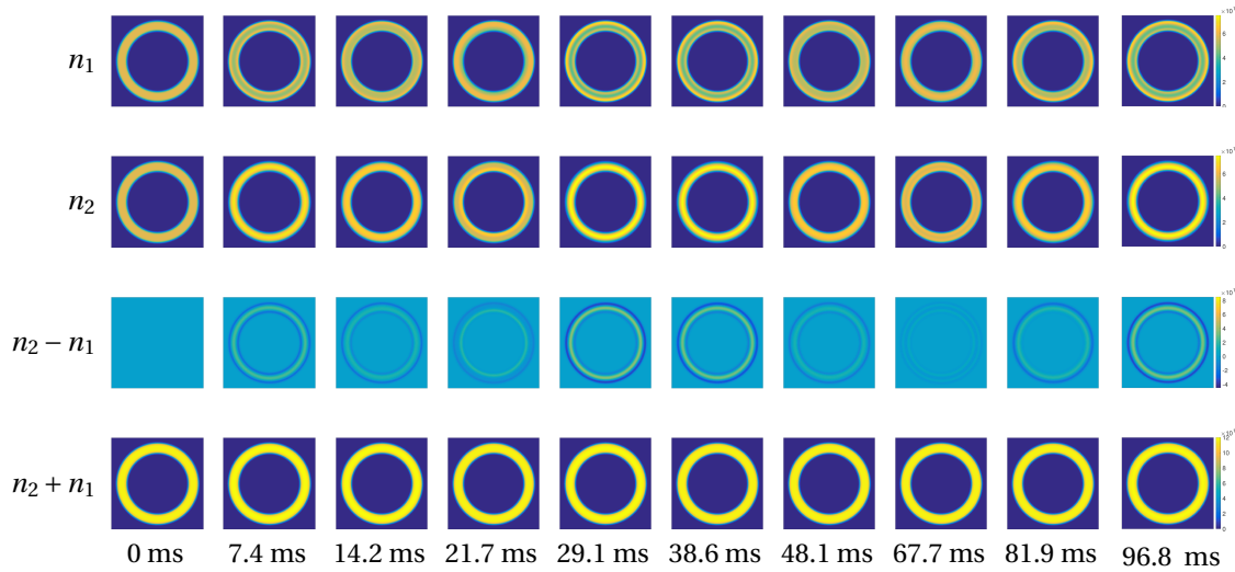
Figure 6.15: Simulation of demixing in SSBC with no seed for n_{\text{tot}} = 30 \mu\text{m}^{-2} . Only radial dynamics with small amplitudes take place up to 100 ms.
