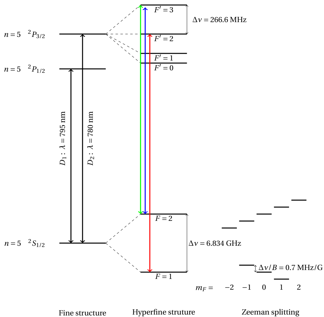
Figure 3.1: Electrical level of ^{87}\text{Rb} . We work with the D2 line. The cooling transition is indicated in blue and the imaging one in green. We also have a repumper beam depicted in red.
