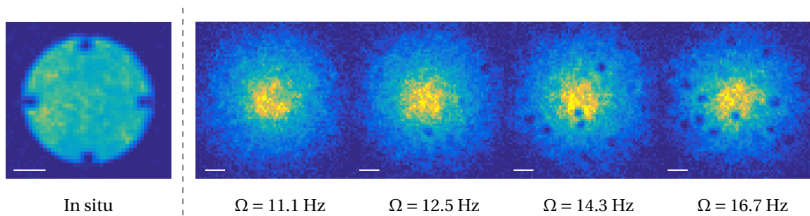
Figure 8.16: Left: stirring created by DMD2 (in situ image). The four teeth rotate at certain frequency in order to inject angular momentum in the cloud. Right: after 10 turns, we image the vortices with a time of flight measurement. The number of vortices grows as we increase the injected angular momentum. The white lines represent 10 \mu\text{m} .
