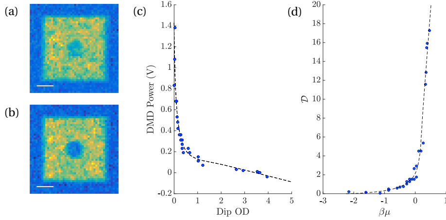
Figure 3.5: Left: absorption images of the cloud. At high DMD2 power (b), the dip created by the extra excitation is almost totally depleted, which is not the case at lower DMD2 power (a). The white line represents 10 \mu\text{m} . Middle: example of the fitting procedure (black dotted line) described above. For this example, we find \bar{T}/T_c = 0.43 and T = 125 \text{ nK} . Right: Same thing but the axis OD and DMD Power have been converted to \mathcal{D} and \beta\mu , respectively.
