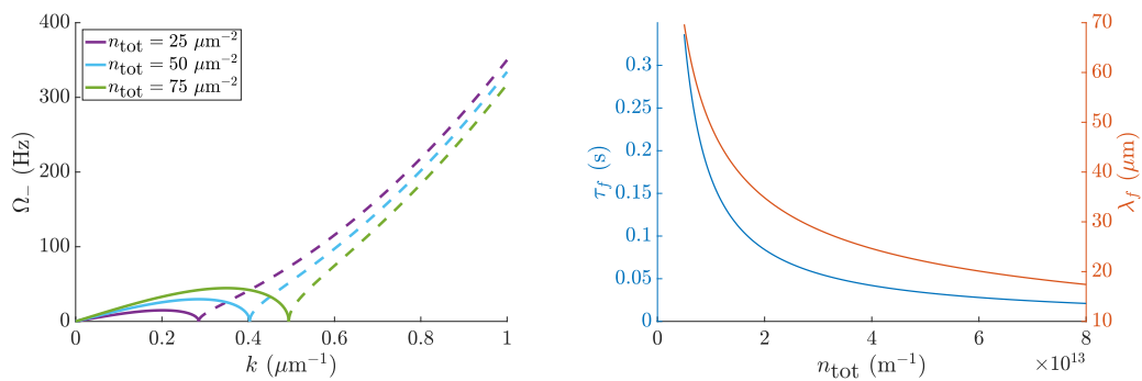
Figure 5.8: Left: evolution \Omega_-(k) with n_{\text{tot}} for a balanced mixture while a_{12} is fixed at 98.9 a_0 . As before, \Omega_- is purely imaginary where the line is solid and real when it is dashed. Right: corresponding appearing wavelength \lambda_f and characteristic growth time \tau_f .
