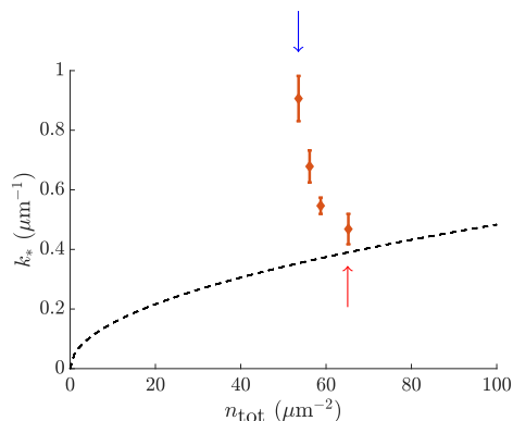
Figure 8.11: Evolution of k_* for temperatures ranging from 78 to 415 nK. The blue arrow denotes the coldest point, and the red arrow the hottest one. The dashed black line represents the prediction from [61] for k_f . We see that in this case, increasing T decreases significantly k_* .
