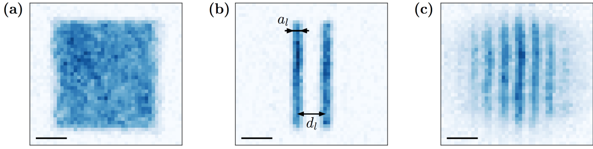
Figure 2.7: Measurement of g_1 with an interferometric method. Two lines (b) are selected from the initial cloud (a) and interfere (c). Averaging (c) over different iterations and extracting the central interference contrast enables us to measure G_1(d_l) . The black line represents 10 \mu\text{m} . Figure taken from [81].
