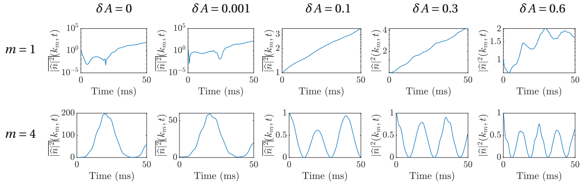
Figure 6.12: Population of the seeded mode for different amplitudes of seed ( n_{\text{tot}} = 30 \mu\text{m}^{-2} , SBC). Top row: we seed m = 1 and vary \delta A from 0 to 0.6. We recover an exponential behaviour for a large enough seed, but this behaviour is lost again when \delta A is increased too much (the graphs are in semi-log scale). Bottom row: same thing for m = 4 . For too small a seed ( \delta A = 0.001 for instance), the modulation is amplified before collapsing (see the (linear) scale), but this behaviour is quite different from the oscillatory nature observed for larger \delta A .
