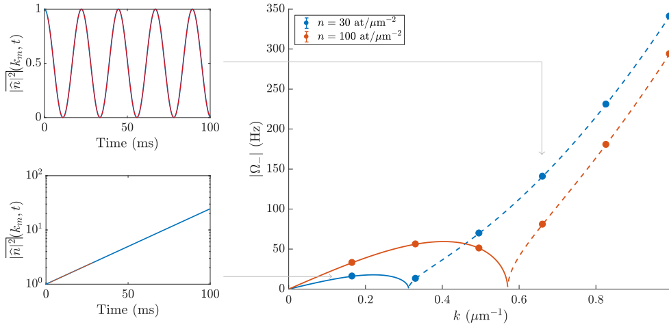
Figure 6.9: Left: example of the time evolution for a stable (top, m = 4 ) and an unstable (bottom, m = 1 ) mode. The red lines are respectively a cosine and an exponential fit. Right: |\Omega_-| for different k at two different atomic densities (PBC, \delta A = 10^{-3} ). The regions where \Omega_- \in i\mathbb{R} are represented with solid lines, while the regions where \Omega_- \in \mathbb{R} are in dotted lines.
