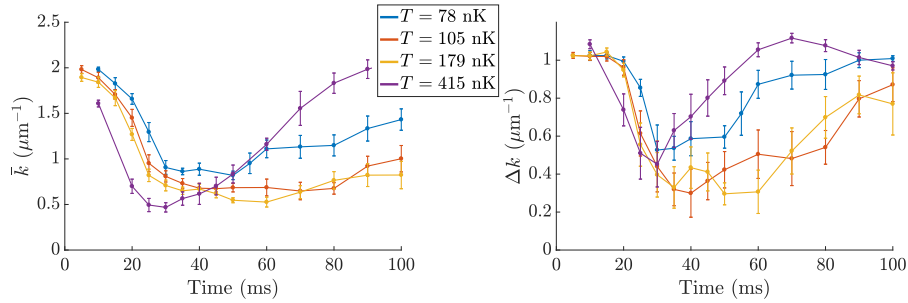
Figure 8.10: Evolution of the mean wave vector \bar{k} present in the system (left), and its standard deviation \Delta k (right) with time, for a box of side L = 40 \mu\text{m} and temperatures T = 78, 105, 179, and 415 nK. The total density is typically 58 \mu\text{m}^{-2} . Each value is averaged over typically 10 iterations; the error bars are the resulting standard deviations over these \simeq 10 iterations.
