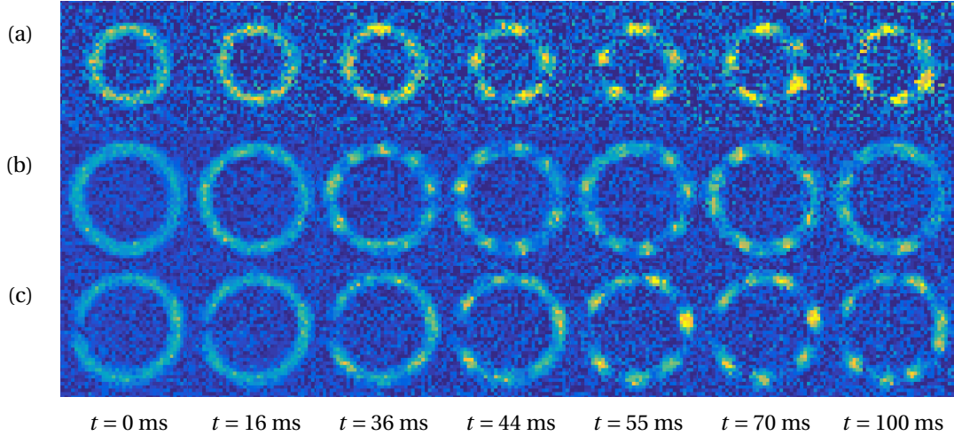
Figure 7.2: Examples of natural demixing experiments in rings of inner and outer radii 10 and 15 \mu\text{m} (top), and 15 and 20 \mu\text{m} (middle/bottom). The bottom ring is cut on its left side. No average has been performed as the blob’s locations are not fixed for the top and middle row.
