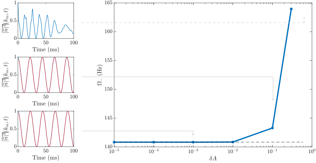
Figure 6.8: Left: we seed the mode 4 of the box (PBC, n_{\text{tot}} = 30 \mu\text{m}^{-2} ) and look at |\hat{n}|^2(k_4, t) , normalised to its initial value, for different amplitudes: \delta A = 10^{-3} (bottom), \delta A = 0.1 (middle), and \delta A = 0.6 (top). We then fit this signal to extract a period showed on the right graph (for the first two graphs, the red line is a cosine fit). When the seed's amplitude becomes too large, non-linearities start appearing, which lead to a non monomode signal. The 3D infinite prediction is shown in dashed lines.
