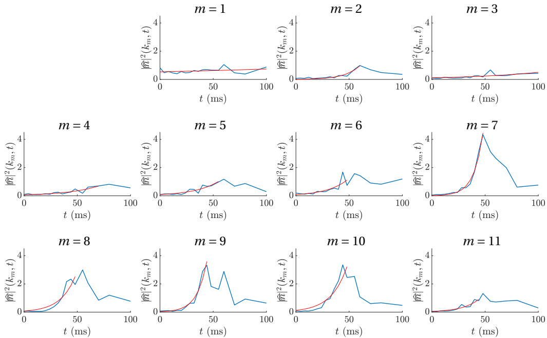
Figure 7.4: Example for the highest density run performed in a large ring. We fit each |\hat{n}|^2(k_m = m/\bar{R}, t) , with m \in \mathbb{N} , by an exponential (in red), and extract a characteristic time scale. In this example, only modes 7-10 get significantly populated.
