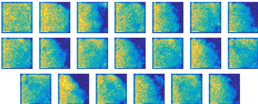
Figure 4.12: Evolution of the atomic density along the loop, for K = 0.25 . Iterations are going from left to right, then from top to bottom. We see that even if \mathcal{F} seems to have reached a steady state at iteration 3, in effect, some regions overshoot and some others undershoot, leading to a more or less constant \mathcal{F} .
