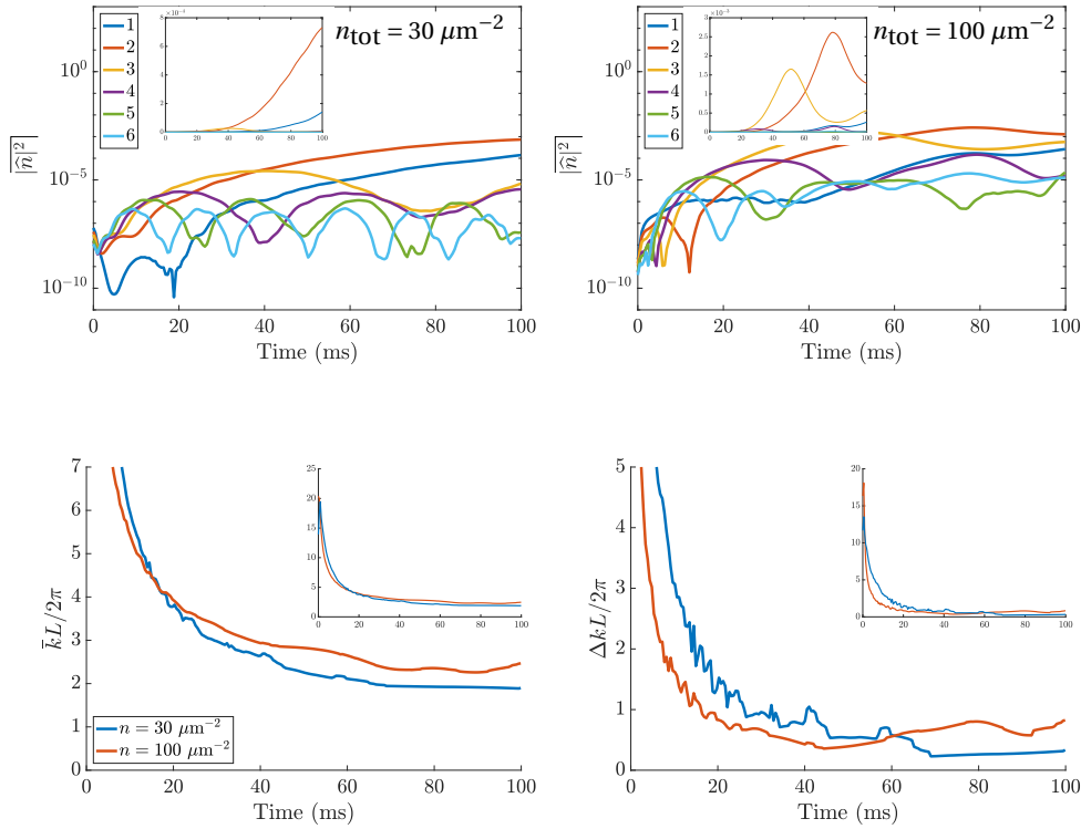
Figure 6.11: Simulation of demixing in a box with no seed. Top: evolution of each mode population |\hat{n}|^2(k_m, t) versus time for n_{\text{tot}} = 30 \mu\text{m}^{-2} (left) and n_{\text{tot}} = 100 \mu\text{m}^{-2} (right), for m \in [1, 6] . The data is shown in semilog scale, while the insets show the same data in a linear scale. Bottom: evolution of \bar{k}(t) (left) and \Delta k(t) (right) in dimensionless units for the same two runs (the insets are the same non-zoomed data). The 3 first graphs show a cascade from high k to smaller k during time evolution, which is also visible in Fig. 6.10.
