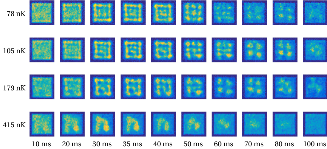
Figure 8.9: Time evolution of the |2, 0\rangle density for T = 78, 105, 179, and 415 nK, while the total density is kept at about 58 \mu\text{m}^{-2} . For these pictures, L = 40 \mu\text{m} . As the temperature is increased, the number of lobes created decreases, although the time of appearance is more or less constant.
