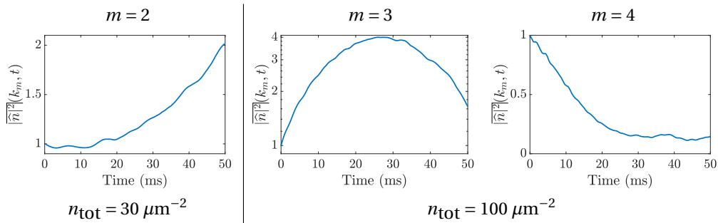
Figure 6.13: For modes too close to the stable/unstable border, the associated evolution time is large compared to the demixing time, and natural demixing takes over. Left: seeding of m = 2 for n_{\text{tot}} = 30 \mu\text{m}^{-2} ; this mode is supposed to oscillate. Middle: seeding of m = 3 for n_{\text{tot}} = 100 \mu\text{m}^{-2} ; this mode is supposed to grow exponentially. Right: seeding of m = 4 for n_{\text{tot}} = 100 \mu\text{m}^{-2} ; this mode is supposed to oscillate.
