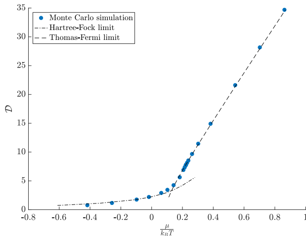
Figure 2.4: Equation of state of the 2D weakly interacting Bose gas, with \tilde{g} = 0.16 . The blue points are the results of Monte Carlo simulation performed in [40], and agree well with both Hartree-Fock and Thomas-Fermi limits.
