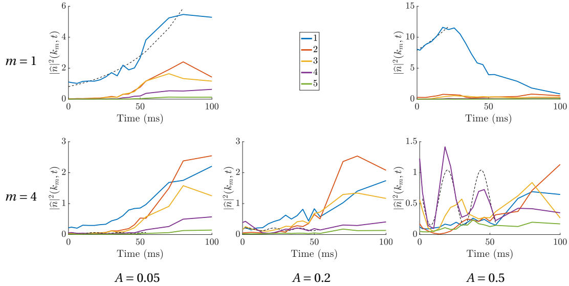
Figure 8.12: Behaviour of |\hat{n}|^2(k_m, t) for different seeds. Top: we seed m = 1 , which is an unstable mode for this density. For too large a seed, the mode only marginally grows before collapsing, making it hard to extract reliably a growth rate. Bottom: we seed m = 4 , which is a stable mode at this density. Below A = 0.5 , we hardly see any oscillation. This incited us to use large A when seeding a stable mode, and small A for unstable ones.
