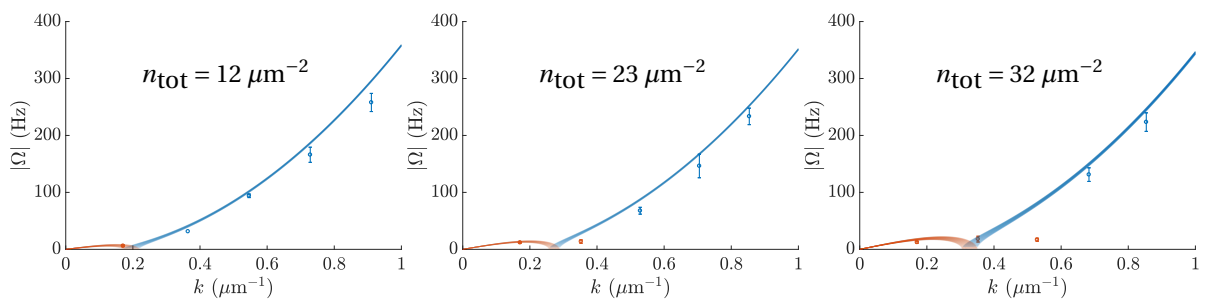
Figure 8.14: Dispersion relations for three different densities : 12 \mu\text{m}^{-2} (left), 23 \mu\text{m}^{-2} (middle) and 32 \mu\text{m}^{-2} (right). We seed modes 1-5 with A = 0.05 for unstable modes (red points) and A = 0.5 for stable ones (blue points). The prediction for an infinite system is shown in red when \Omega_- \in i\mathbb{R} and in blue when \Omega_- \in \mathbb{R} . Each run has a slightly different density (the standard deviation in density within each graph is typically 15 % of the mean), which gives rise to the corresponding shaded areas.
