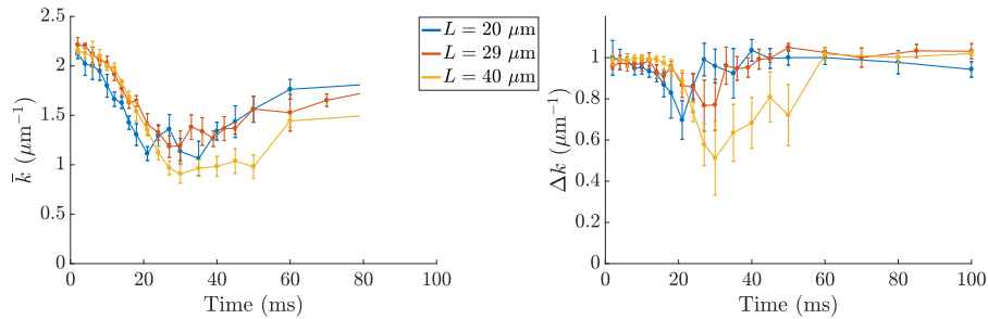
Figure 8.7: Evolution of the mean wave vector \bar{k} present in the system (left), and its standard deviation \Delta k (right) with time, for boxes of sides L = 20, 29, and 40 \mu\text{m} . The total density is typically 80 \mu\text{m}^{-2} . Each value is averaged over typically 10 iterations; the error bars are the resulting standard deviations over these 10 iterations.
