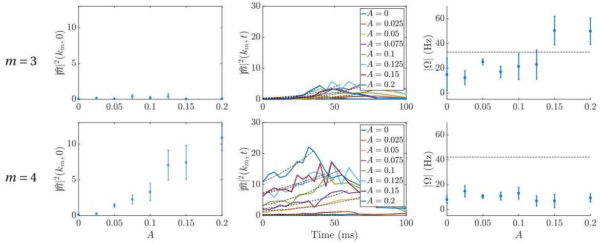
Figure 7.7: Left: Initial mode population for different values of the seed A . The curves for modes m \neq 4 are quite flat, and loosely populated, in opposition with the m = 4 case: the perturbation that we seed is quite monomode. Middle: time evolution of the modes' populations for different seeds A . Only mode 4 gets macroscopically populated. From this graph, we can extract a growth rate plotted on the right row: on the explored range, |\Omega| seems more or less independent of A for the seeded mode. The black dashed lines correspond to the prediction from [61] with the values from [131].
