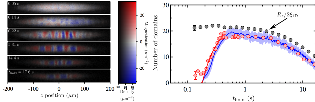
Figure 5.6: Left: a quasi 1D BEC of ^{87}\text{Rb} is initially prepared in an equal superposition of the 2 immiscible spin states |F = 1, m_F = \pm 1\rangle . The number of spin domains quickly increases, before slowly decreasing (see right): because of atomic losses, eventually, small domains cannot maintain a total polarisation and they coalesce into bigger domains. Right: number of domains with time. The red points are the experimentally observed values (typical uncertainty plotted on the leftmost point), the red line is an exponential fit, the blue line is a Gross-Pitaevskii simulation (with uncertainties denoted by the blue band), and the grey points correspond to the ratio R_z/2\xi where R_z is the Thomas-Fermi radius of the gas, and \xi the healing length. Considering that the system is of total size 2R_z and that the domains have a typical size of 4\xi , this ratio gives an estimate of the number of domains present in the system. Both figures are taken from [58].
