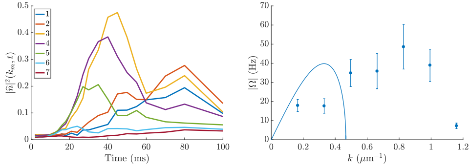
Figure 8.4: Left: evolution of each mode's population |\hat{n}|^2(k_m, t) for n_{\text{tot}} = 67 \mu\text{m}^{-2} , and L = 40 \mu\text{m} . As can be seen in Fig. 8.1, each mode grows before collapsing. Modes with a higher k collapse before modes with lower ones, causing a cascade of k on experimental images. Right: we can try to fit these modes's growths with exponentials; however, in this case, the obtained \Omega(k) is very different from what is expected in an infinite system (blue line). This naive picture is no longer applicable, and in order to better understand the system's important features, we decide to focus on a simpler observable: we look at the pattern's average mode number instead of performing this individual mode analysis.
