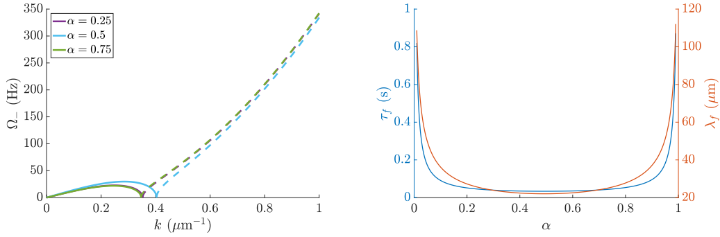
Figure 5.9: Left: evolution of \Omega_-(k) with \alpha while n_{\text{tot}} and a_{12} are fixed at 50 \mu\text{m}^{-2} and 98.9 a_0 , respectively. As before, \Omega_- is purely imaginary where the line is solid and real when it is dashed. Right: corresponding appearing wavelength \lambda_f and characteristic growth time \tau_f .
