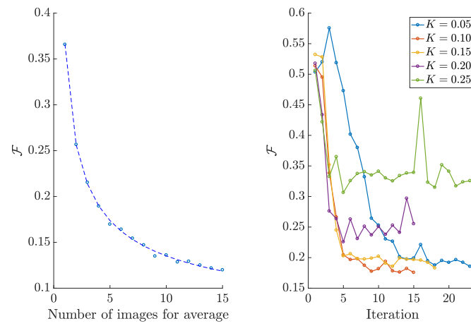
Figure 4.13: Left: decrease of \mathcal{F} with the number N_r of images taken. The dashed line is a square-root fit. Right: figures of m erite corresponding to gains K = 0.05 - 0.25 .
