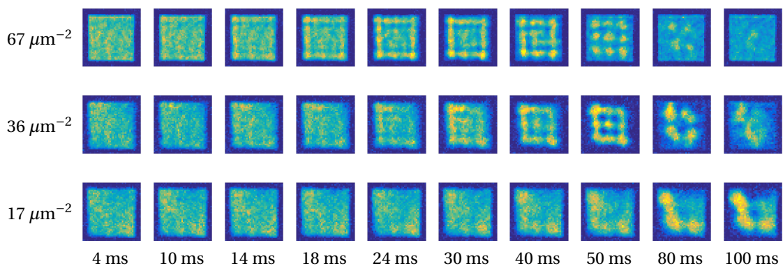
Figure 8.3: Average images of |2, 0\rangle populations for total atomic densities n_{\text{tot}} = 67 (top), 36 (middle), and 17 \mu\text{m}^{-2} (bottom). The box's size is 40 \mu\text{m} \times 40 \mu\text{m} , while T is typically set at 90 nK. We see that the higher the density, the faster the patterns appear, and the higher the mode.
