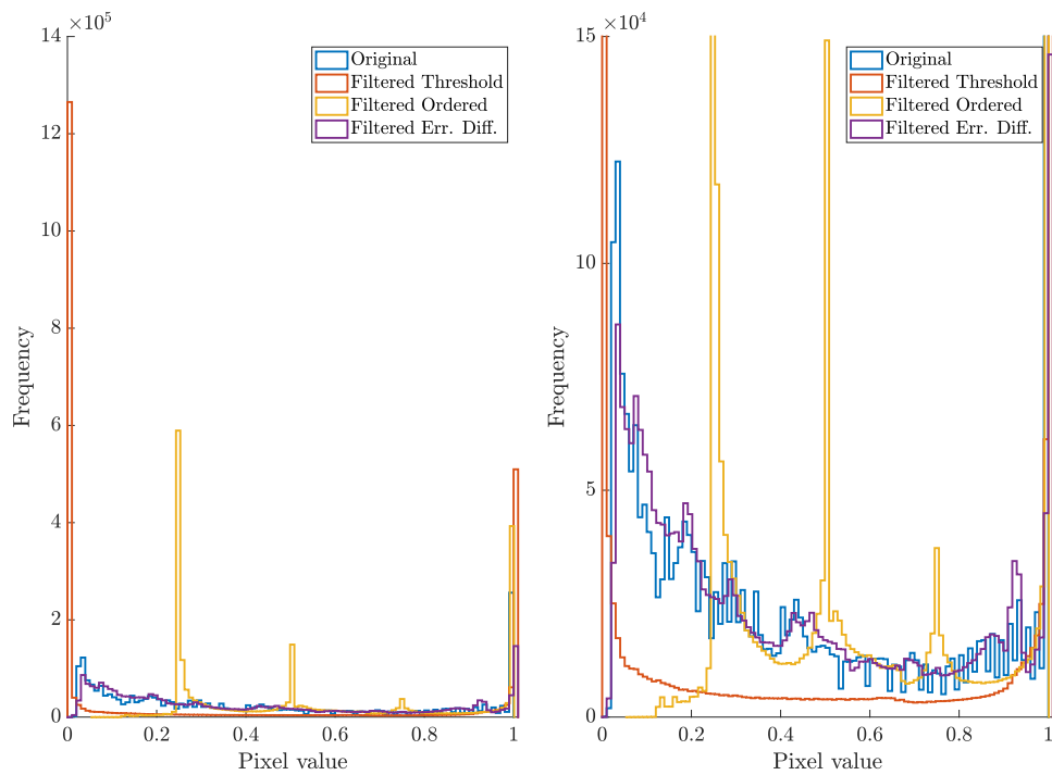
Figure 4.2: Statistics of dithered pixels for different algorithms. All the images have been convolved with a gaussian of width 15 pixels before being analysed. Left: histogram for original image, filtered threshold, filtered ordered, and filtered error diffusion ditherings. Right: enlarged version of the previous histogram. Threshold dithering is a method based on one threshold, and as such, produces two peaks on the histogram. Ordered dithering, with the previous matrix, is based on 3 thresholds, and thus creates four distinctive peaks on the histogram. Error-diffusion dithering, on the other hand, reproduces more faithfully the original distribution.
