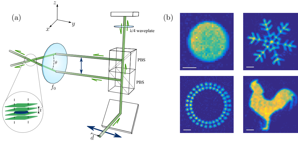
Figure 3.2: Left: optical accordion: by changing the impact position on the bottom right mirror, we can vary the interfringe from 11 \mu\text{m} to 2 \mu\text{m} . Figure taken from [76]. Right: absorption images of clouds for different boxes created by our DMD. The white lines represent 10 \mu\text{m} .
