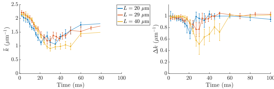
Figure 8.7: Evolution of the mean wave vector \bar{k} present in the system (left), and its standard deviation \Delta k (right) with time, for boxes of sides L = 20, 29, and 40 \mu\text{m} . The total density is typically 80 \mu\text{m}^{-2} . Each value is averaged over typically 10 iterations; the error bars are the resulting standard deviations over these 10 iterations.
