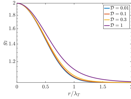
Figure 2.8: Behaviour of g_2(r) for an ideal gas above the condensation threshold: the value of the function is 2 in 0, and decays to 1 in a scale set by \lambda_T .
