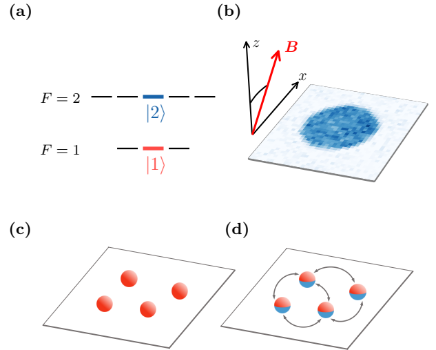
FIG. 1. (a) Level diagram of the hyperfine ground-level manifold showing the two states relevant to this work |1\rangle \equiv |F = 1, m = 0\rangle and |2\rangle \equiv |F = 2, m = 0\rangle . (b) Image of the atomic cloud obtained through absorption imaging along the direction perpendicular to the atomic plane. Atoms are confined in the xy plane in a disk of radius 12\mu\text{m} . The orientation of the magnetic field \mathbf{B} is tuned in the xz plane. (c) Schematics of atoms prepared in the state |1\rangle , with no MDDI in this case. MDDI are also absent when all atoms are in |2\rangle . (d) Significant MDDI occur for atoms in a linear superposition of |1\rangle and |2\rangle .
