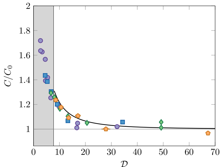
Figure 8.15: variation of C/C_0 with the phase-space density \mathcal{D} , the non-superfluid regime corresponding to the grey area. The different densities that were used are \bar{n} = 10.4, 21, 31.5 , and 42 \mu\text{m}^{-2} , and correspond respectively to violet disks, blue squares, green diamonds, and orange pentagons. The black line is a Bogoliubov prediction. Figure taken from [85].
