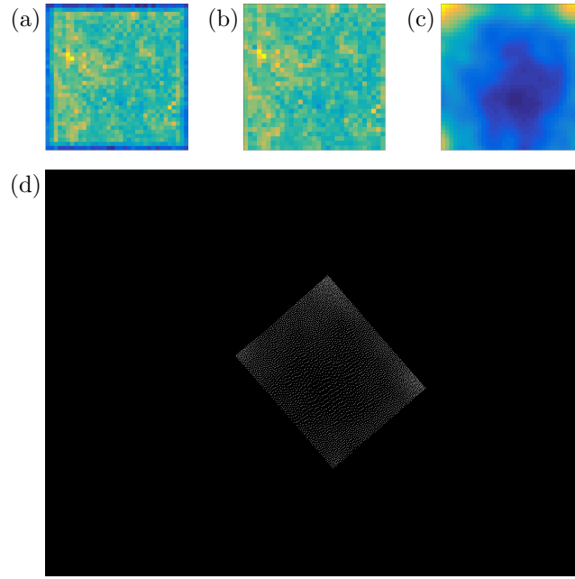
Figure 4.8: Example of a typical loop. The images shown are taken from the first iteration of the loop, and the target is a uniform density. With (a), we take an image \text{imTot}_n slightly bigger than the box. In (b), we take a subimage \text{imLoc}_n of (a) in order to avoid border effects. We then compute the output s_n shown in (c); note that in order to compensate for the gaussian shape of the beam, the gain is higher on the edges than in center, resulting in an output also higher on the edges. Finally, we resize everything and create a grey-level image (d) that we load on the DMD. We can then reiterate.
