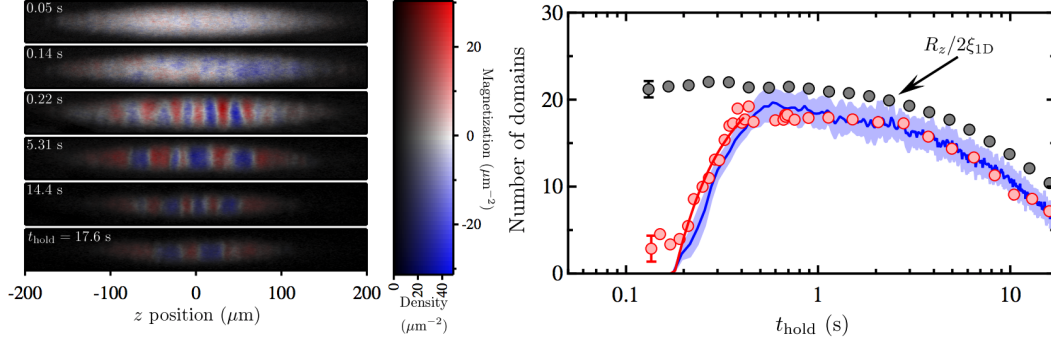
Figure 5.6: Left: a quasi 1D BEC of ^{87}\text{Rb} is initially prepared in an equal superposition of the 2 immiscible spin states |F=1, m_F=\pm 1\rangle . The number of spin domains quickly increases, before slowly decreasing (see right): because of atomic losses, eventually, small domains cannot maintain a total polarisation and they coalesce into bigger domains. Right: number of domains with time. The red points are the experimentally observed values (typical uncertainty plotted on the leftmost point), the red line is an exponential fit, the blue line is a Gross-Pitaevskii simulation (with uncertainties denoted by the blue band), and the grey points correspond to the ratio R_z/2\xi where R_z is the Thomas-Fermi radius of the gas, and \xi the healing length. Considering that the system is of total size 2R_z and that the domains have a typical size of 4\xi , this ratio gives an estimate of the number of domains present in the system. Both figures are taken from [58].
