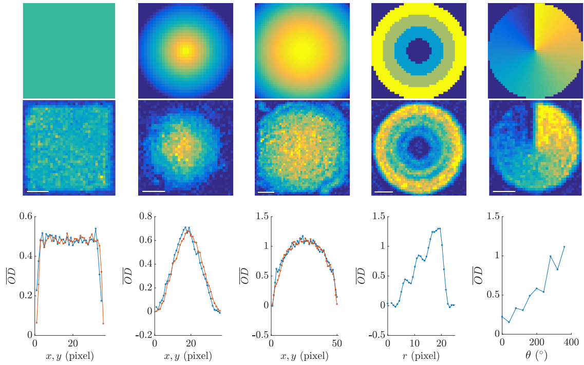
Figure 4.9: Examples of images realised thanks to the correction algorithm. All these images are averaged over typically 7 iterations. The white line represents 10\ \mu\text{m} . From top to bottom: target image, loop corrected image, and mean OD along the two directions for corrected image (radial and azimuthal average for the Hanoi towers and phase winding pattern respectively).
