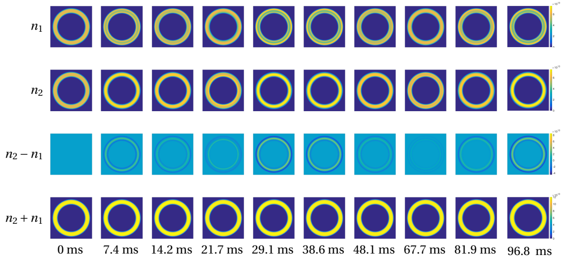
Figure 6.15: Simulation of demixing in SSBC with no seed for n_{\text{tot}} = 30 \mu\text{m}^{-2} . Only radial dynamics with small amplitudes take place up to 100 ms.
