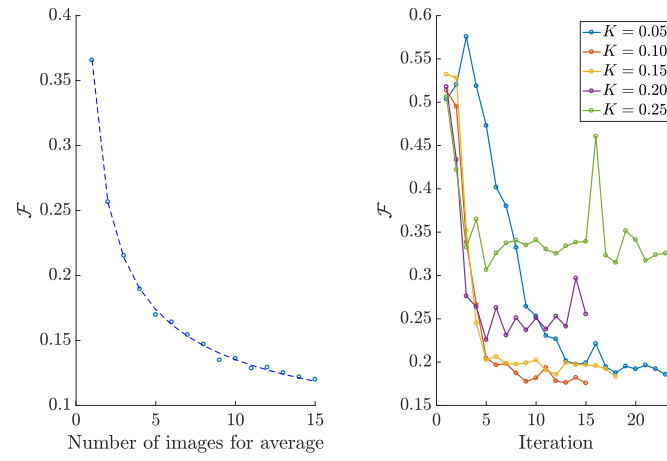
Figure 4.13: Left: decrease of \mathcal{F} with the number N_r of images taken. The dashed line is a square-root fit. Right: figures of mérite corresponding to gains K = 0.05 - 0.25 .
