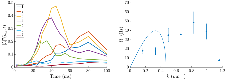
Figure 8.4: Left: evolution of each mode's population |\hat{n}|^2(k_m, t) for n_{\text{tot}} = 67 \mu\text{m}^{-2} , and L = 40 \mu\text{m} . As can be seen in Fig. 8.1, each mode grows before collapsing. Modes with a higher k collapse before modes with lower ones, causing a cascade of k on experimental images. Right: we can try to fit these modes's growths with exponentials; however, in this case, the obtained \Omega(k) is very different from what is expected in an infinite system (blue line). This naive picture is no longer applicable, and in order to better understand the system's important features, we decide to focus on a simpler observable: we look at the pattern's average mode number instead of performing this individual mode analysis.
