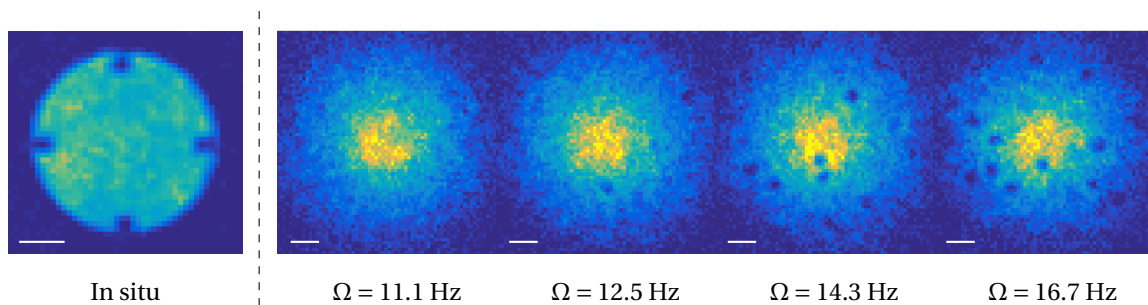
Figure 8.16: Left: stirring created by DMD2 (in situ image). The four teeth rotate at certain frequency in order to inject angular momentum in the cloud. Right: after 10 turns, we image the vortices with a time of flight measurement. The number of vortices grows as we increase the injected angular momentum. The white lines represent 10 \mu\text{m} .
