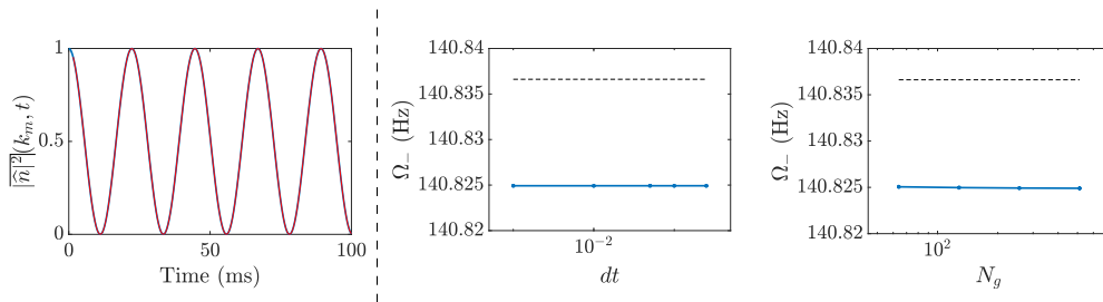
Figure 6.6: Left: Evolution of |\hat{n}|^2(k_m, t) for m = 4 , dt = 0.05 , N_g = 256 , and \delta A = 10^{-3} (the red line is a cosine fit). The function looks very monochromatic, and the same thing goes for all the other dt and N_g that were explored. Middle: From the fit, we extract a pulsation \Omega that we plot versus dt . The same thing is done for N_g on the right graph. The dashed black lines are the prediction from [61]. Note the values on the y -scale.
