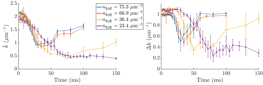
Figure 8.5: Evolution of the mean wave vector \bar{k} present in the system (left), and its standard deviation \Delta k (right) with time, for boxes of sides L = 40 \mu\text{m} and various densities. Each value is averaged over typically 10 iterations; the error bars are the resulting standard deviations over these \simeq 10 iterations.
