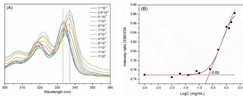
Fig. 5.6 Fluorescence excitation spectra (A) and I336/I334 vs. LogC plots (B) of HPMC7K-JEF M2K diblock copolymer solutions at different concentrations
