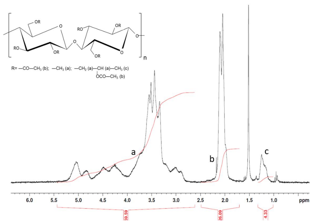
Fig. 2. 1 NMR spectrum in CDCl_3 of acetylated K4M. Signal (a) is assigned to protons on the glucose ring, the methyl substituents and the proton on isopropyl substituents, signal (b) to protons on the acetyl groups and signal (c) to methyl protons on isopropyl substituents.
