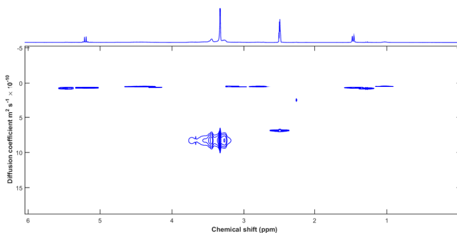
Fig. 3. 4 DOSY- NMR spectrum of HPMC-PLA 10 in DMSO- d 6
