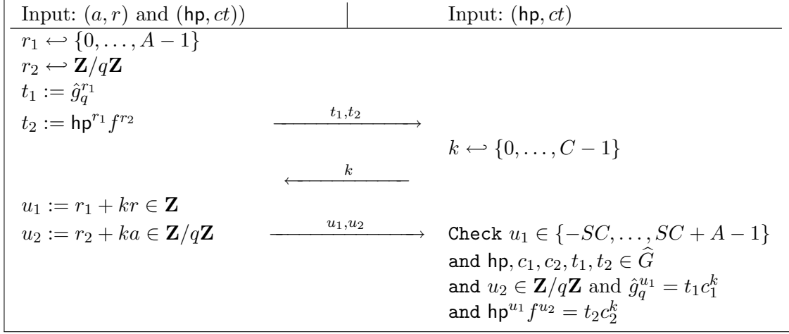
Figure 3.9: ZKAoK for \mathcal{R}_{\text{Enc}} .
