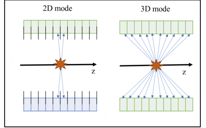
Figure 4: 2D and 3D acquisition modes
