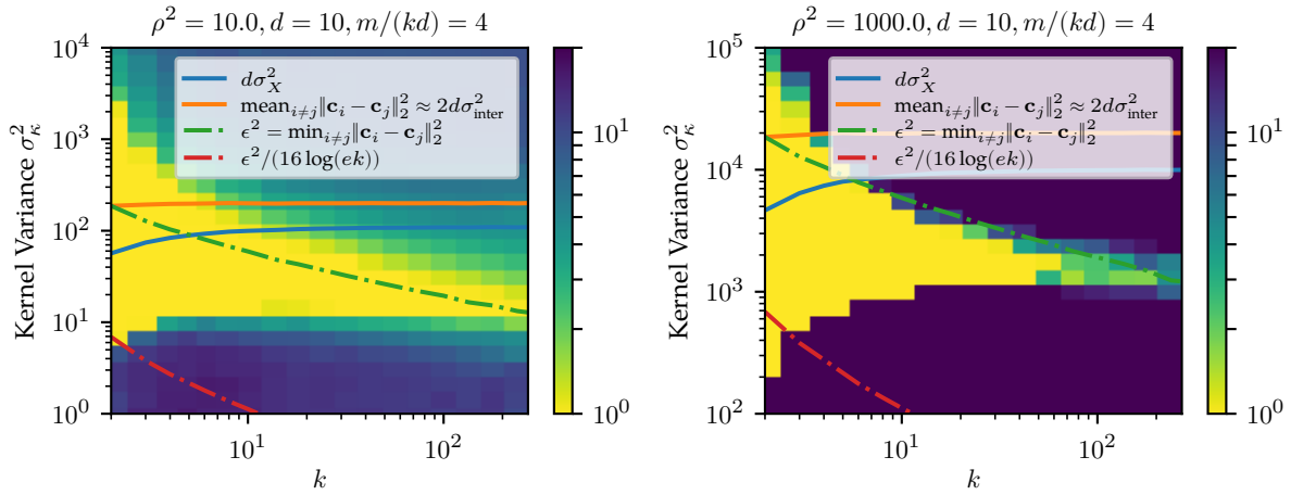
Figure 4.8: RSE as a function of both k and \sigma_x^2 . Here \sigma_{\text{intra}}^2 = 1.0 , and errors are clipped to the interval [1, 20] for coherence with other figures.
