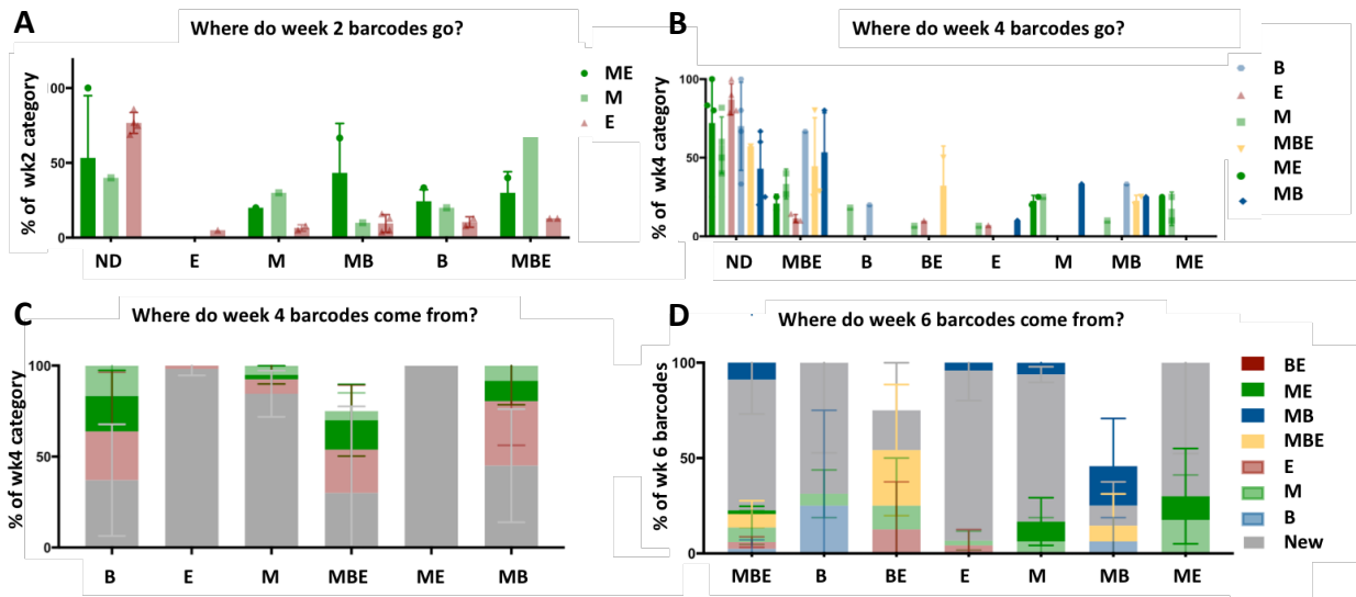
Figure S6: Changes in lineage restriction of individual HSC over time. (A-D) HSC were sorted from CD45.1 mice, barcoded using the LG2.2 cellular barcoding library, and transplanted into sublethal-irradiated wt mice. Analysis of barcodes in the E, M, and B lineage from blood at week 2, 4, and spleen 6 in the same individual mice. (A-D) Bar-graph showing the fate (A, B) and origin (C, D) of barcodes detected with the indicated lineage restriction at the indicated timepoint. Fate and origin are defined based on the detection and lineage restriction at the respectively previous (origin) and next (fate) analysis timepoint. Shown are values from the same animals throughout (n=4 from one experiment). For all bar graphs mean and S.D. between mice are depicted.
